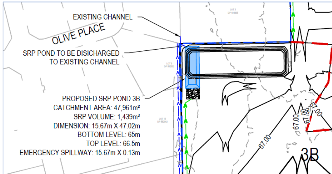
Figure 9: Erosion and Sediment Control for SW Basin C
