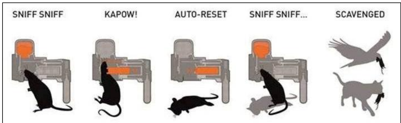
Figure 21: Operation process diagram of Goodnature A24 rodent and mustelid trap.
