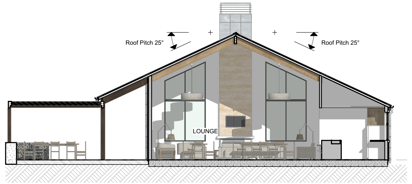
Section 4 1:100
