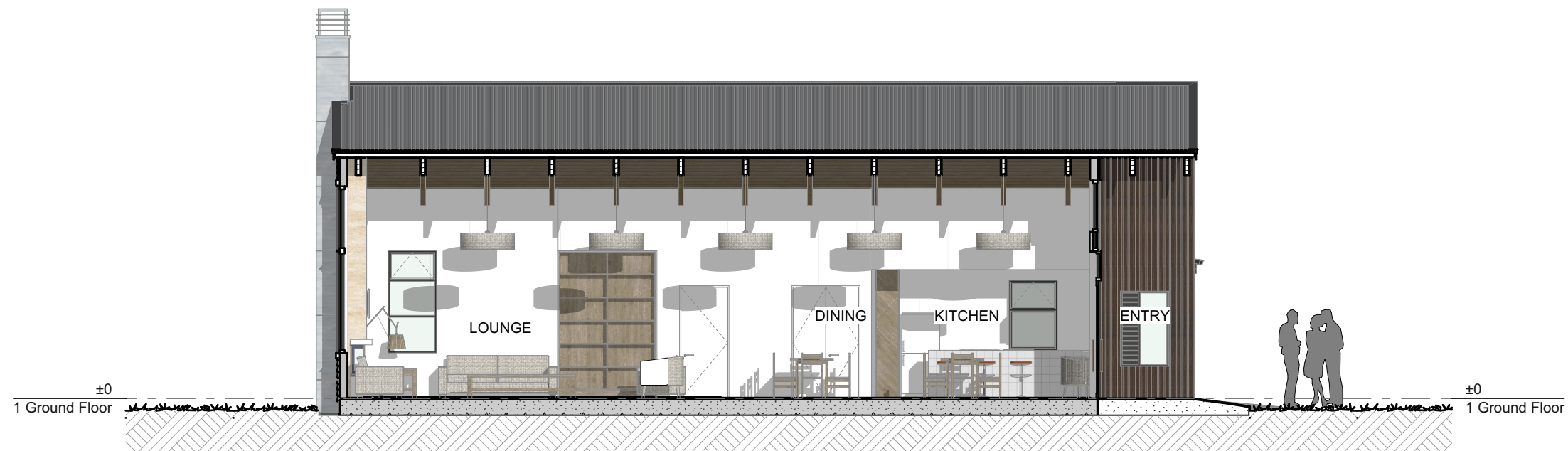
Section 3 1:100
