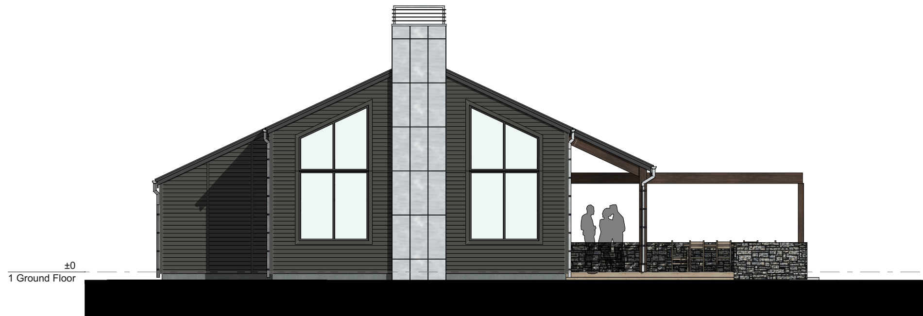
South Elevation 1:100
