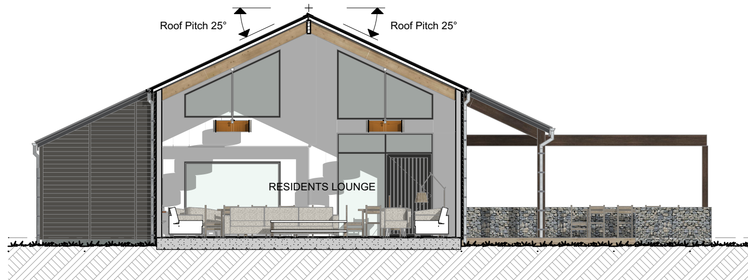
Section 2 1:100
