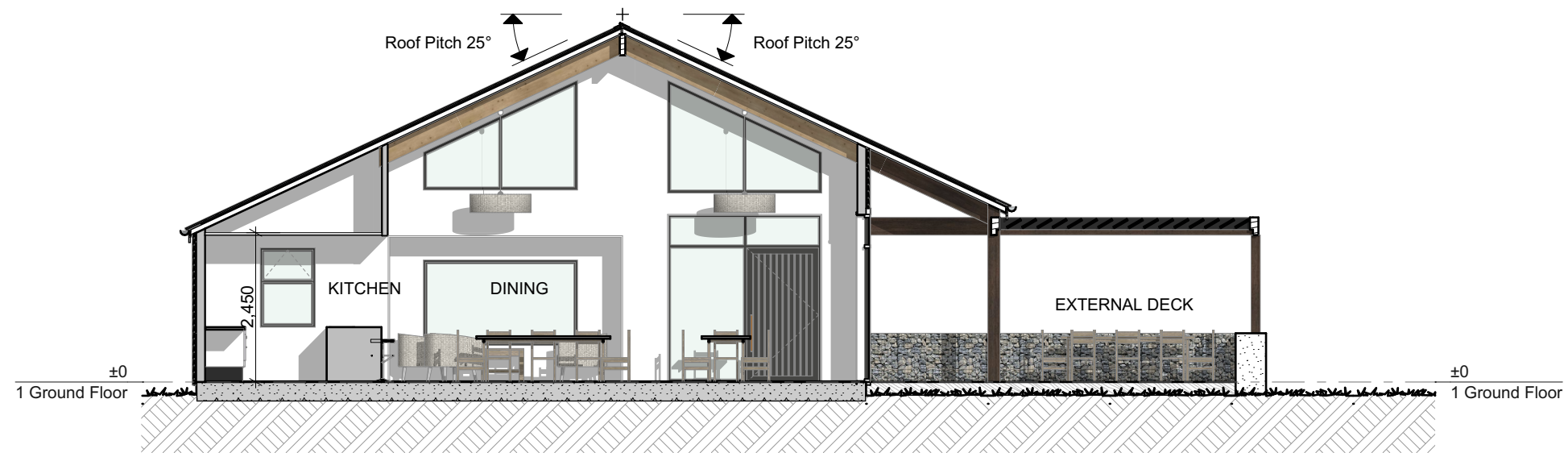
Section 1 1:100
