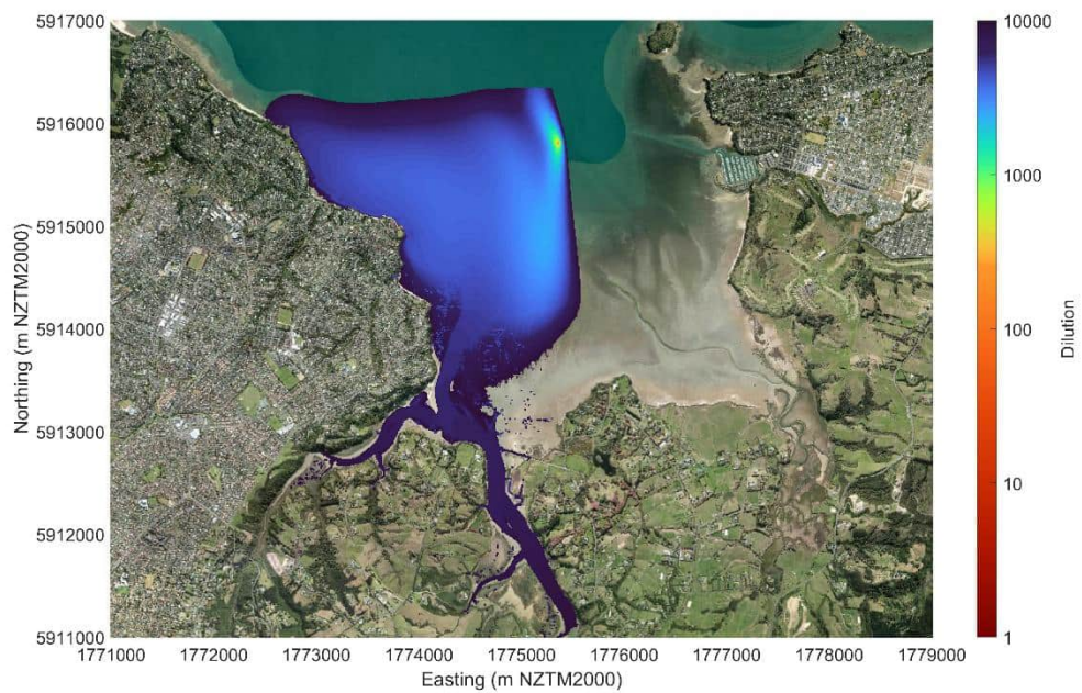
Figure Appendix C.2: Horizontal dispersion coefficient of 0.5 \text{ m}^2/\text{s} .
