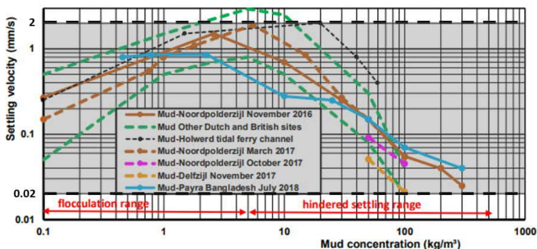
Figure 3-8 Flocculation and hindered settling
