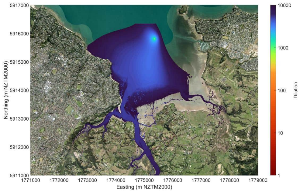
Figure Appendix C.4: Horizontal dispersion coefficient of 5 \text{ m}^2/\text{s} .
