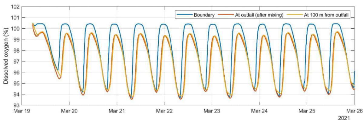
Figure 6.9: Dissolved oxygen saturation ( DO_{sat} ) at the boundary, at the outfall (after mixing) and 100 m from the outfall.
