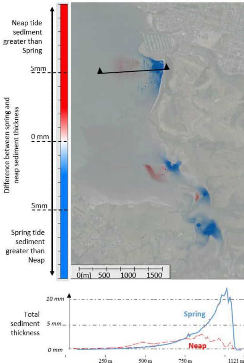
Figure 4-3 Neap vs spring sediment thickness map comparison
