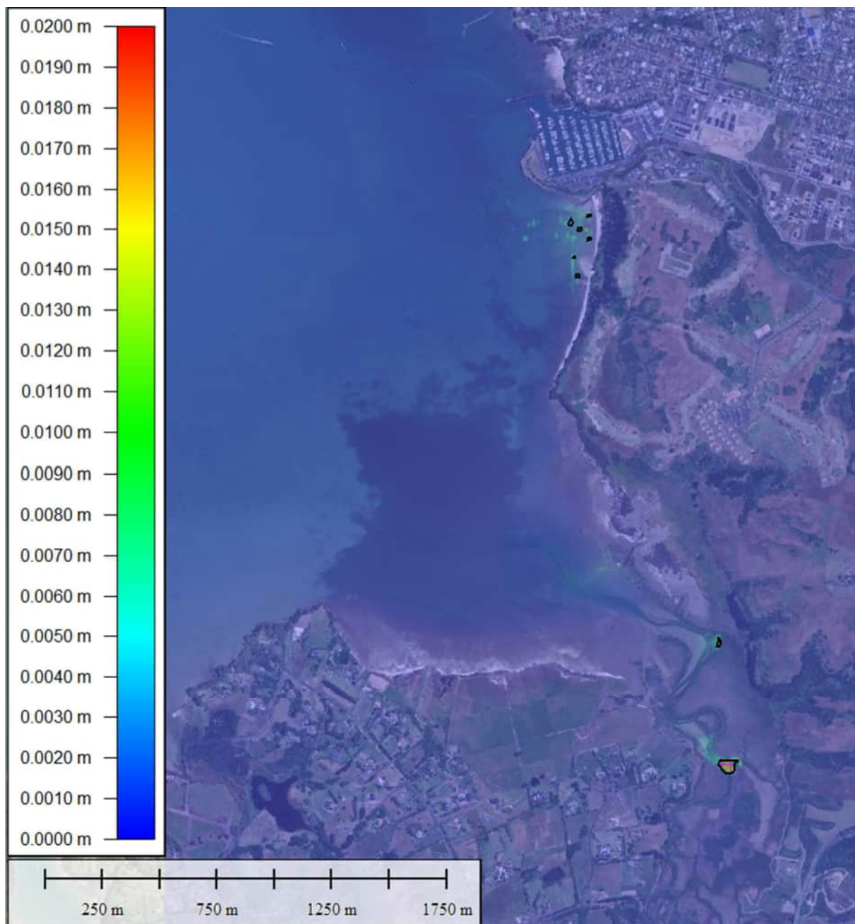
Figure 10-25 10 ARI TSS assuming Neap tide, HT peak discharge
