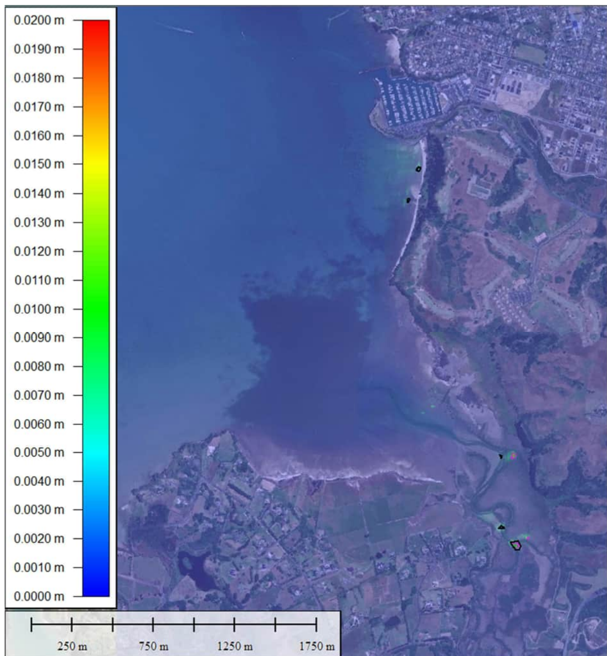
Figure 10-23 10 ARI TSS assuming Spring tide, FT peak discharge
