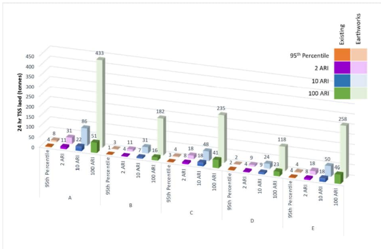
Figure 2-22 24 h TSS loads from each stream outlet for existing baseline and earthworks stages for 95 th percentile, 2-y ARI, 10-y ARI and 100-y ARI events.
