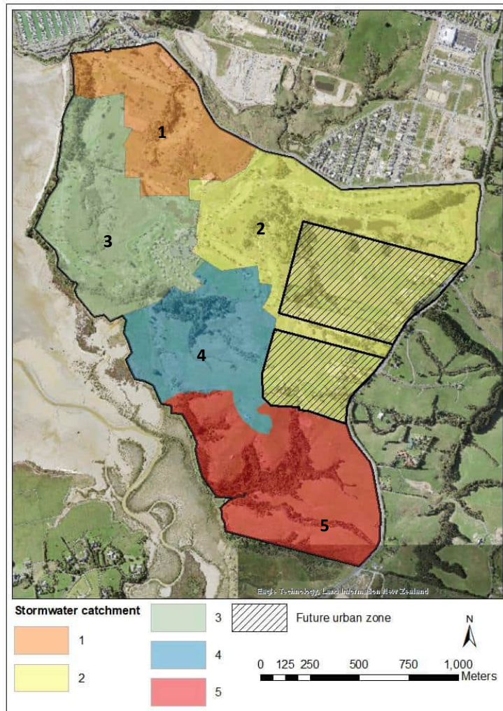
Figure 3-1: Stormwater catchments for the plan change area under the fully-developed scenario.
