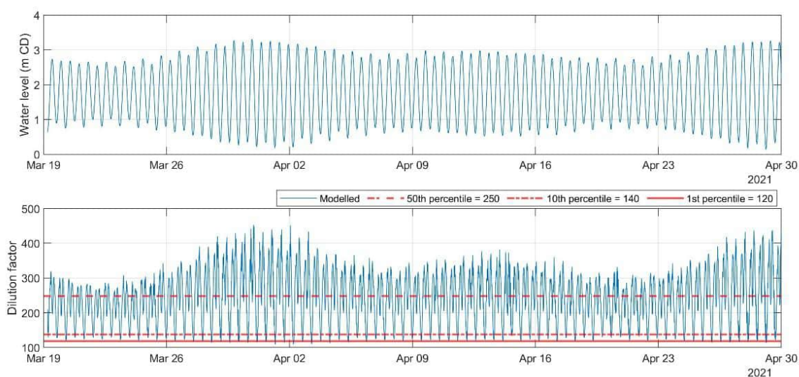
Figure 6.5: (upper) Water level at the discharge location and (lower) depth-averaged dilution at the discharge location.
