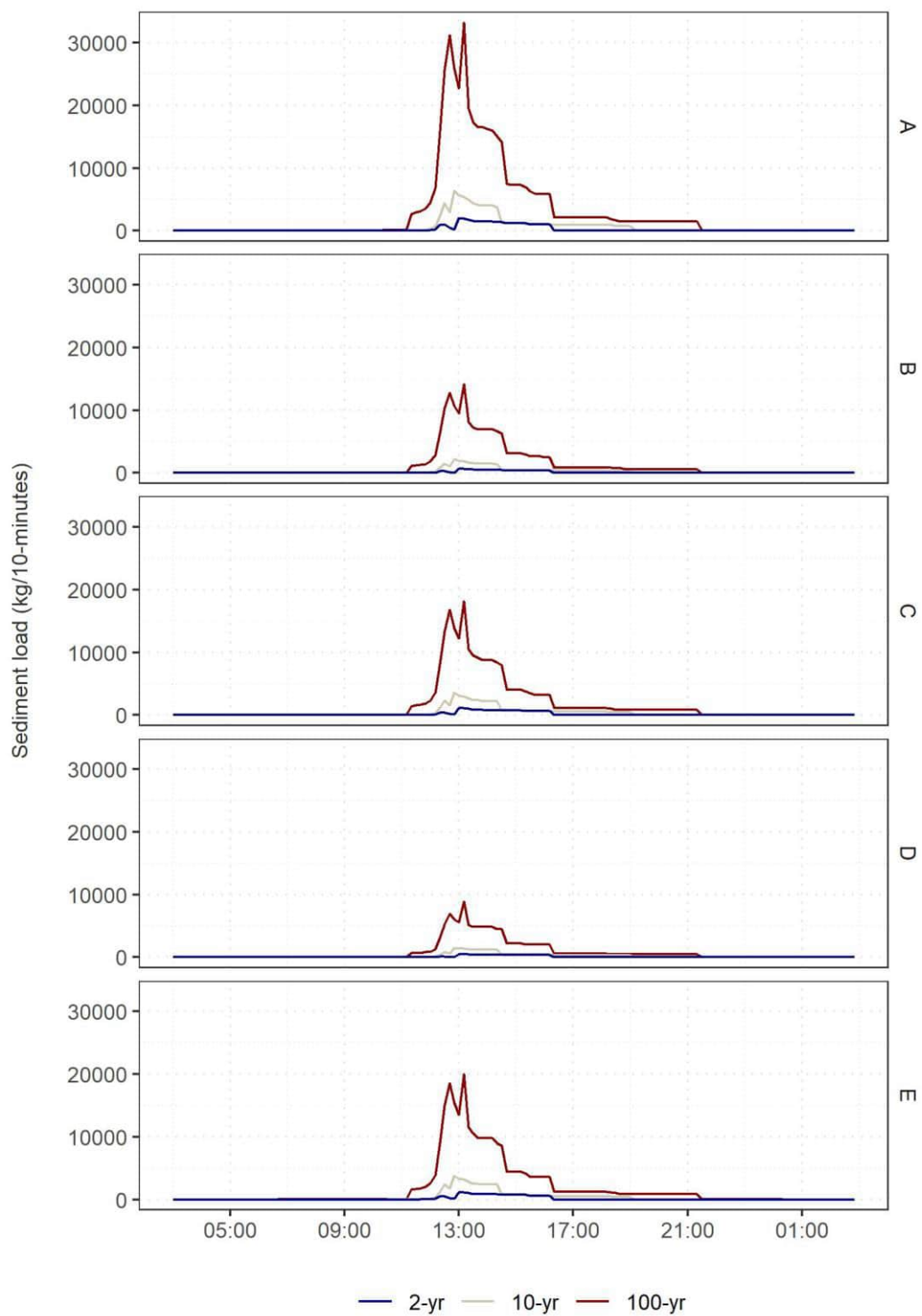
Figure C-2: Time series of disaggregated 24-hr ARI sediment loads by outlet.
