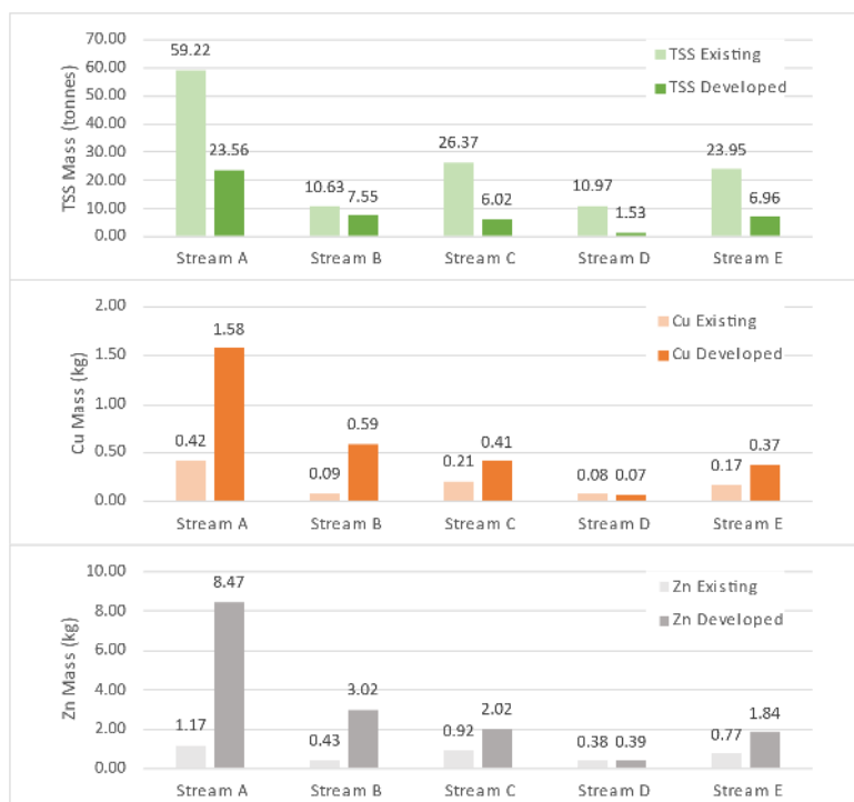
Figure 2-23 Comparison of existing and developed annual mean loads of TSS, Cu and Zn
