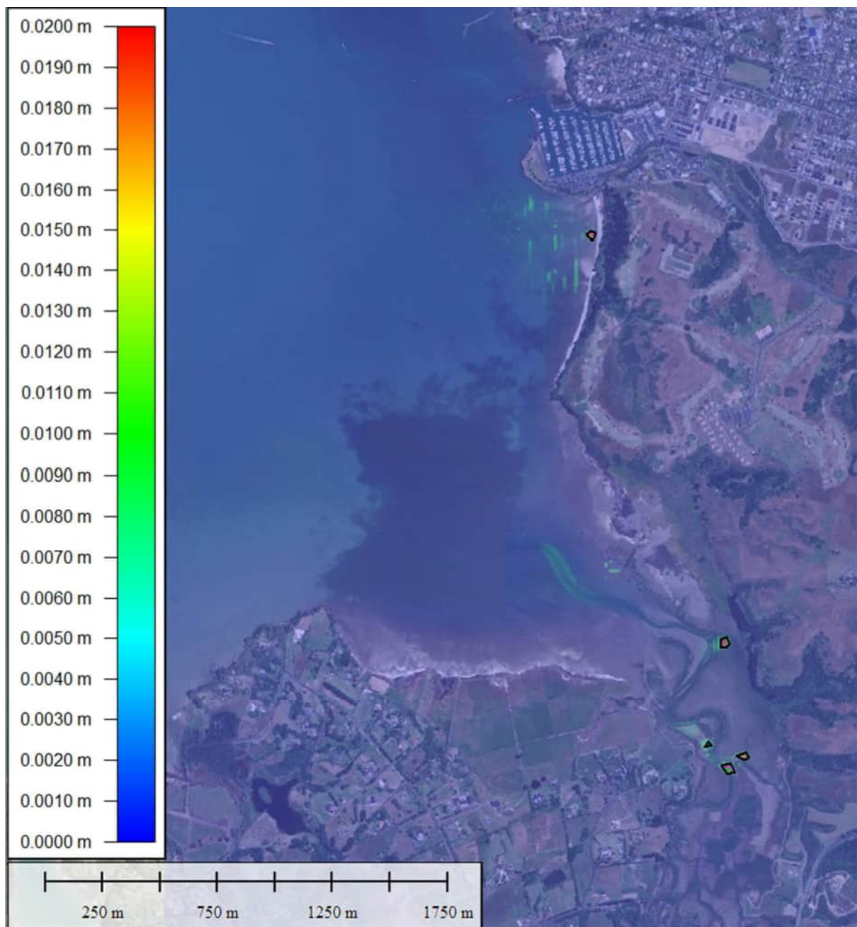
Figure 10-24 10 ARI TSS assuming Spring tide, ET peak discharge
