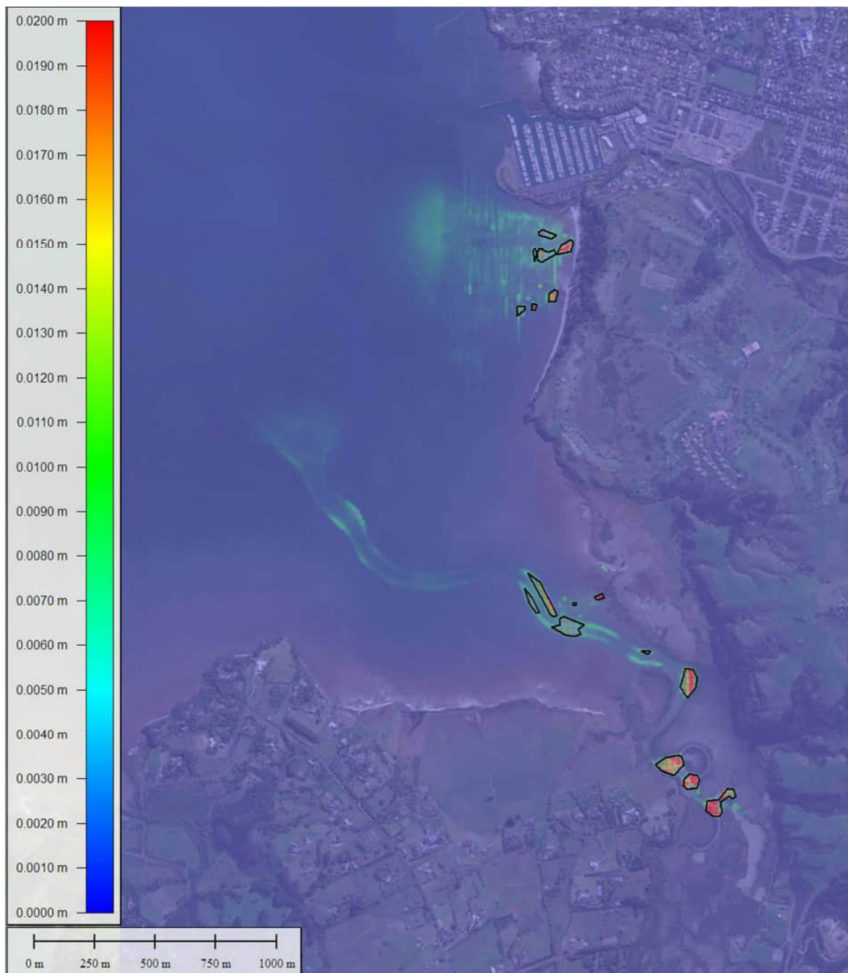
Figure 10-18 100 ARI TSS assuming Neap tide, LT peak discharge
