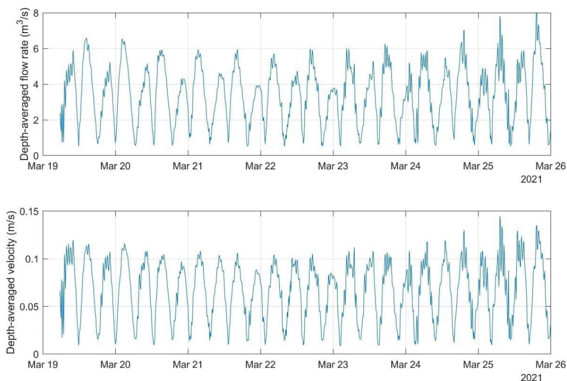
Figure 4.1: Depth-averaged flowrate and velocity at the discharge location using the baseline hydrodynamic model. The minimum flowrate is 0.53 m 3 /s, which is much higher than the discharge flowrate of 0.046 m 3 /s.
