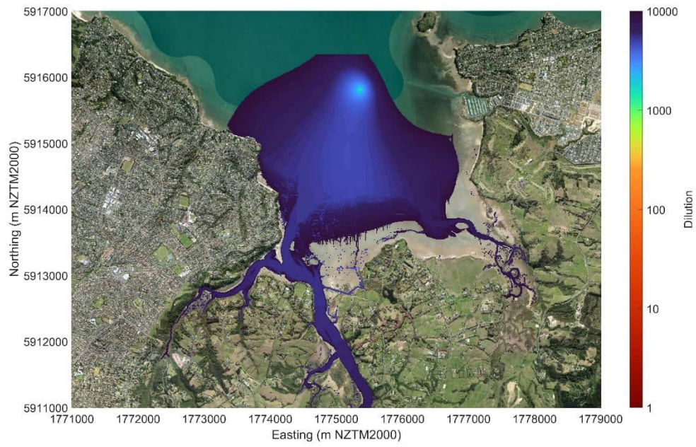
Figure Appendix C.5: Horizontal dispersion coefficient of 10 m 2 /s.
