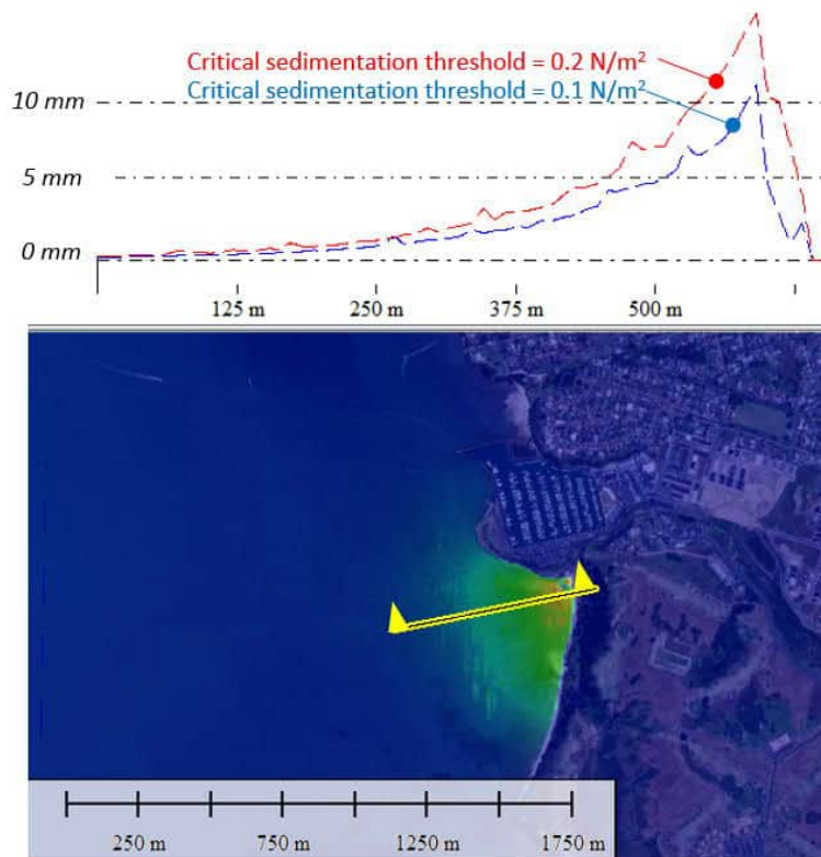
Figure 3-11 Sensitivity of modelled deposition thickness to critical bed shear stress for sedimentation
