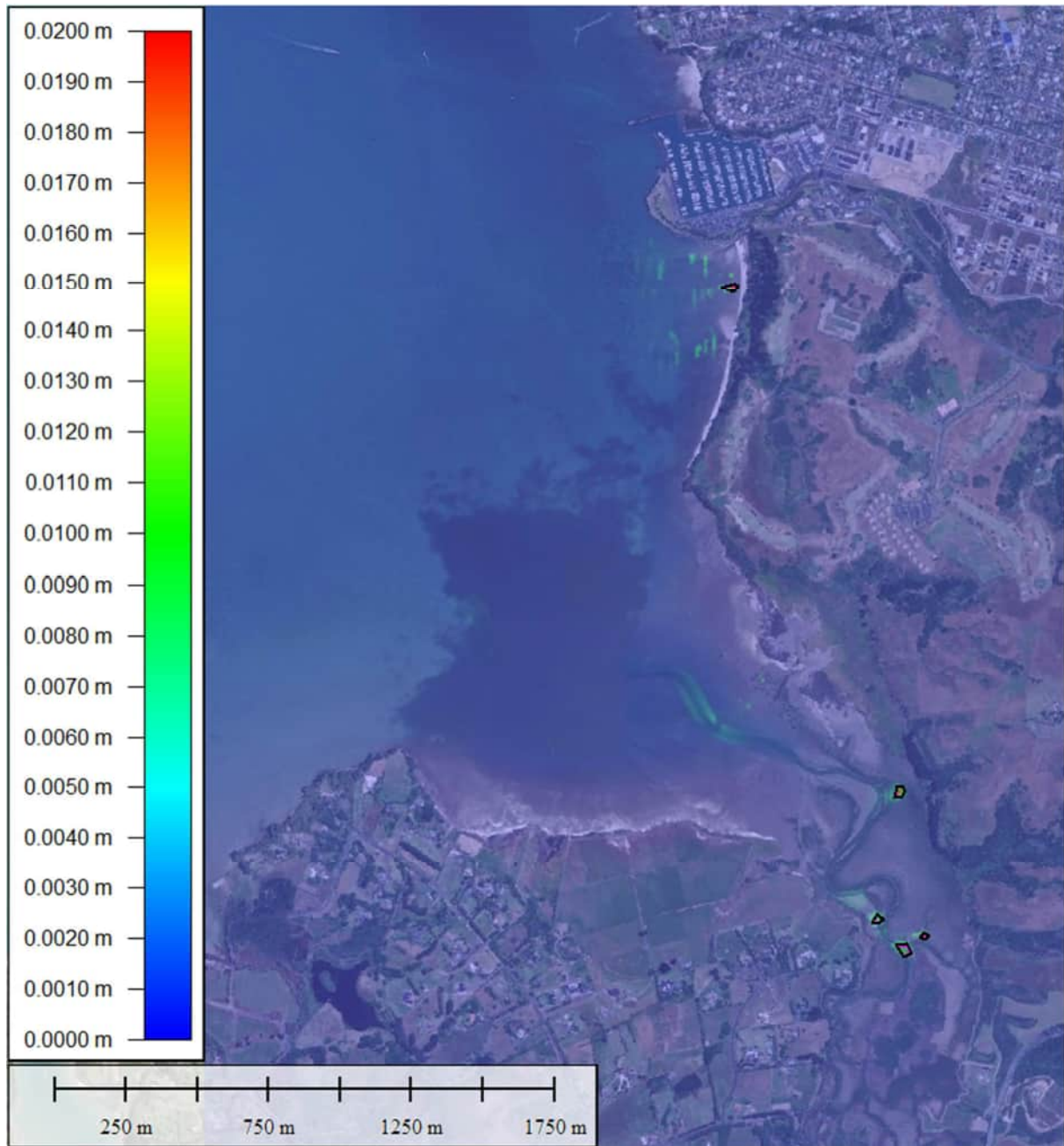
Figure 10-22 10 ARI TSS assuming Spring tide, LT peak discharge
