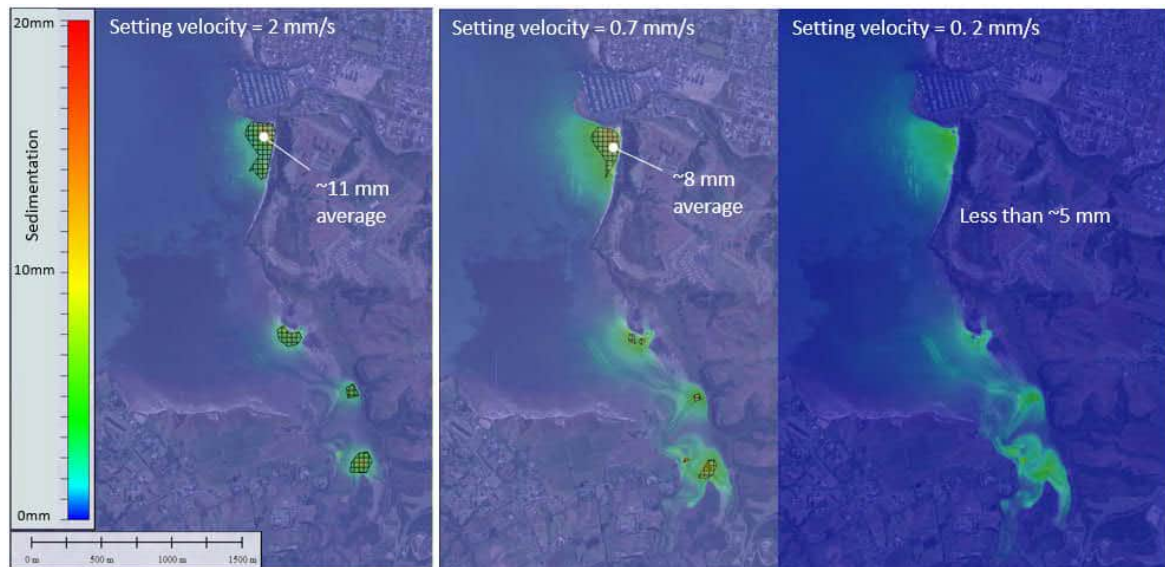
Figure 3-9 Sensitivity of settling velocity parameters based on high spring tide condition
