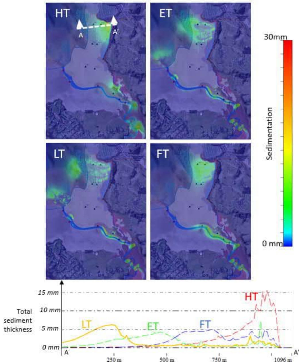
Figure 4-2 Discharge simulations for different tidal stages
