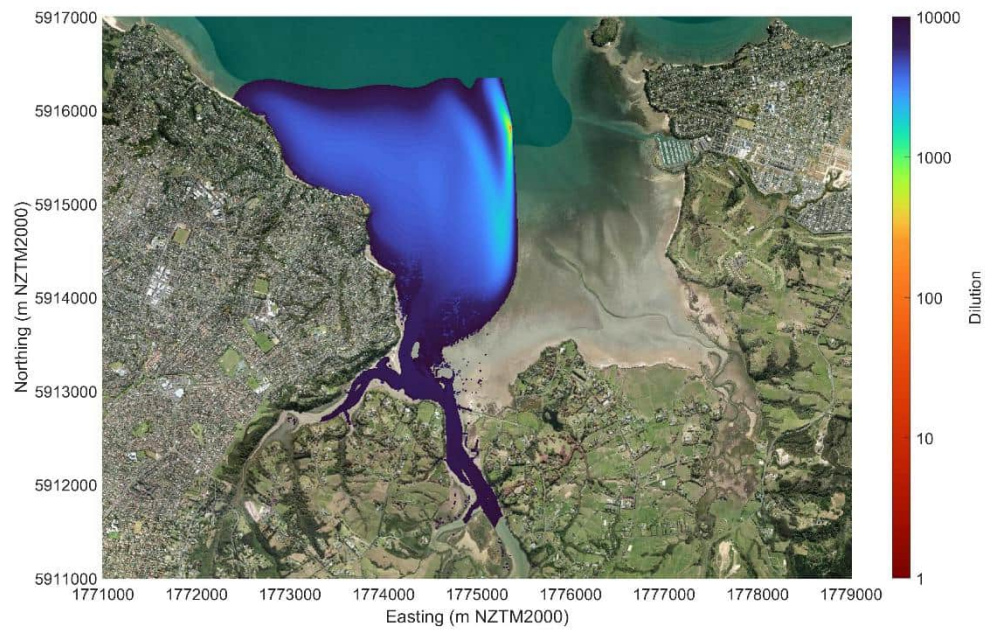
Figure Appendix C.1: Horizontal dispersion coefficient of 0.05 \text{ m}^2/\text{s} .
