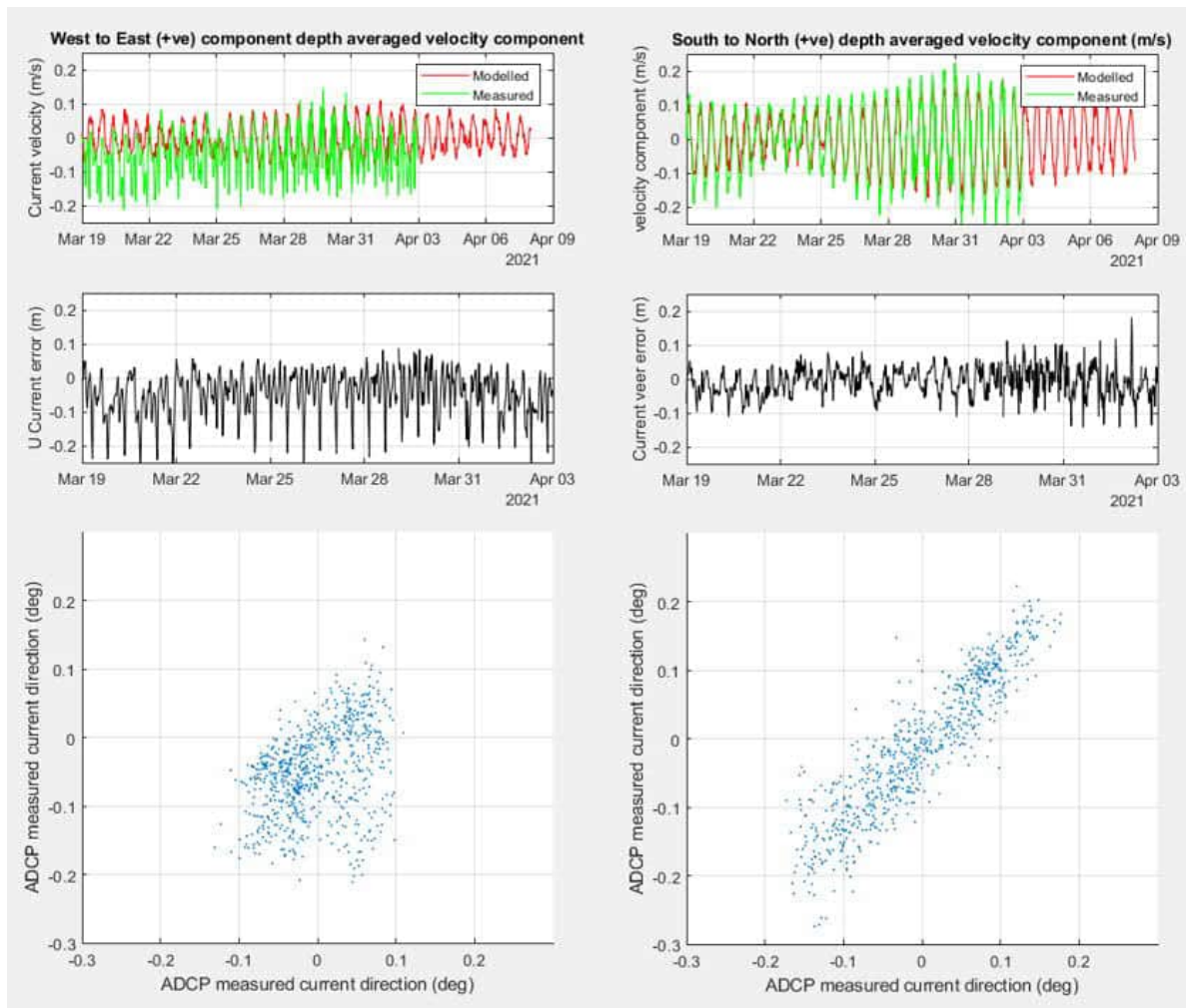
Figure 10-12 Review of currents in cartesian (+ve flowing to north and east directions)
