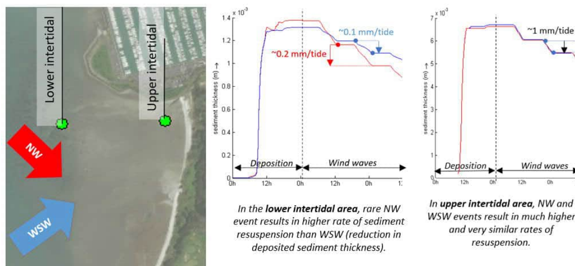
Figure 4-6 Sediment resuspension from wind waves applied over consecutive tidal cycles
