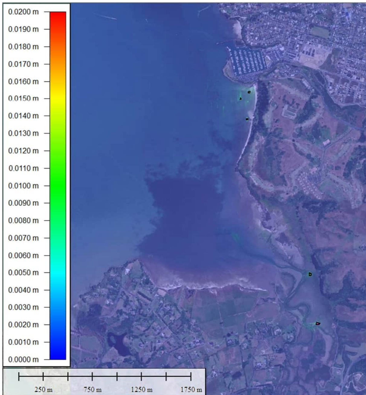
Figure 10-21 10 ARI TSS assuming Spring tide, HT peak discharge
