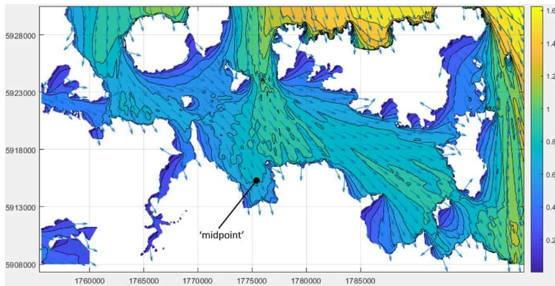
Figure 3-7 Extended model domain
