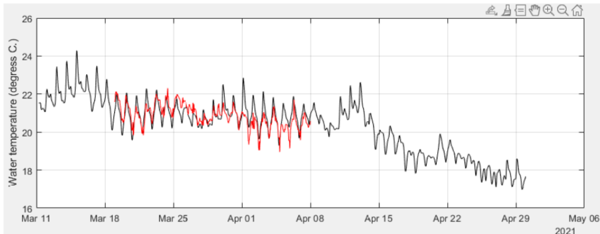
Figure 3-6 Comparison between measured temperatures in the location of the ADCP and modelled boundary values (red line indicates measured values, black line shows adopted boundary values)
