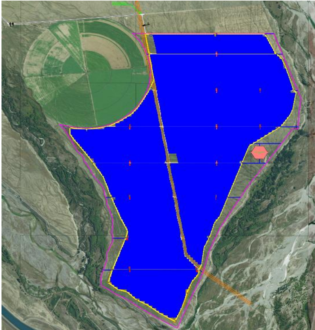
Figure 2.2: Proposed The Point Solar Farm
