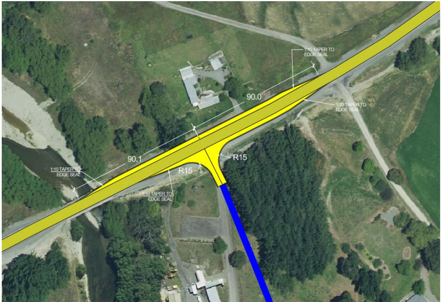
Figure 3.4: Site Entrance Design Summary plan as per NZTA Planning Policy Manual (Diagram E)
