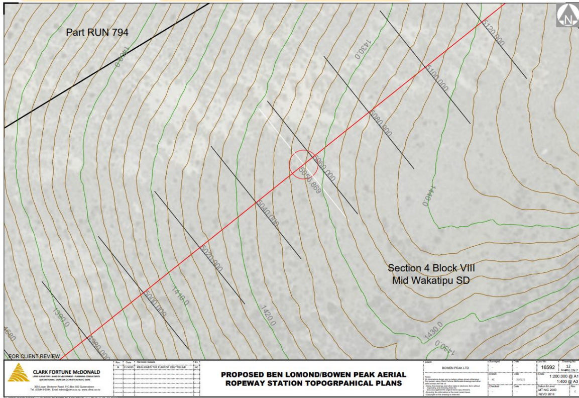
Figure 10: Pylon 7 Topo Plan
