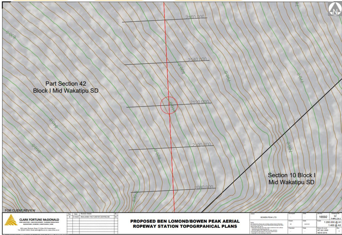
Figure 7: Pylon 4 Topo Plan
