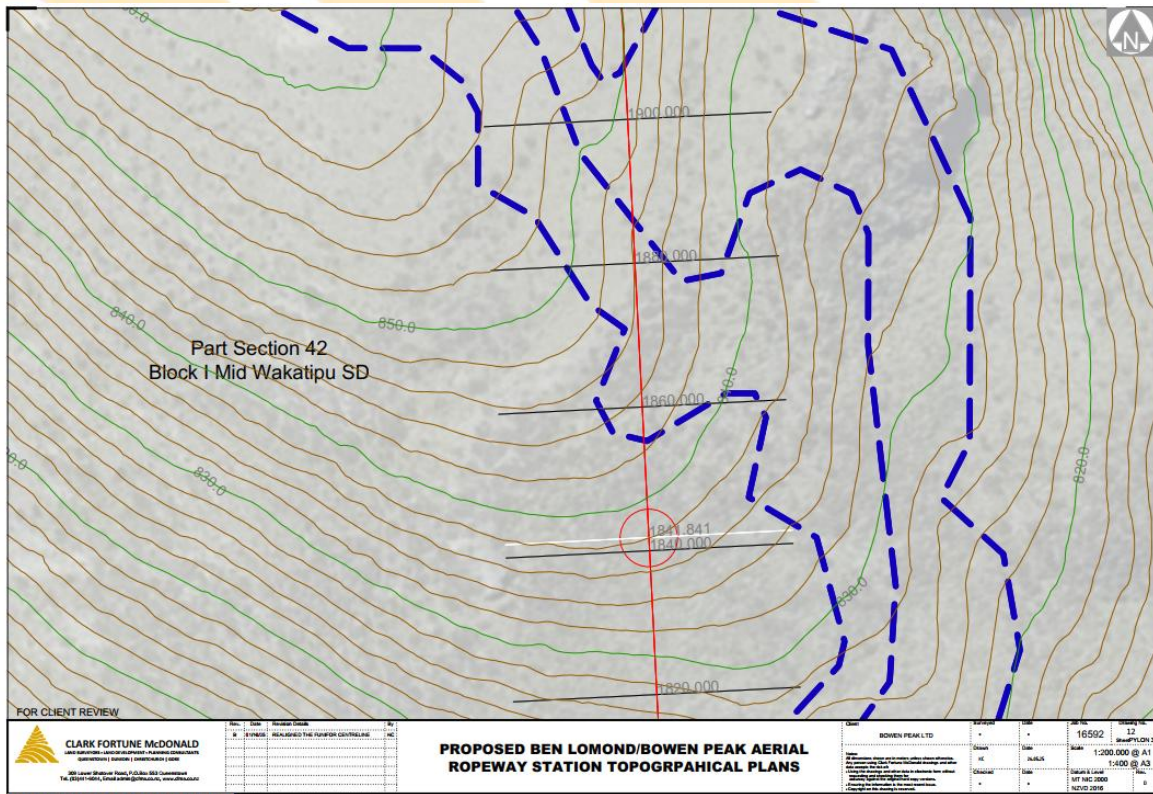
Figure 6: Pylon 3 Topo Plan
