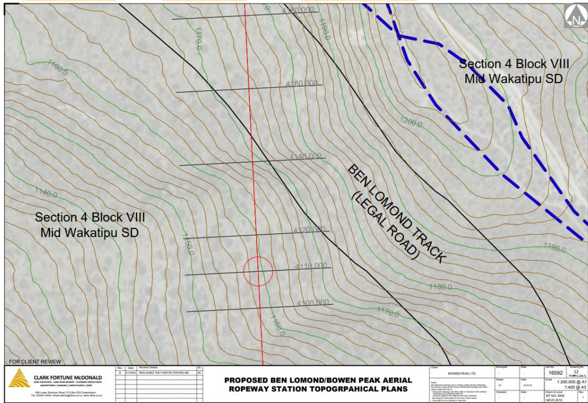
Figure 8: Pylon 5 Topo Plan
