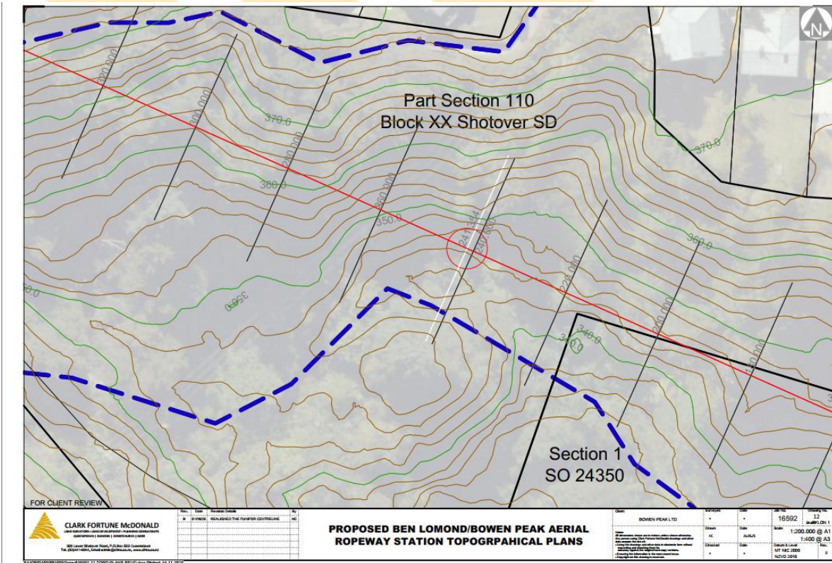
Figure 3: Pylon 1 Topo Plan
