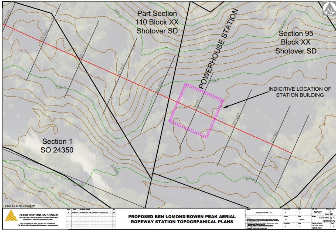
Figure 2: Powerhouse Station Topo Plan
