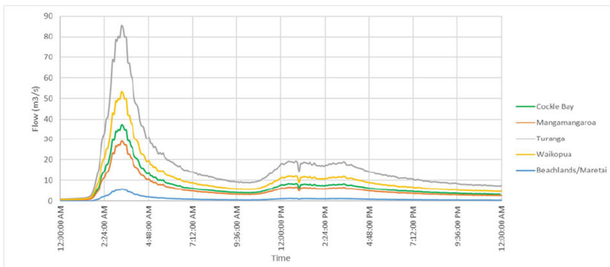
Figure 5.2: Flow hydrographs for wider catchments for the April 2017 event
