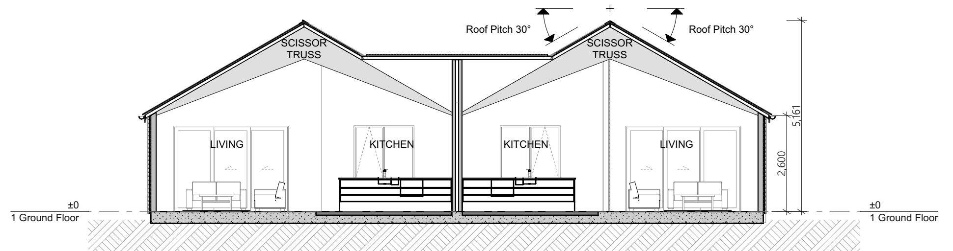
Section 2 1:100
