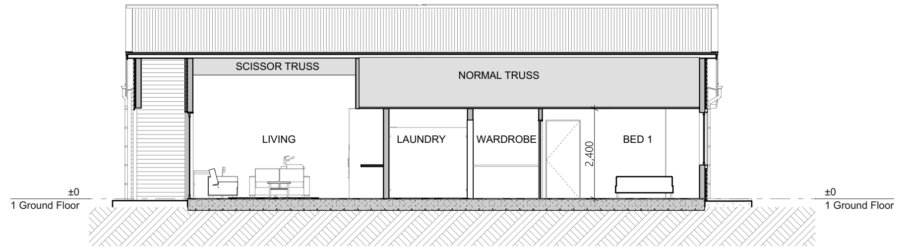
Section 1 1:100
