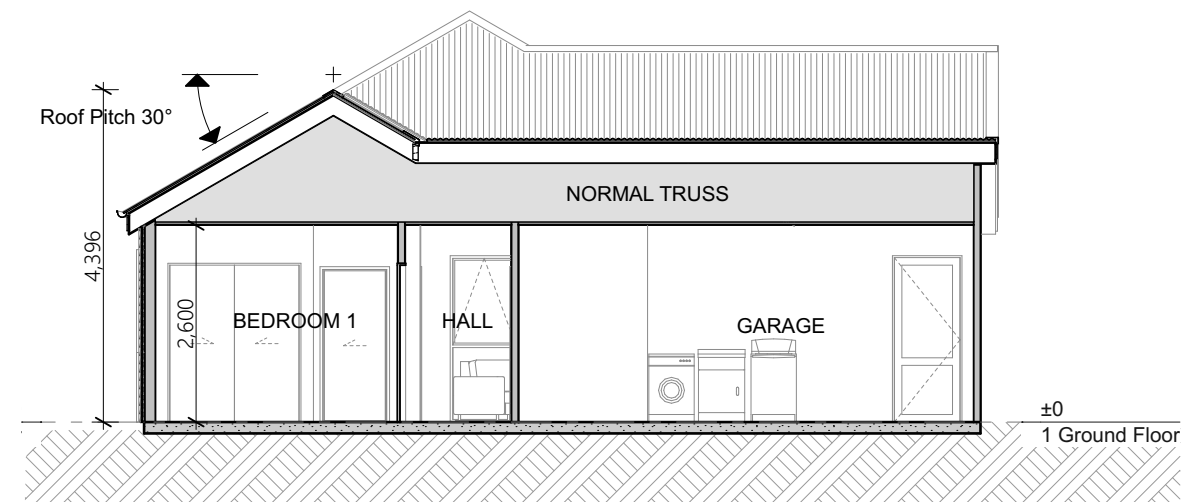
Section 2 1:100
