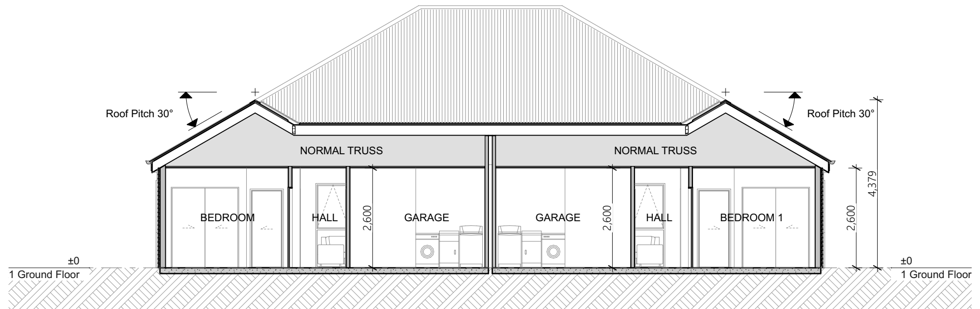
Section 2 1:100
