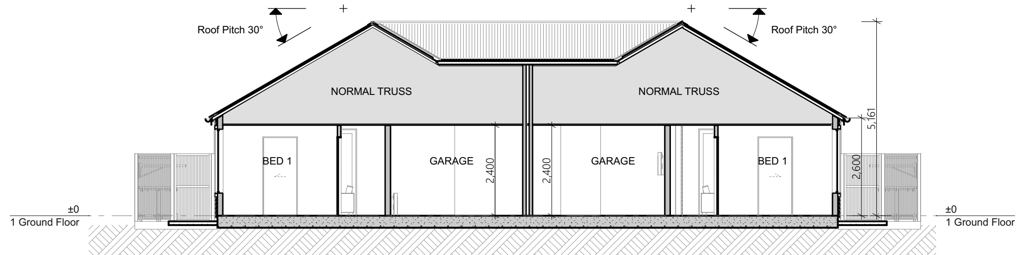
Section 2 1:100
