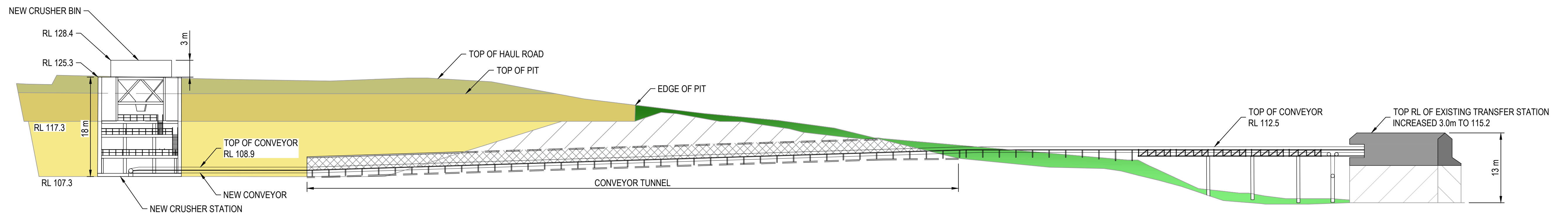
A SECTION 1:400
