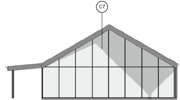
COMMUNITY FACILITY - ELEVATION 4 SCALE @ A3 - 1 : 200
