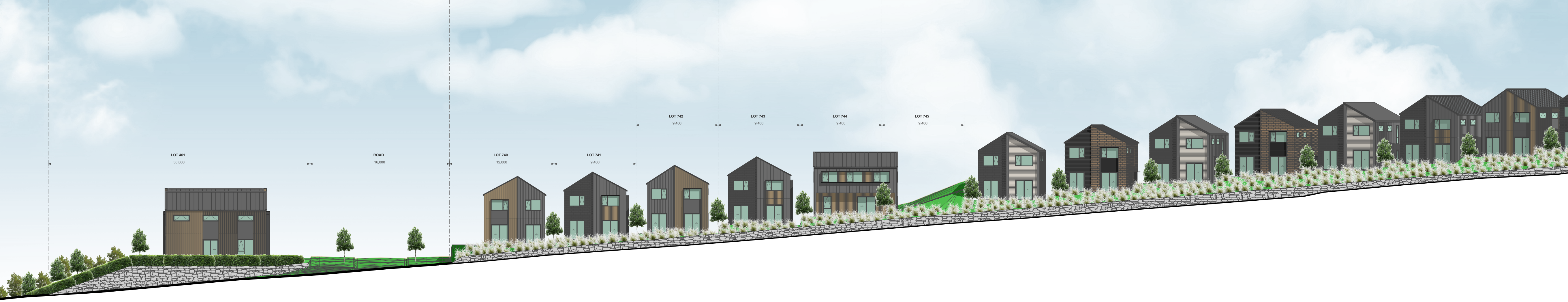
ELEVATION - STAGE 2A-1 - LOTS 740-756
