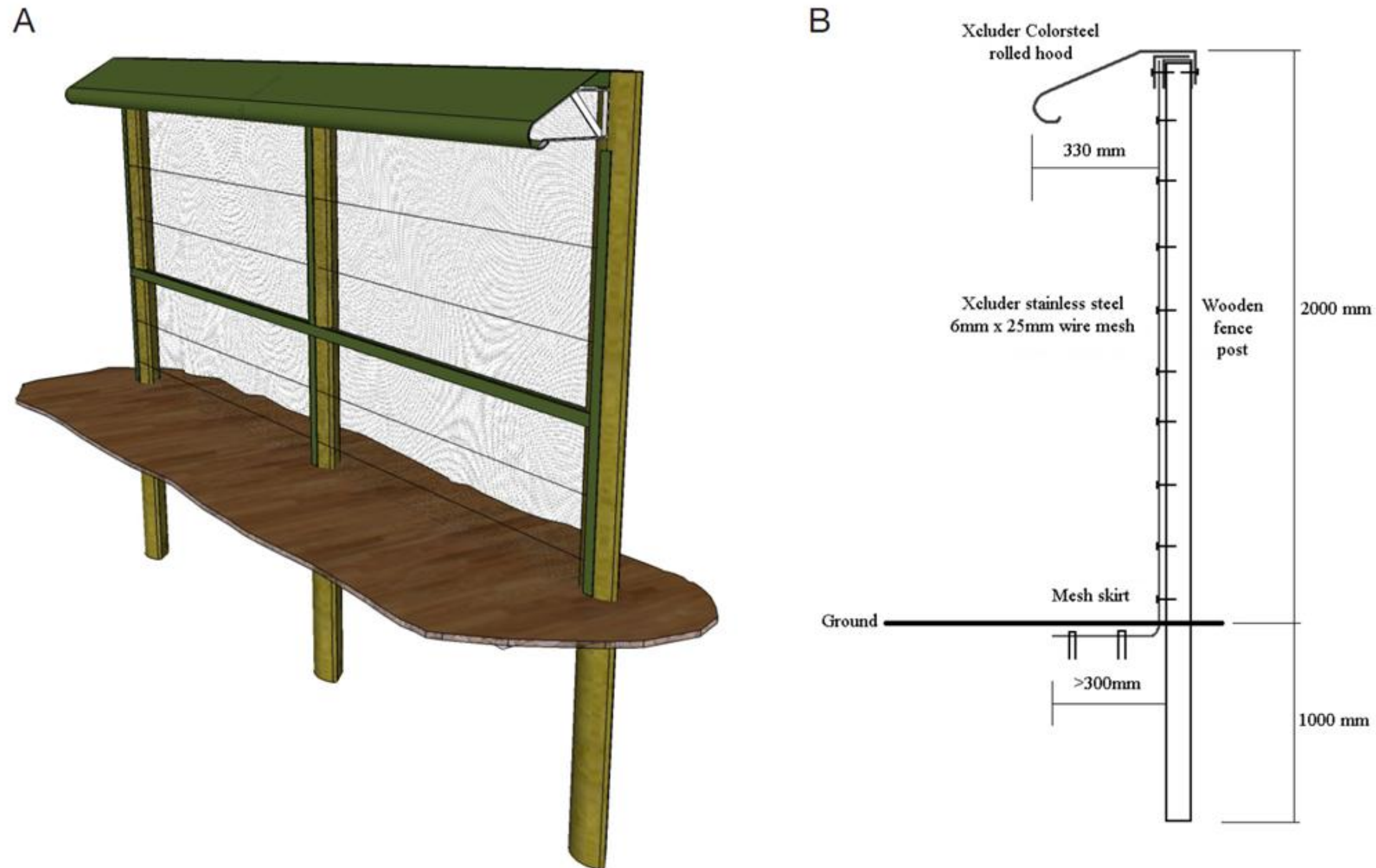
Figure 14. Example diagram of predator exclusion fence (A) and cross section of Xcluder® predator exclusion fence (B) (Bell, 2014).
