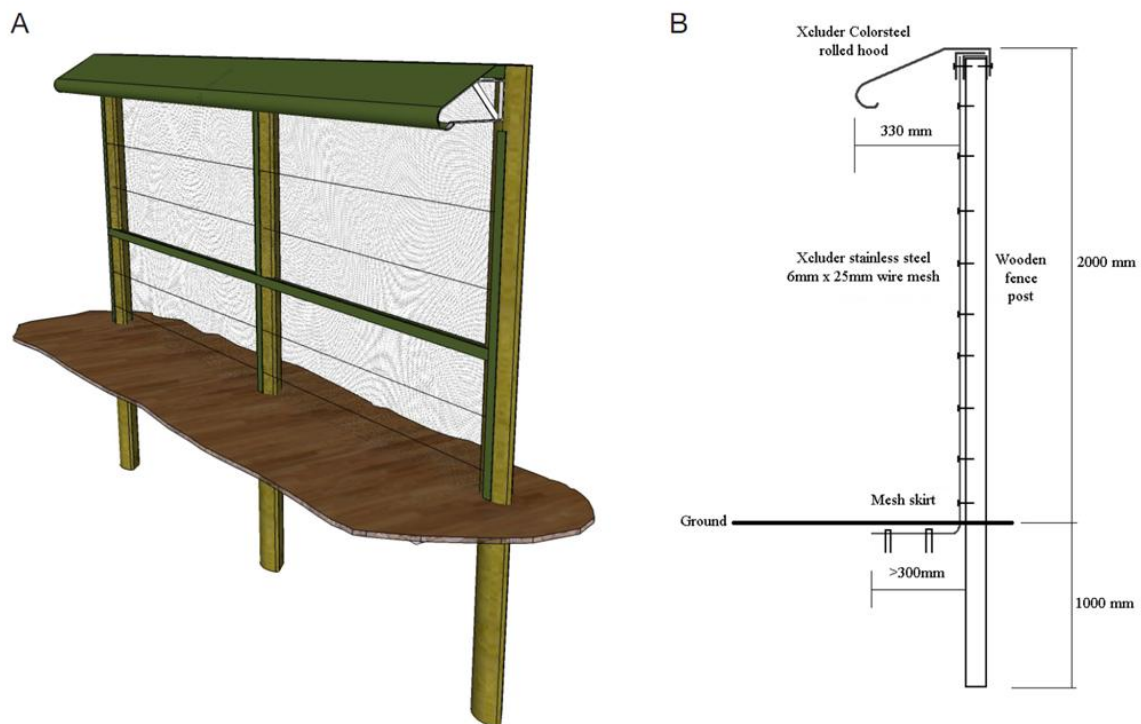
Figure 1: Example diagram of predator exclusion fence (A) and cross section of Xcluder® predator exclusion fence (B) (Bell, 2014).
