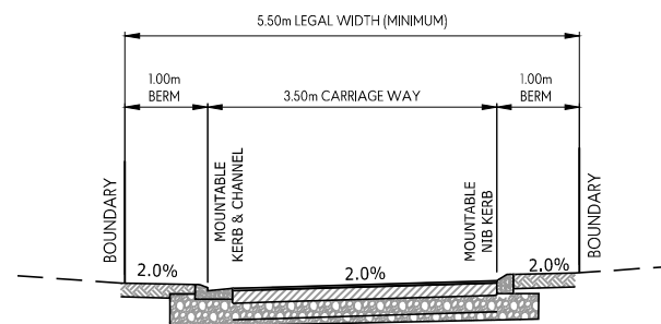
TYPICAL CROSS-SECTION - JOAL TYPE 3 5.5m (3.5m) SCALE: 1:50-A1 1:100-A3
