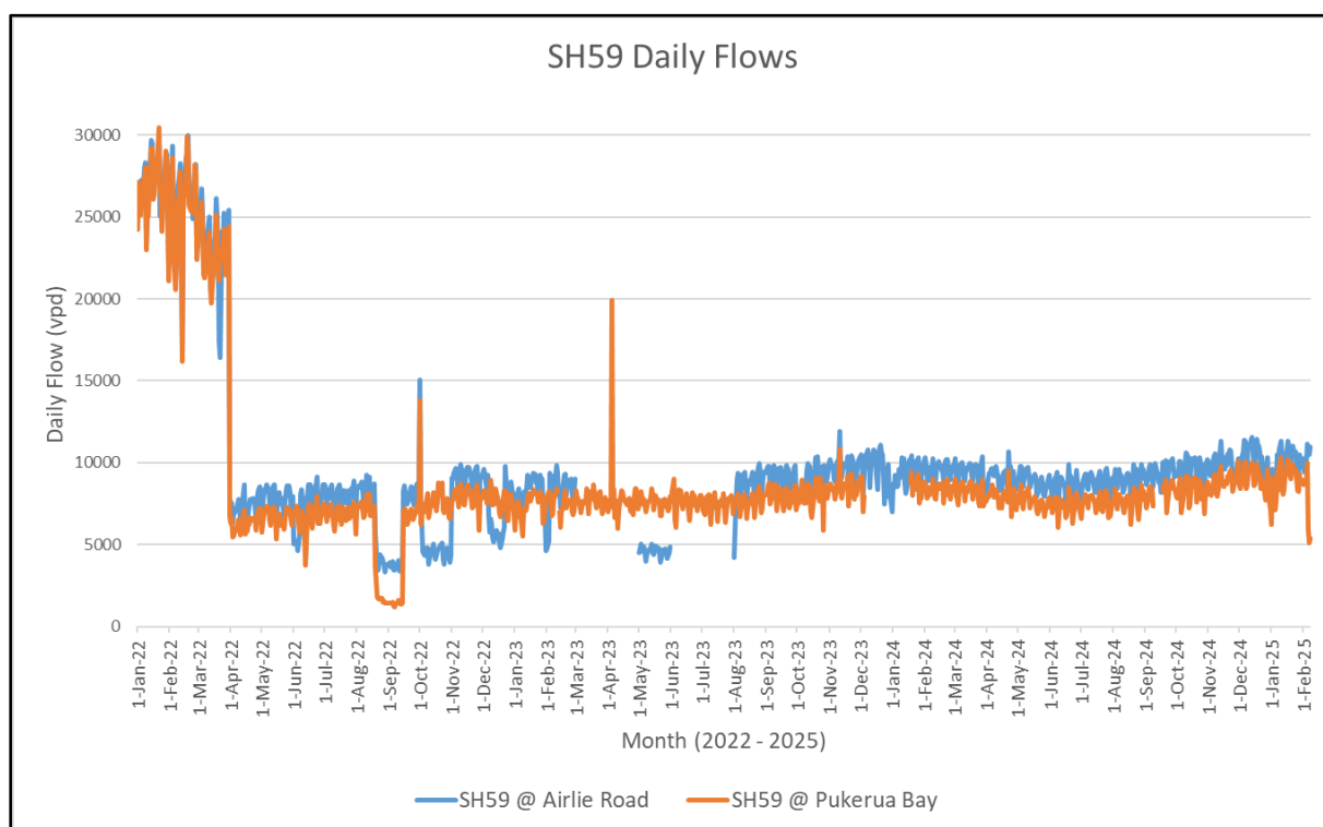
Figure 3-3: Daily Traffic Flows on SH59 at Airlie Road and Pukerua Bay (NZTA TMS)
