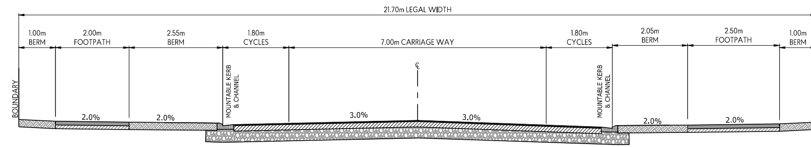
TYPICAL CROSS-SECTION - TYPE B COLLECTOR ROAD - 21.7m WITH CYCLEWAY AND BERM SCALE: 1:50-A1 1:100-A3
