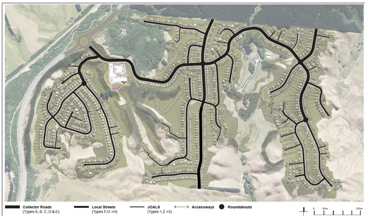
Figure 8-1: Site Roding Layout
