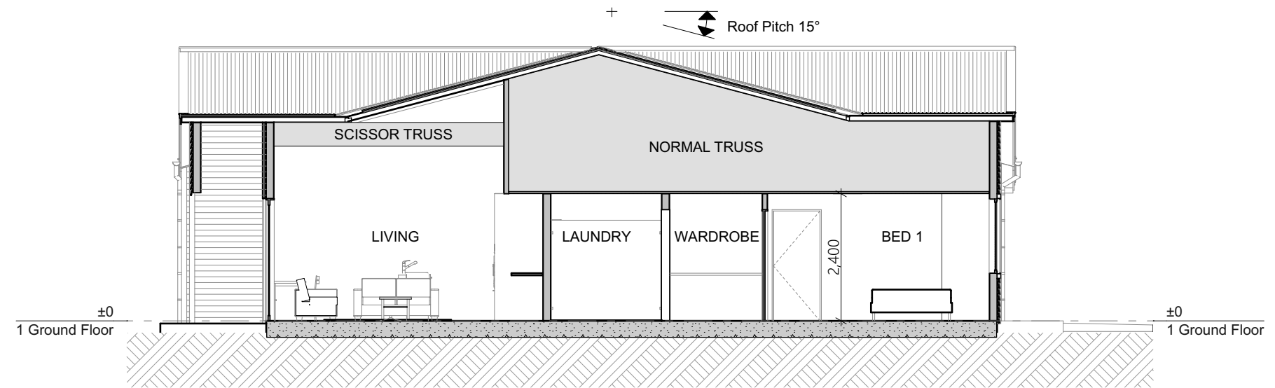
Section 1 1:100
