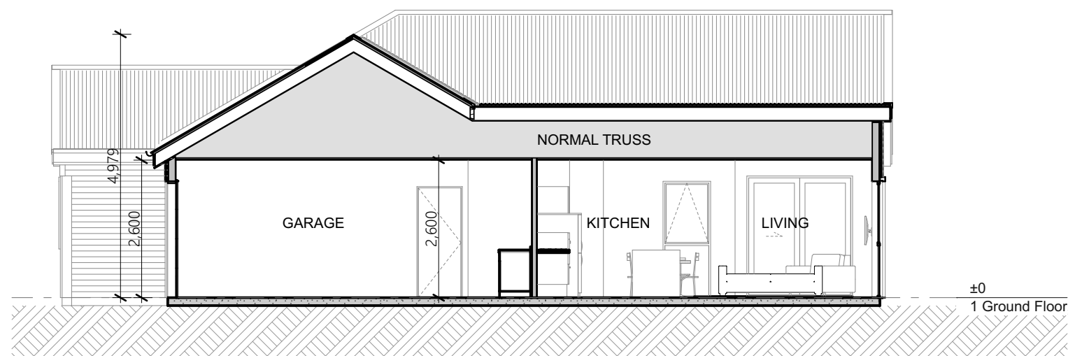
Section 3 1:100
