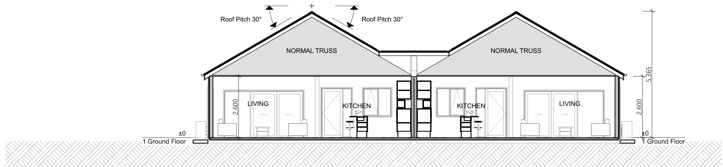
Section 2 1:100
