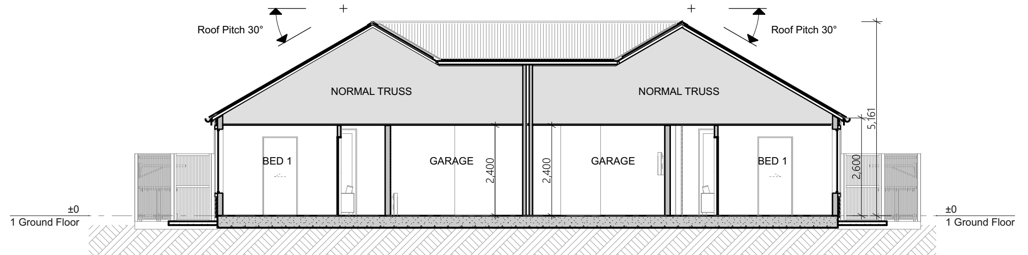
Section 2 1:100
