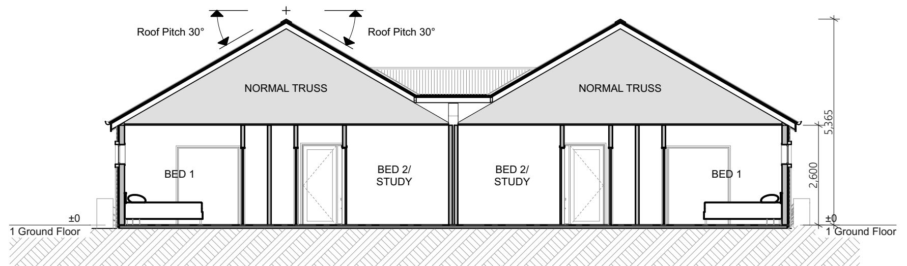
Section 3 1:100
