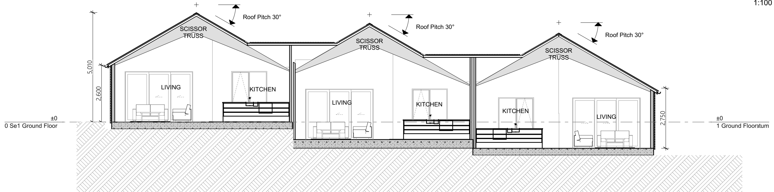
Section 2 1:100
