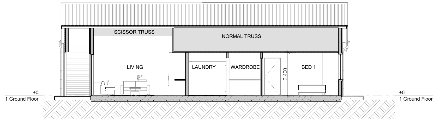
Section 1 1:100
