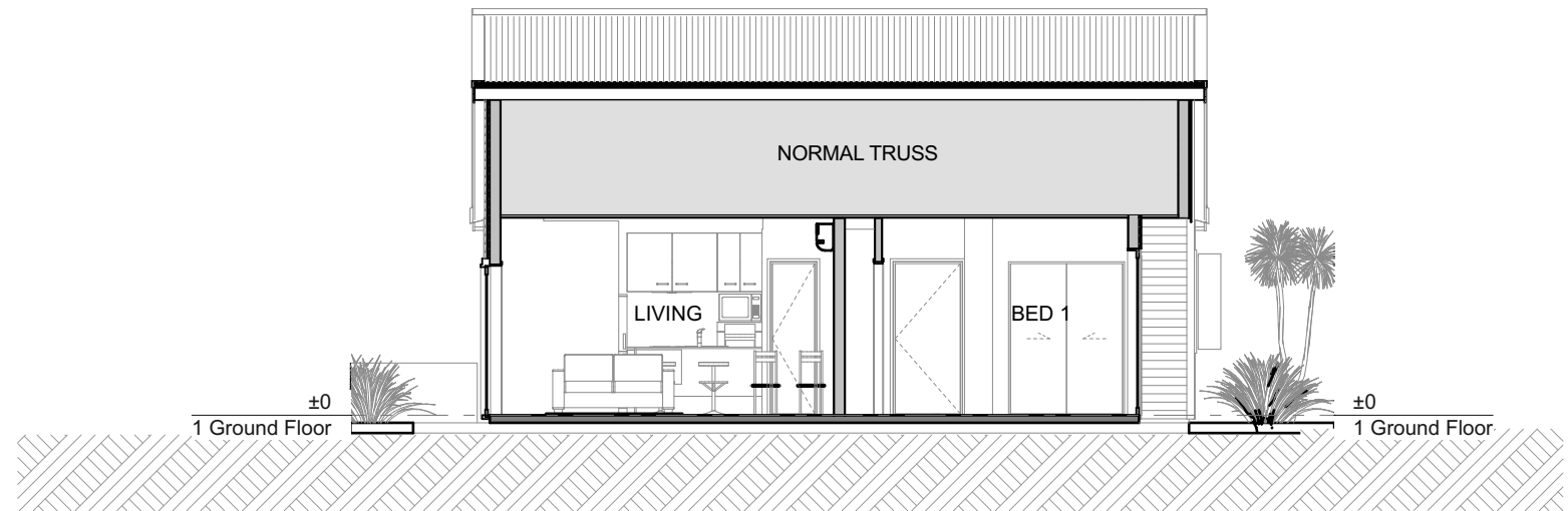
Section 1 1:100
