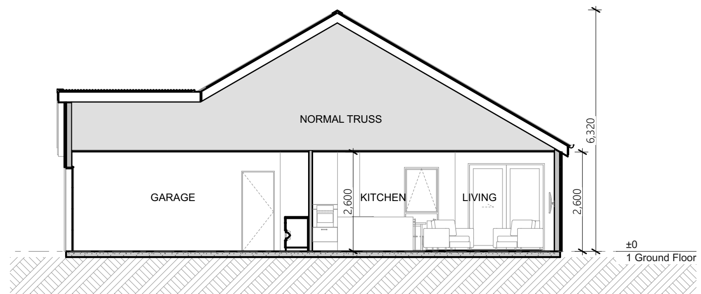
Section 3 1:100
