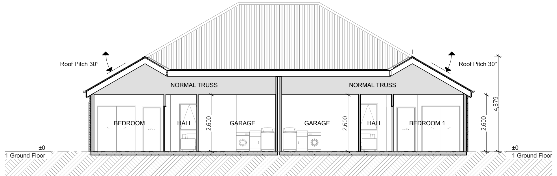
Section 2 1:100
