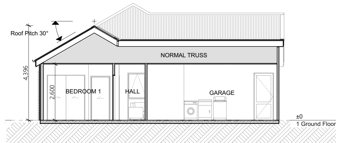
Section 2 1:100
