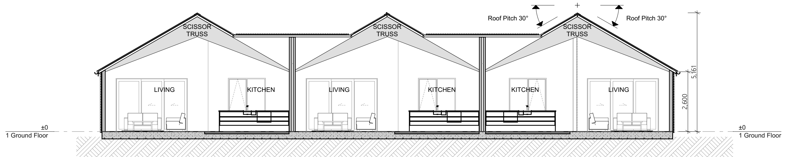
Section 2 1:100
