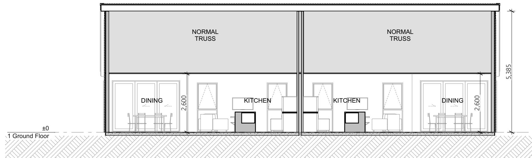
Section 1 1:100
