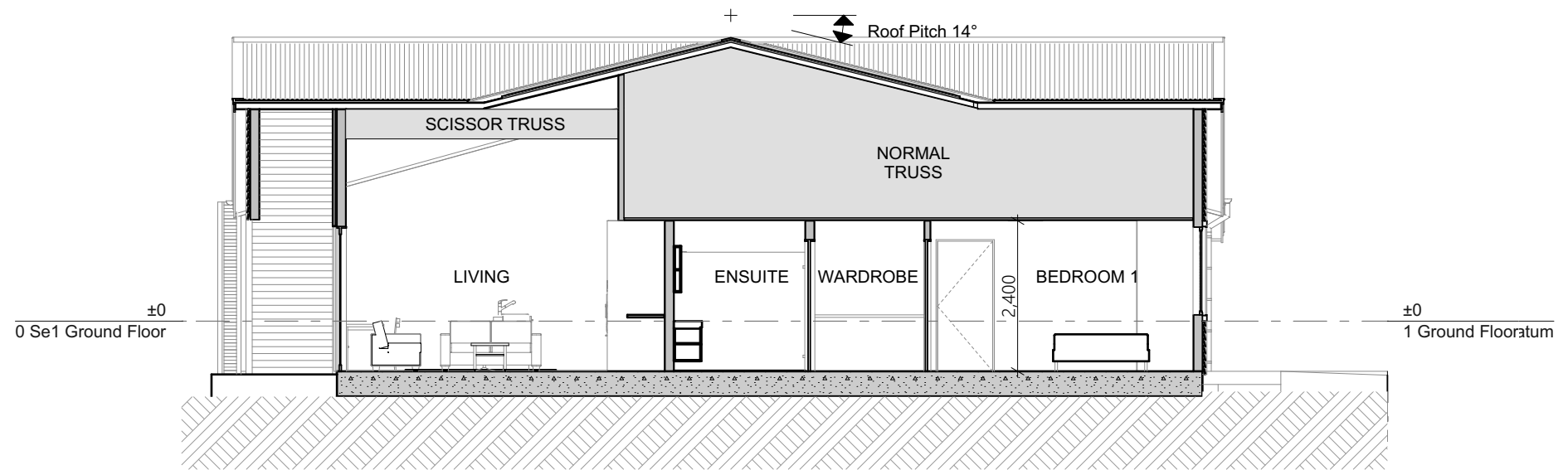
Section 1 1:100
