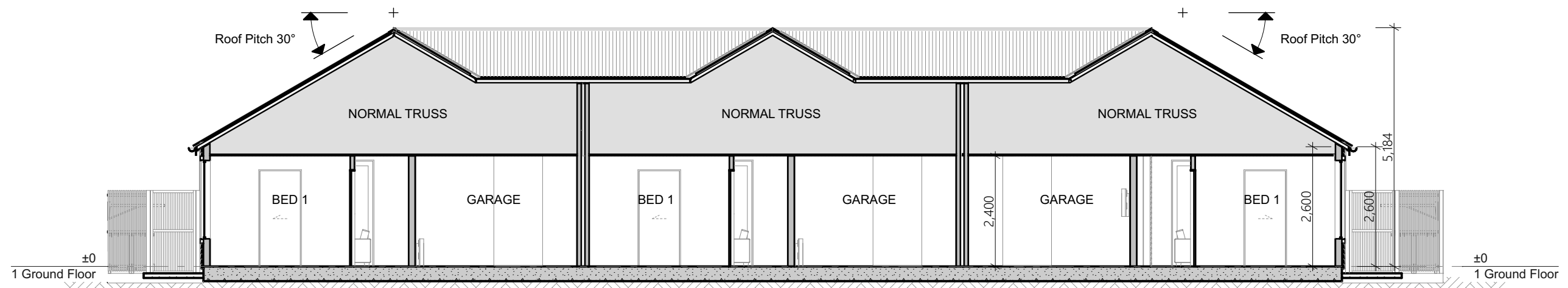
Section 3 1:100
