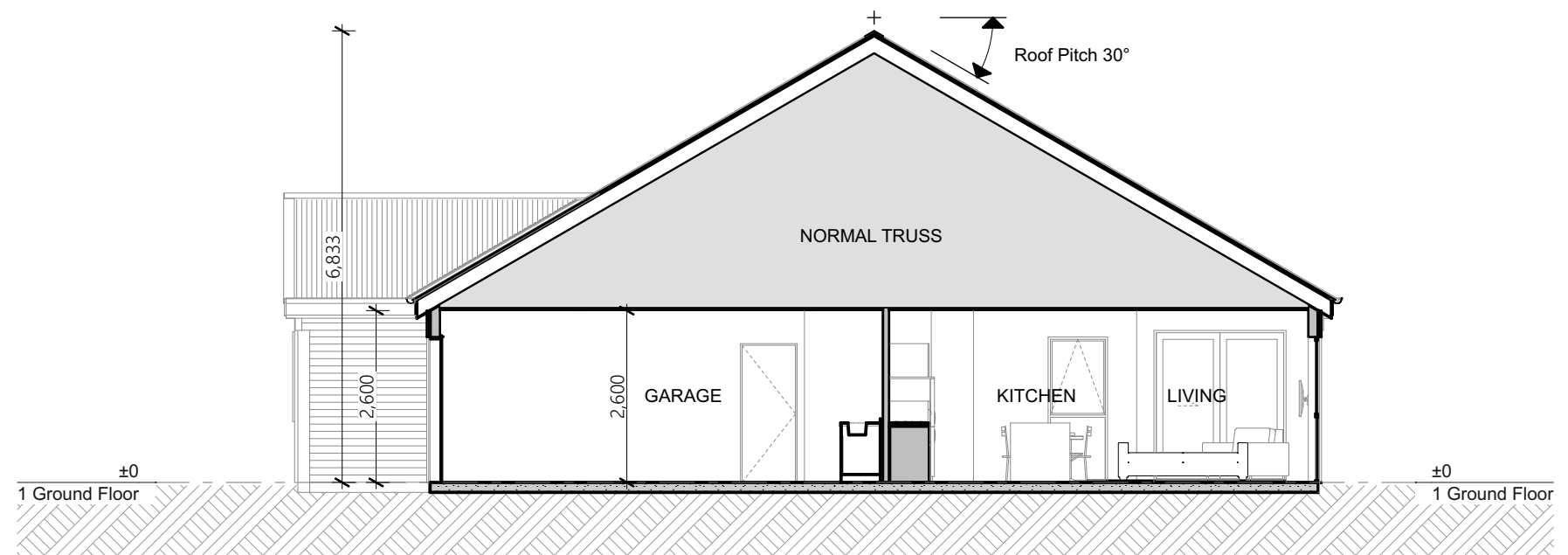
Section 3 1:100
