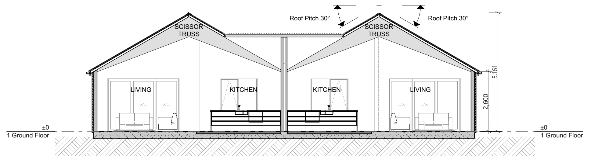
Section 2 1:100
