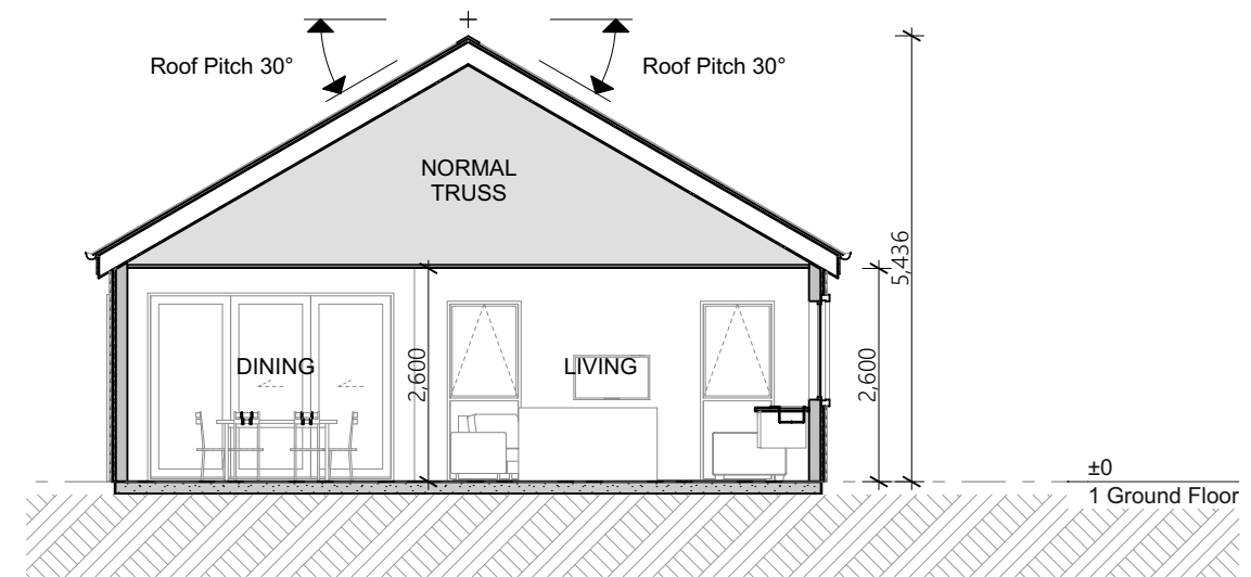
Section 1 1:100
