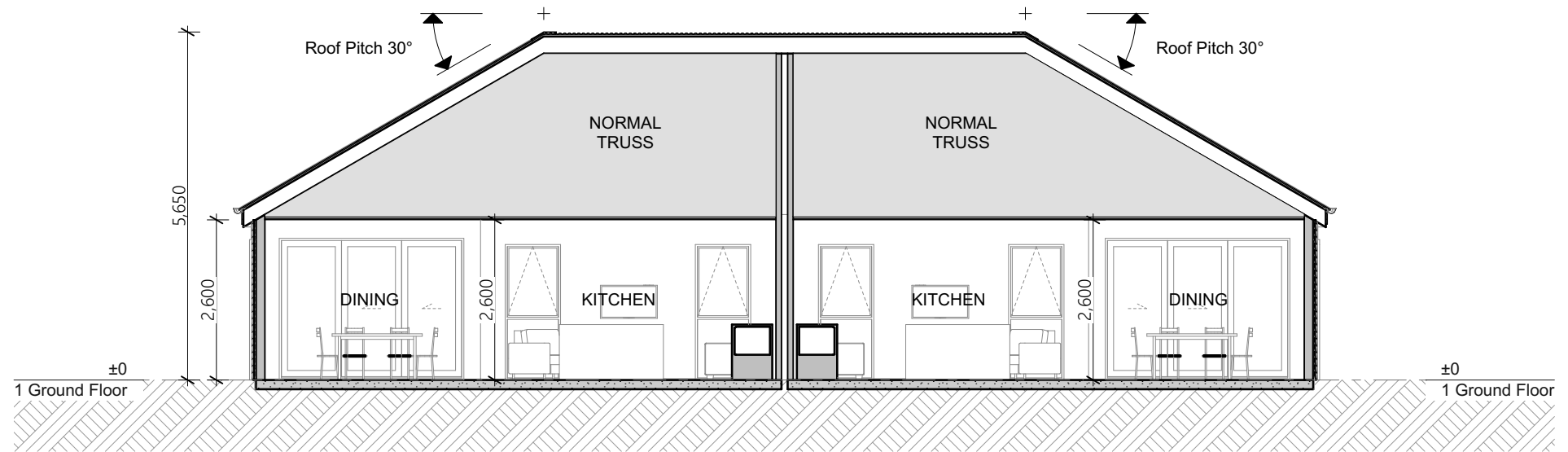
Section 1 1:100
