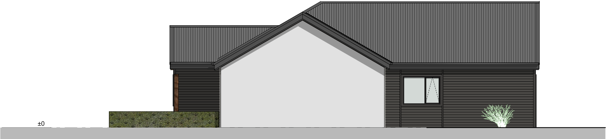
North Elevation 1:100
