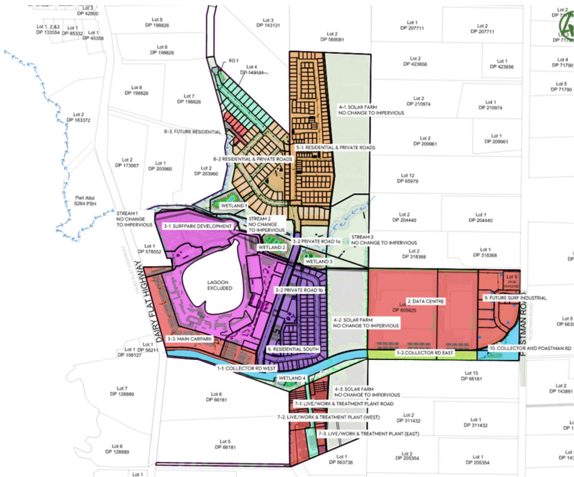
Figure 16 – Stormwater Management Device Catchment Plan (Source: Proposed Catchment Plan by MCCL)
