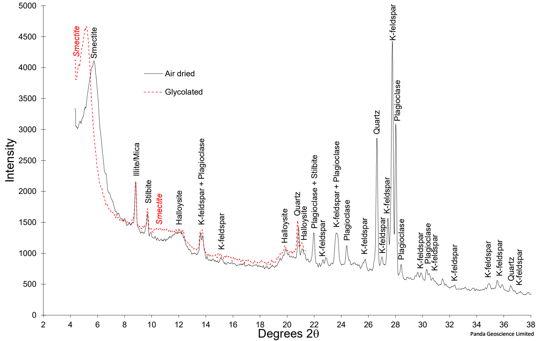
XRD: Sample BH2B_1157 43.50-43.75. Clay separate, air dried and glycolated, smoothed
