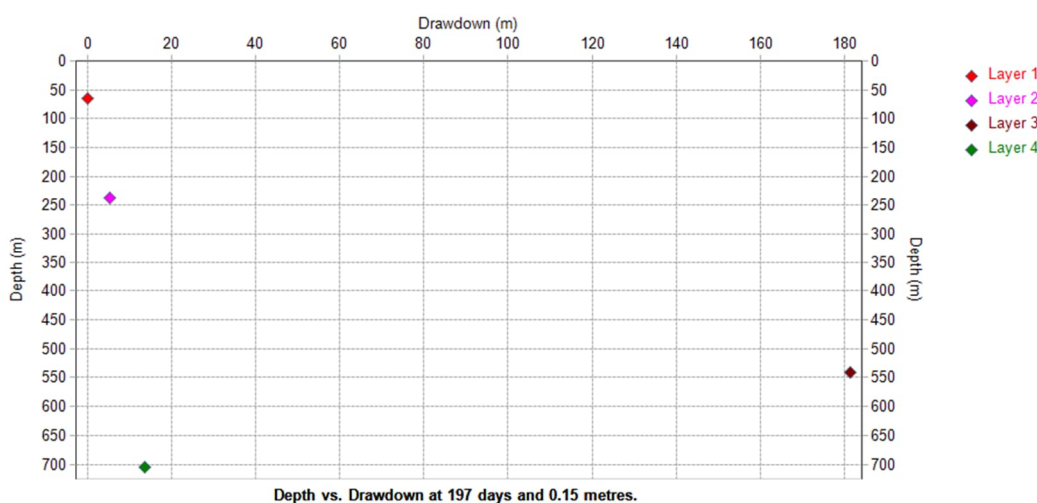
Figure 4. Simulated drawdown in each model layer at the Applicant's bore.
