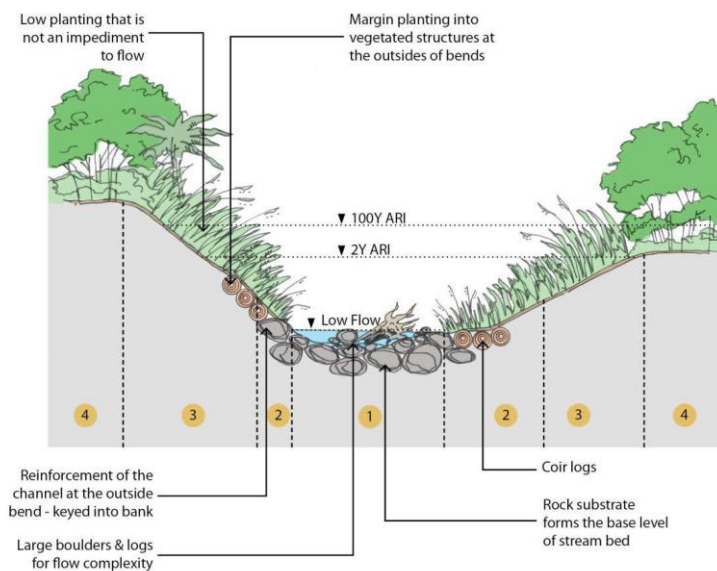
Figure 313132: Example of a channel design, illustrating a low flow channel and the use of rocky substrates and woody debris.
