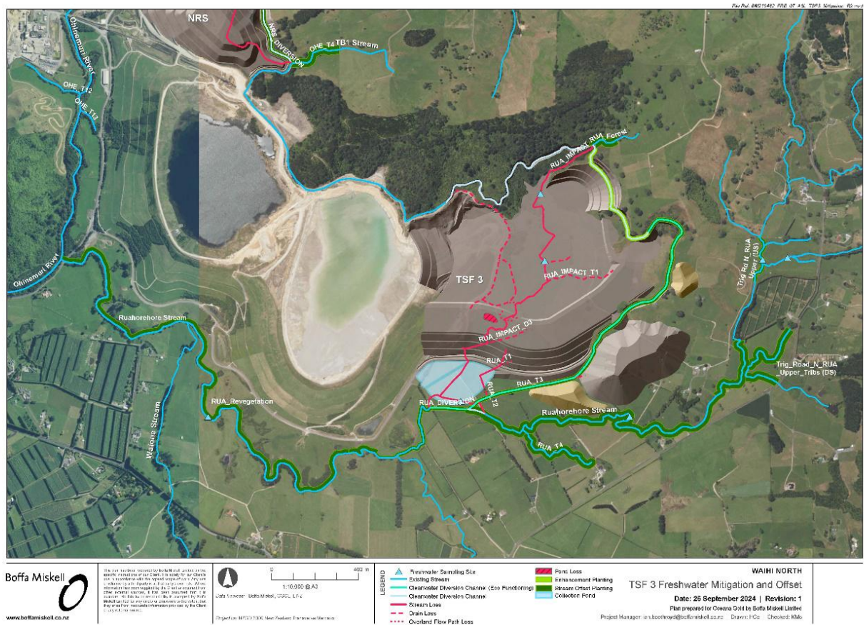
Figure 303631: Map of the existing Ruahore Stream and Tributaries, and proposed TSF3 Diversion.
