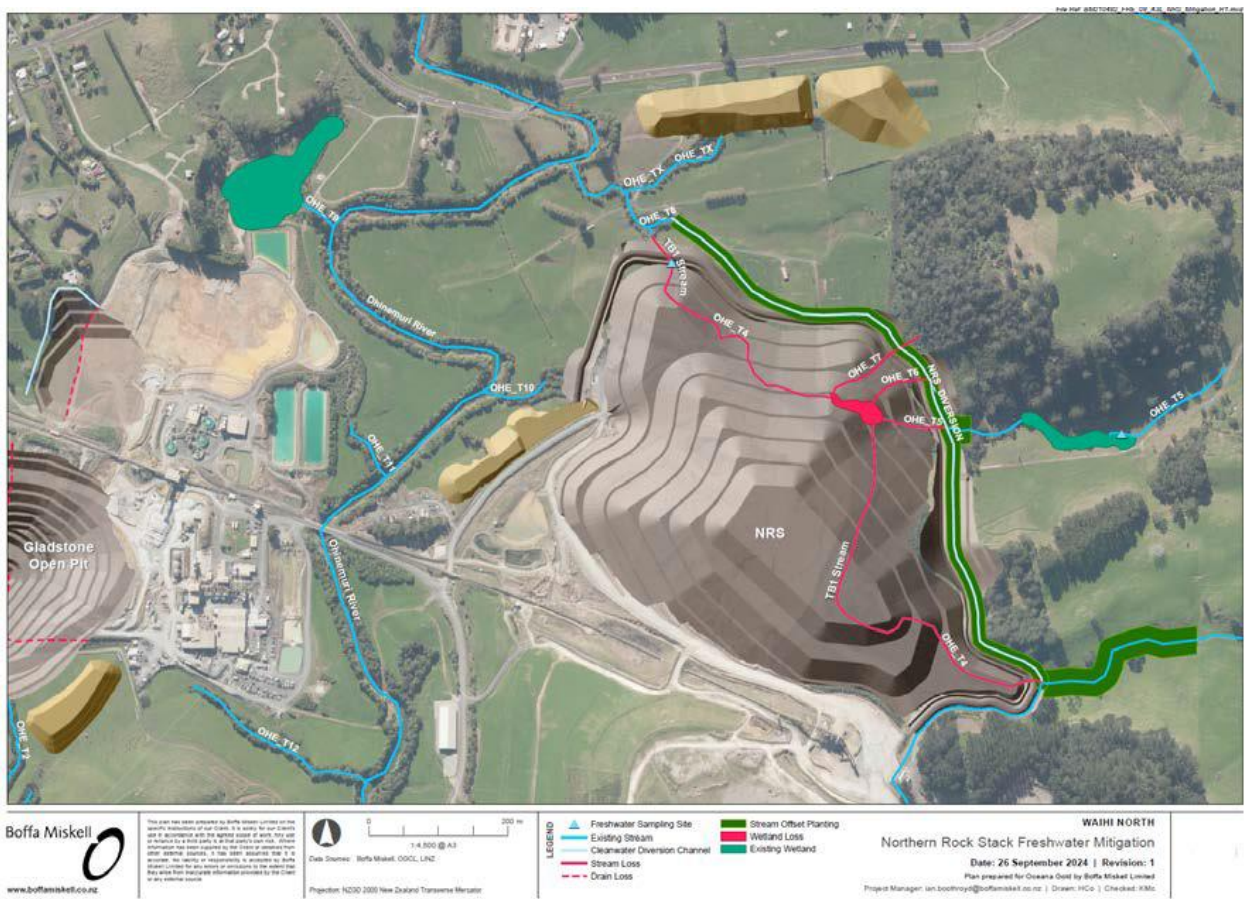
Figure 29: Map of the existing TB1 Stream and proposed NRS Diversion.
