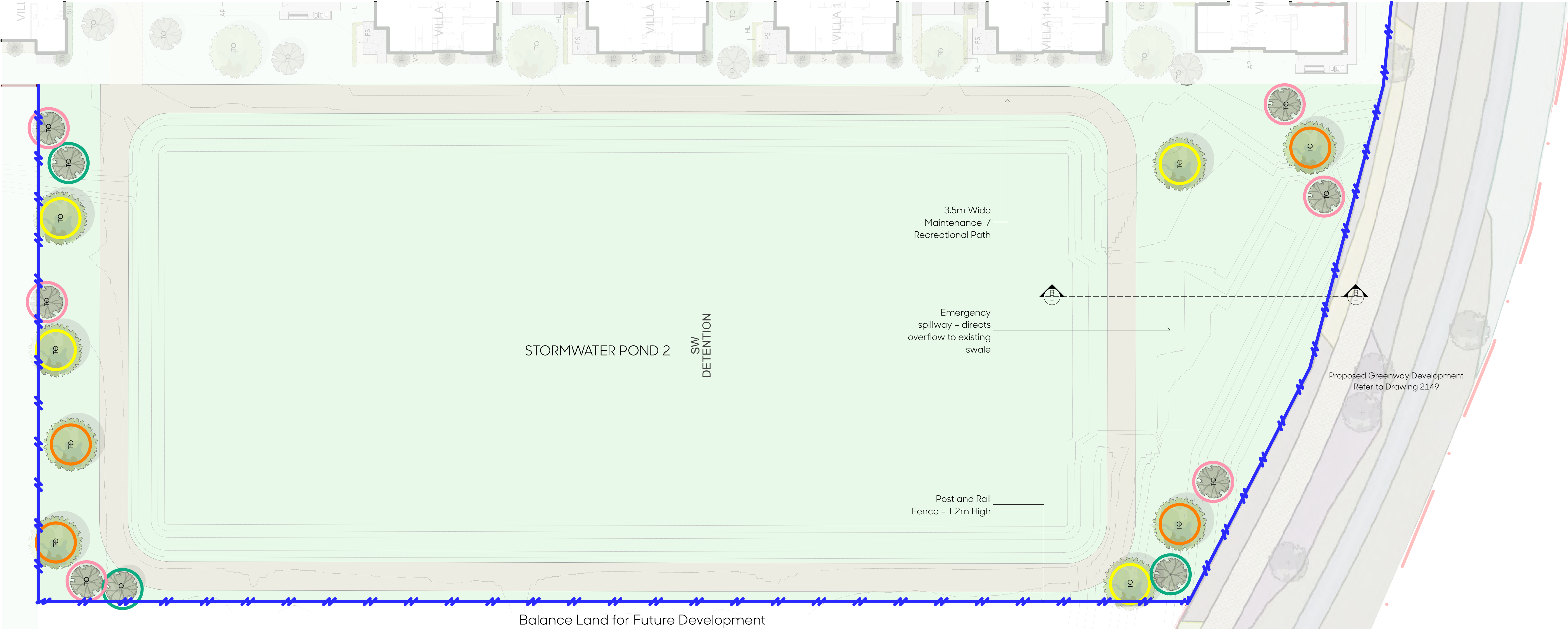
PLAN : STORMWATER POND 2 1:250@A1 / 1:500@A3
