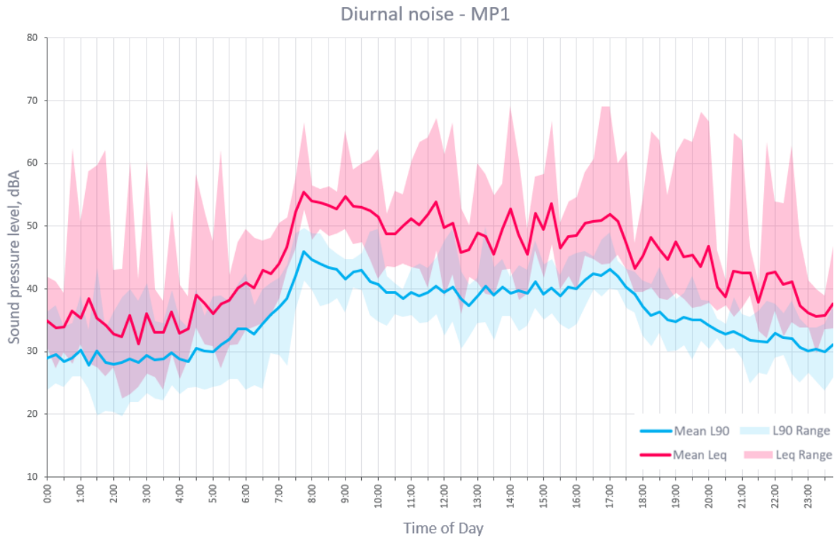
Figure 9: MP1 Full noise data
