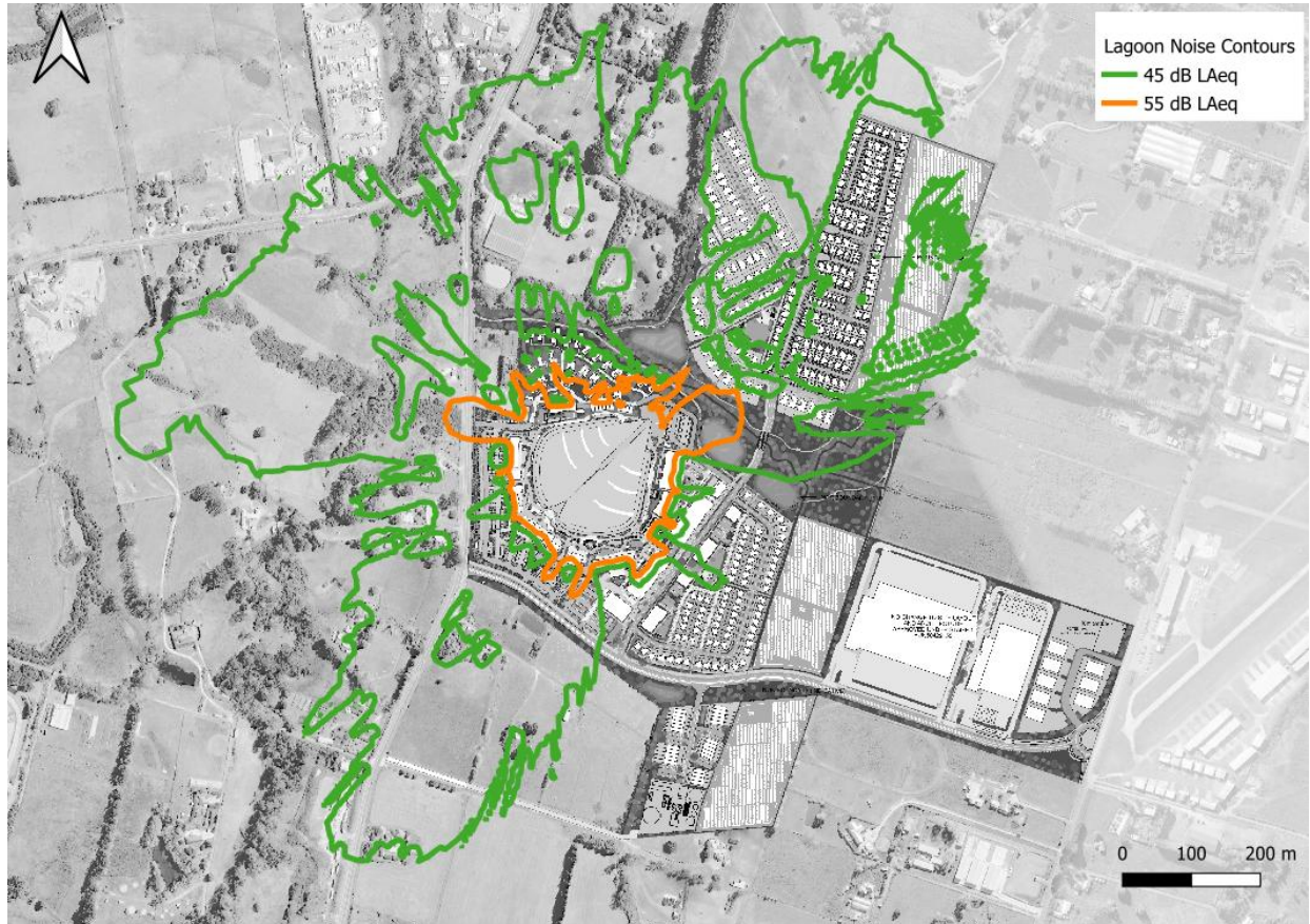
Figure 11 Surf lagoon noise contours
