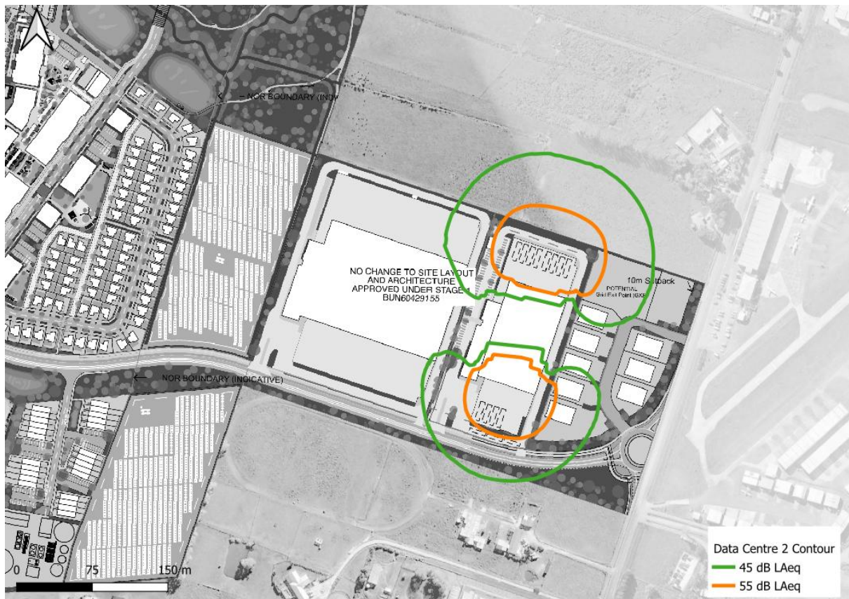
Figure 13 Data Centre 2 noise contour
