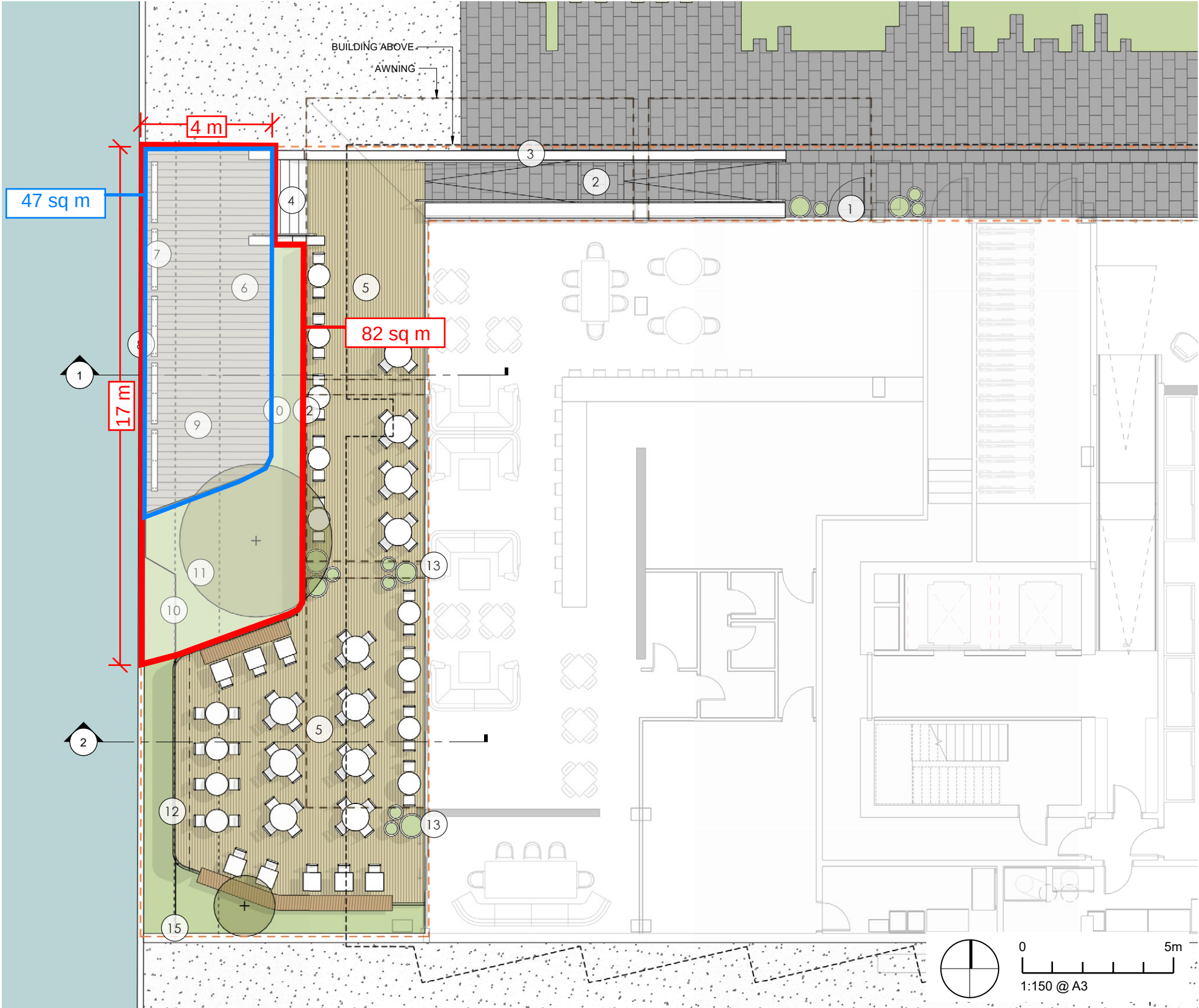
PLAN SHOWING GROUND FLOOR LAYOUT
