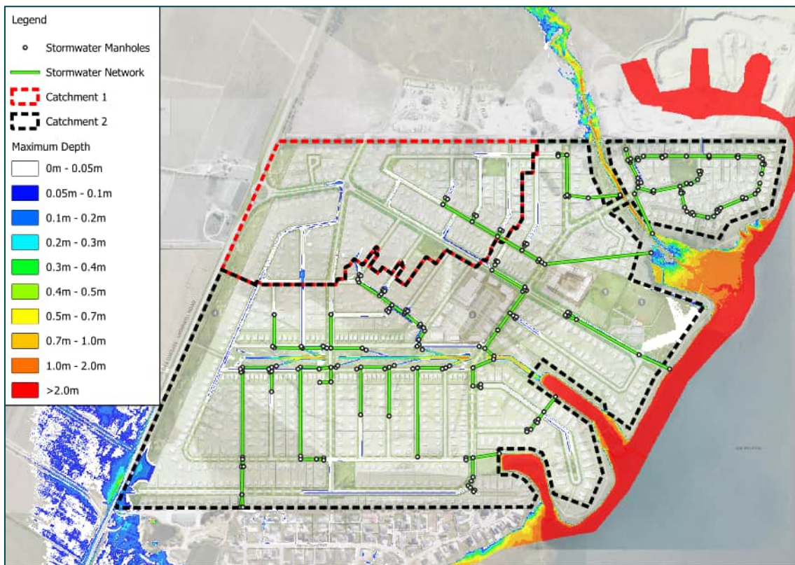
Figure 15: 5-year ARI internal flooding
