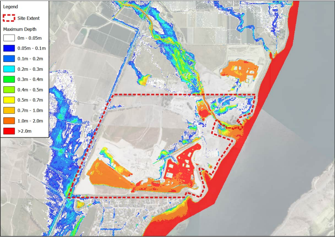
Figure 10: Predevelopment 100-year ARI RCP8.5
