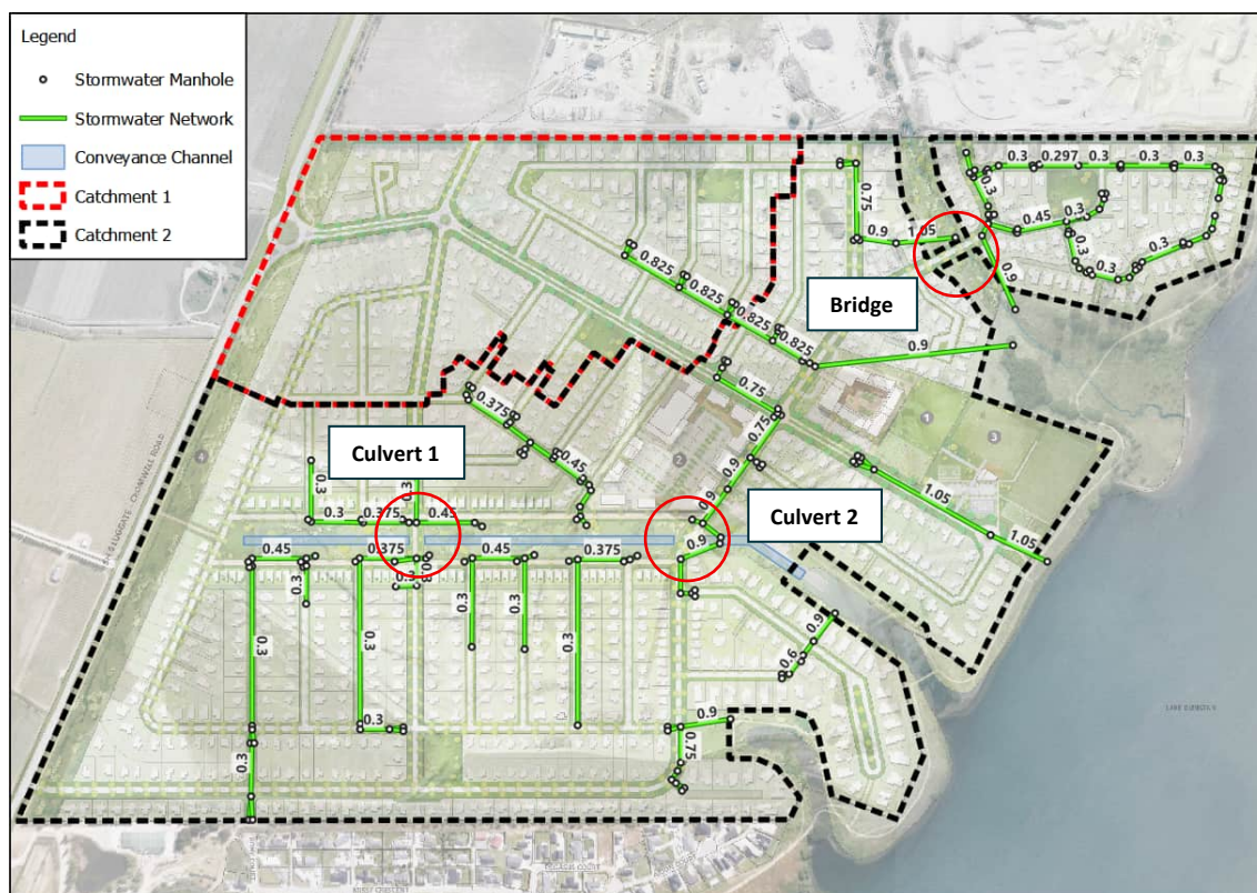
Figure 8: Preliminary stormwater pipe network
