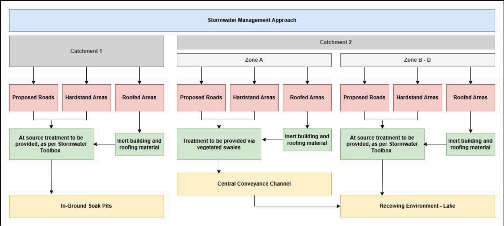
Figure 9: Stormwater Management Summary
