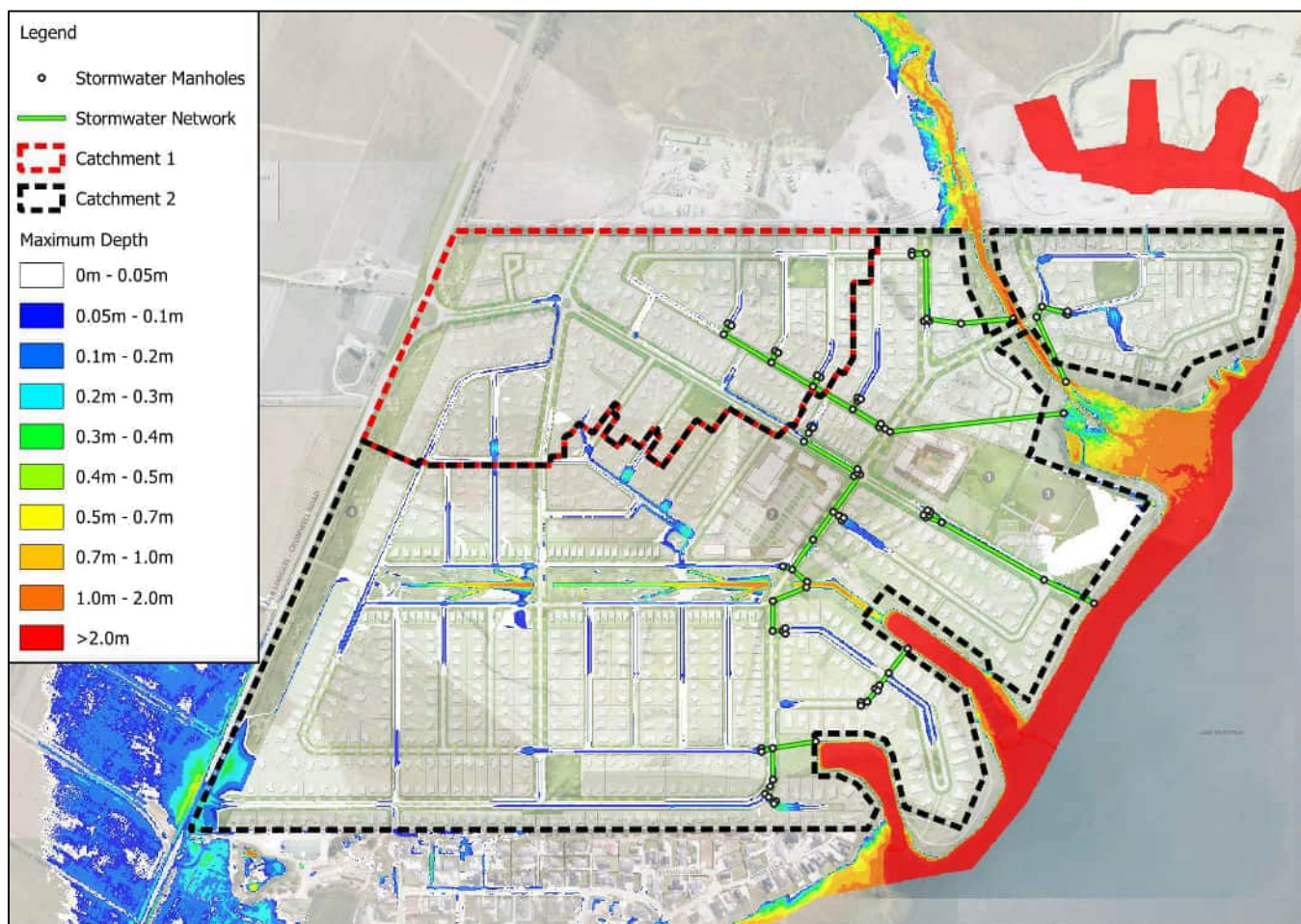
Figure 16: 100-year ARI internal flooding
