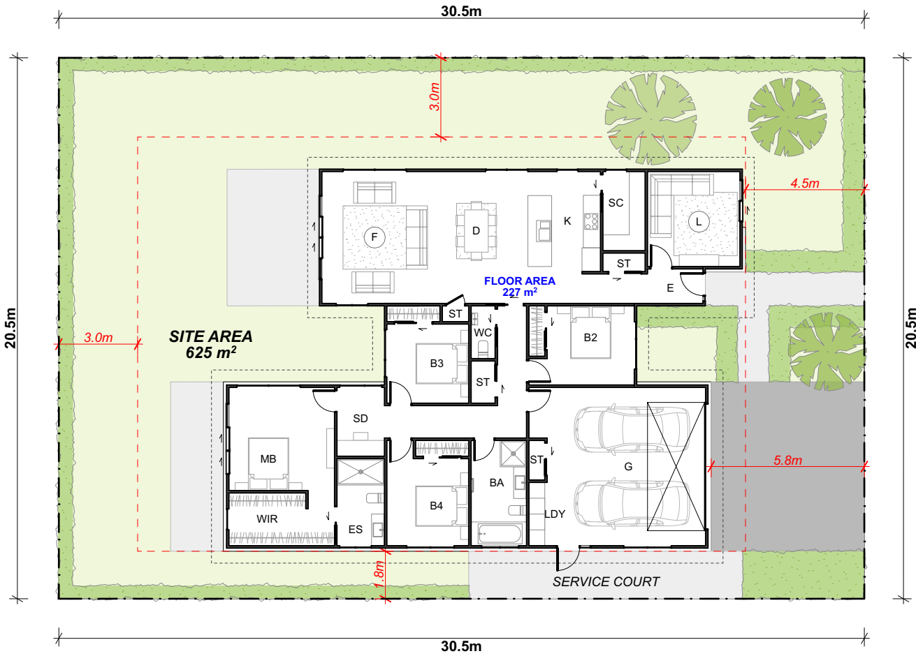
4 - INDICATIVE BUILDING LAYOUT 1:200
