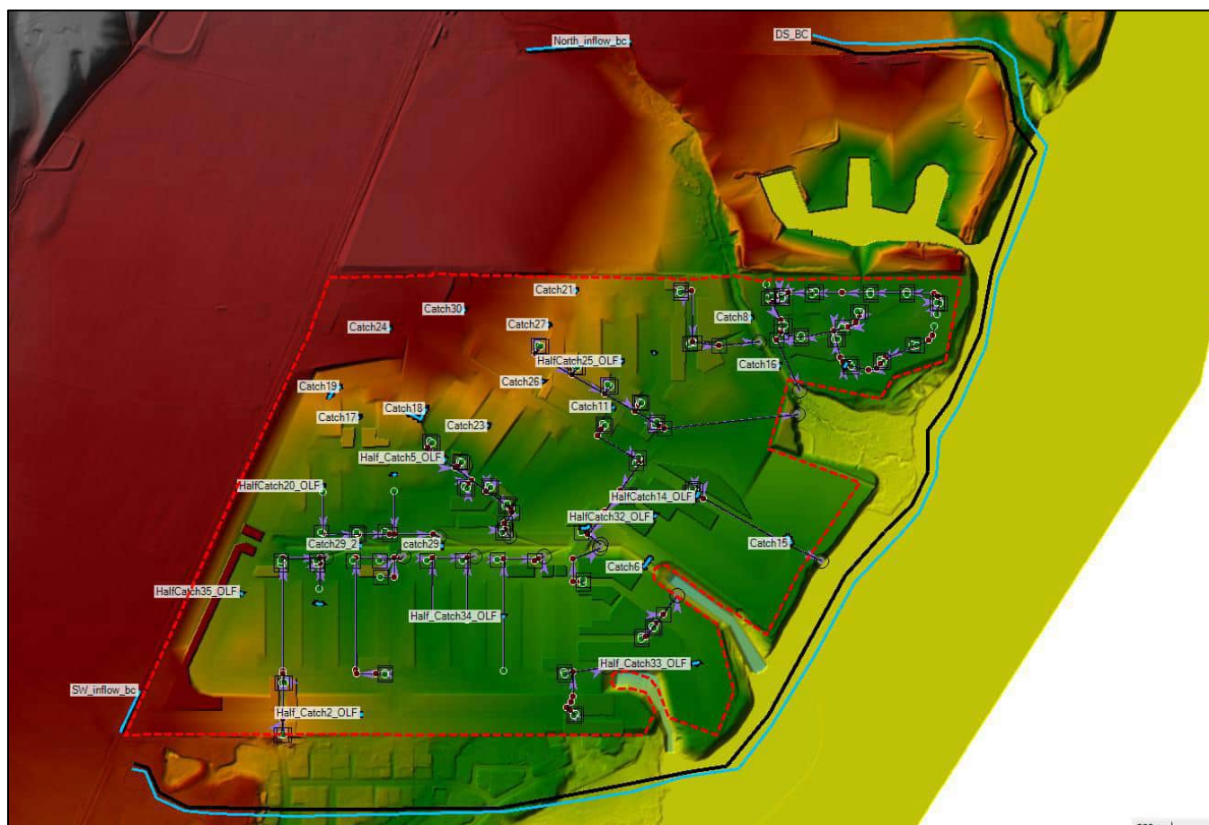
Figure 8: Internal model boundary conditions
