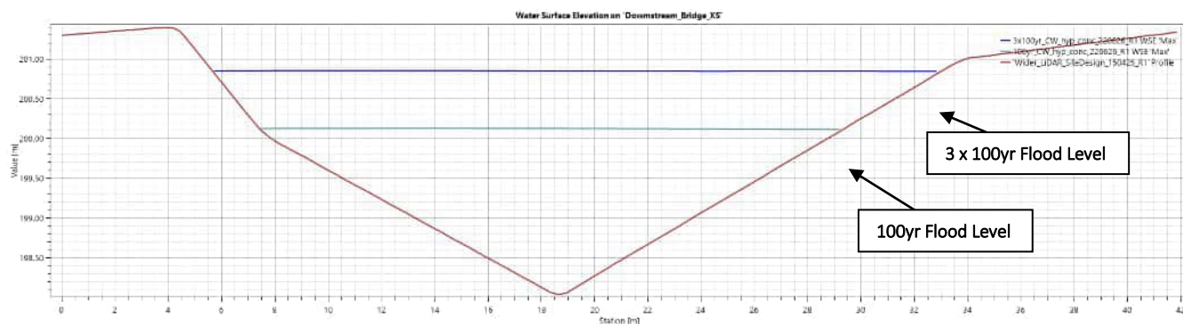
Figure 19: Downstream flood levels (1x100yr vs 3x100yr events)
