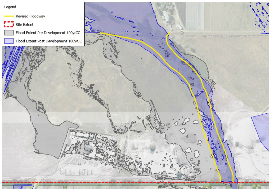
Figure 12: Flooding upstream Bonisch Site
