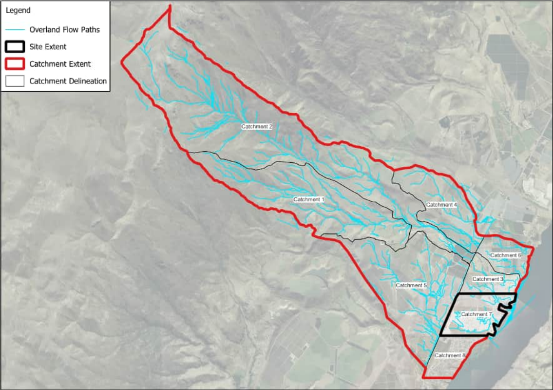
Figure 3: Existing overland flow paths (wider catchment)
