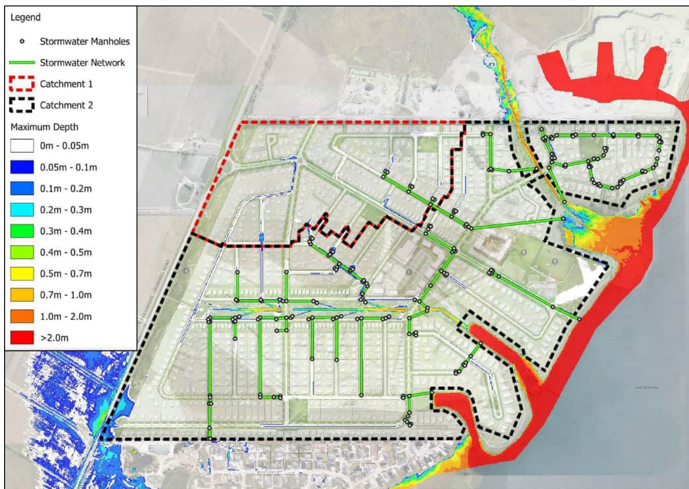
Figure 15: 10-year ARI internal flooding
