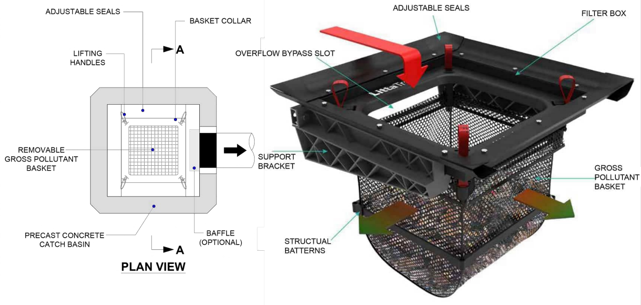
LITTATRAP™ COMPONENTS
