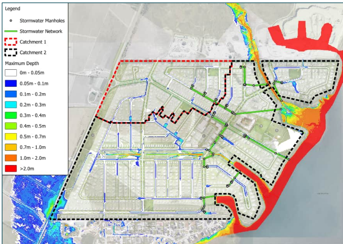
Figure 17: 100-year ARI internal flooding
