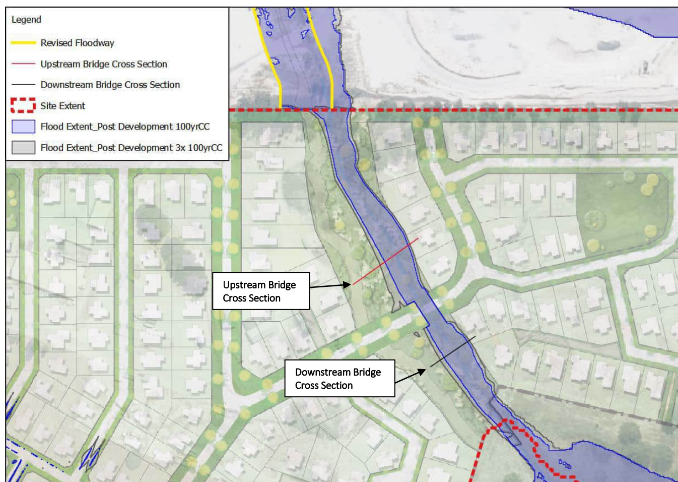
Figure 17: Extreme flood levels through drainage corridor
