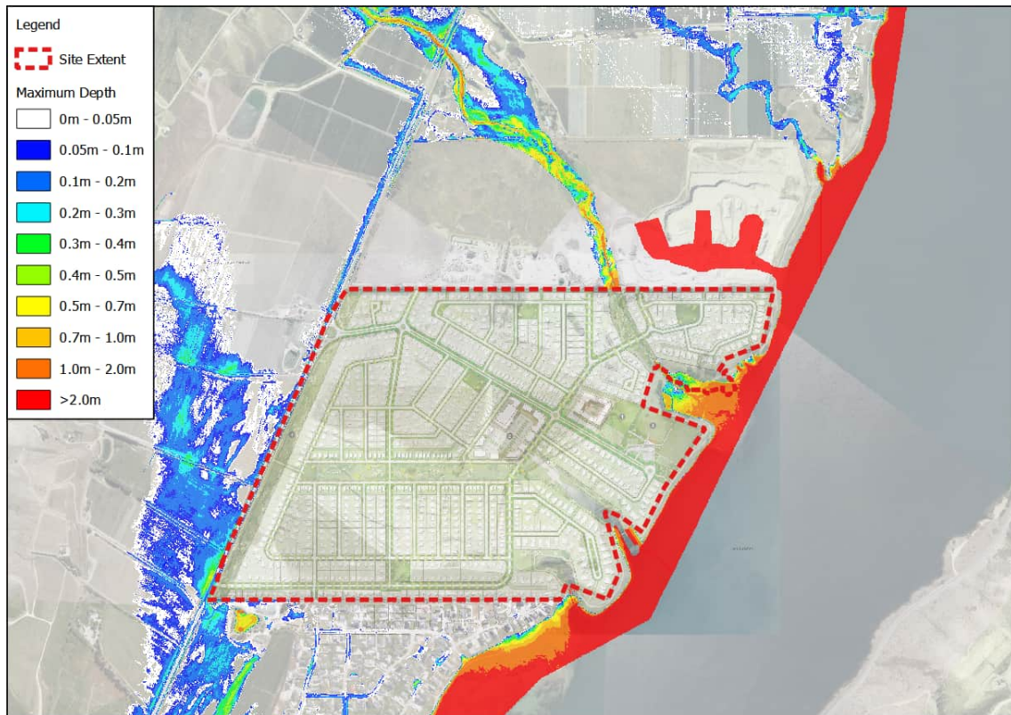
Figure 11: Post development 100-year ARI RCP8.5
