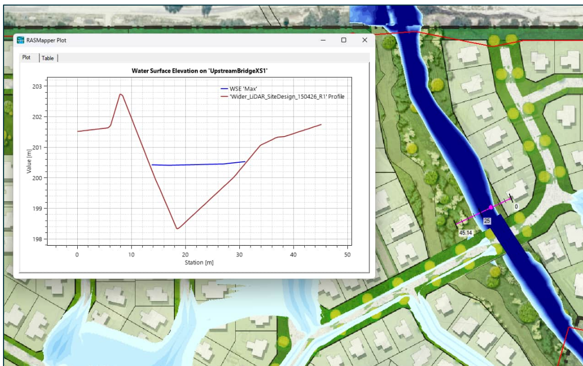
Figure 14: Flooding within Parkburn Site along corridor
