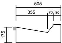
No. 8 Type Mountable Kerb & Channel
