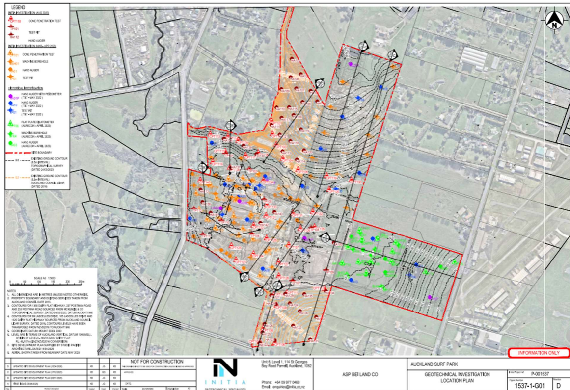
Figure 10 - Location of Geotechnical Boreholes (Source: Geotechnical Factual Report Rev G, Initia, April
