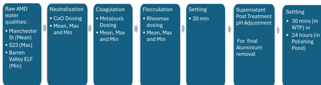
Figure 1 Treatment Processes used in Confirmation Testing
