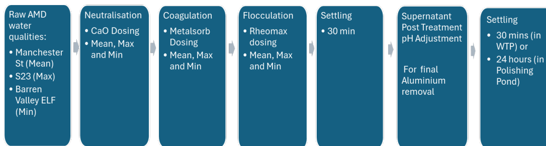
Figure 33 Treatment Processes used in Confirmation Testing
