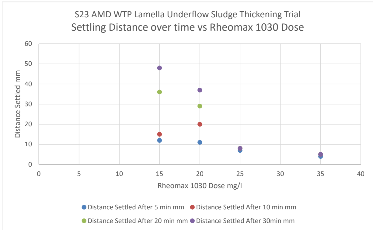
Figure 14 Sludge Thickening - Settling Distance over time - S23 AMD with Rheomax 1030
