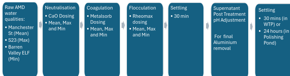
Figure 4 Treatment Processes used in Confirmation Testing
