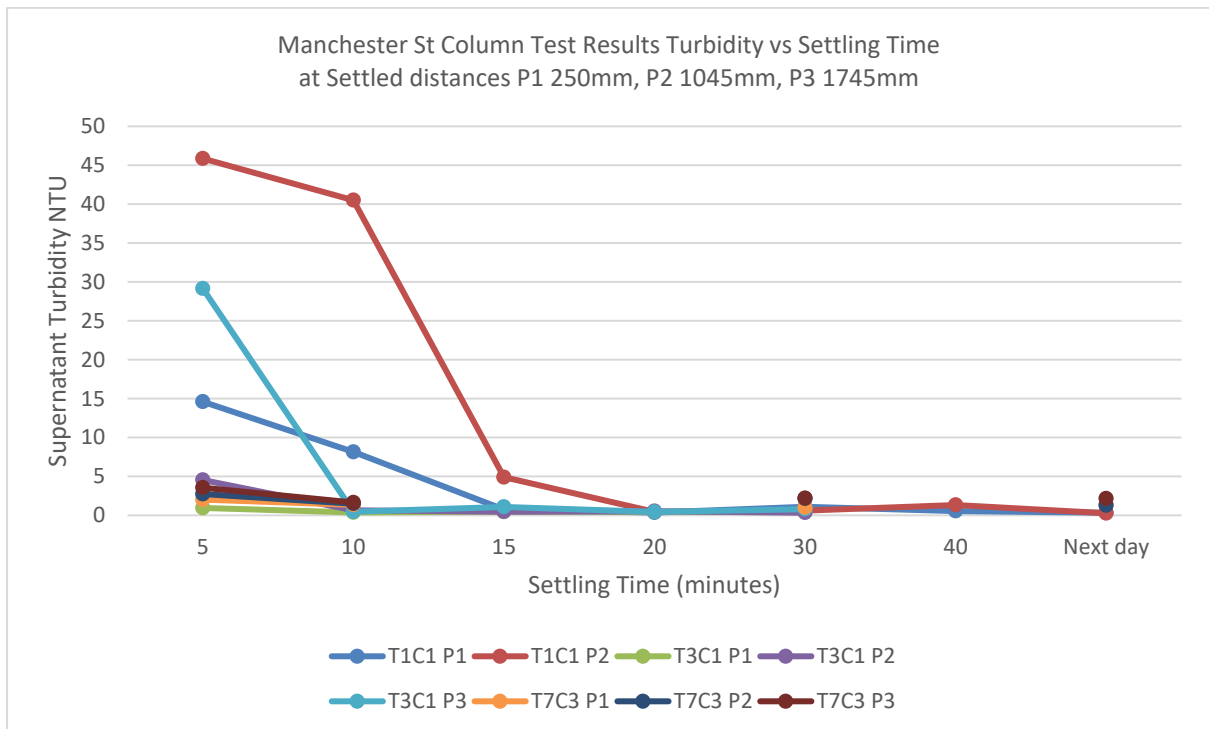
Figure 13 Manchester Turbidity vs Settling Time
