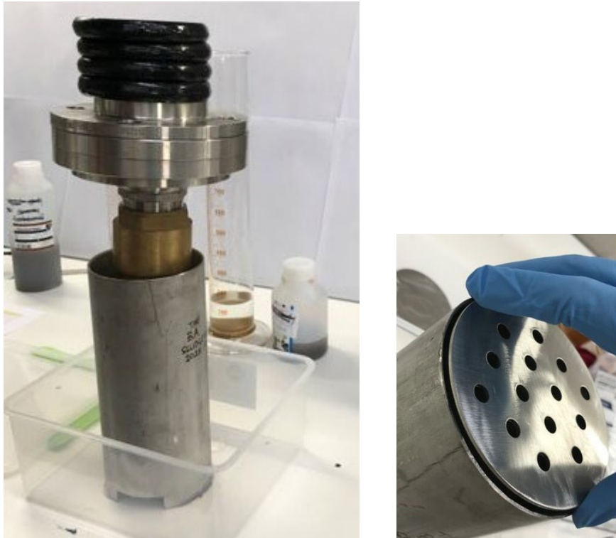
Figure 19 Pressure Dewatering Assembly (Left) and Perforated Disc (Right)
