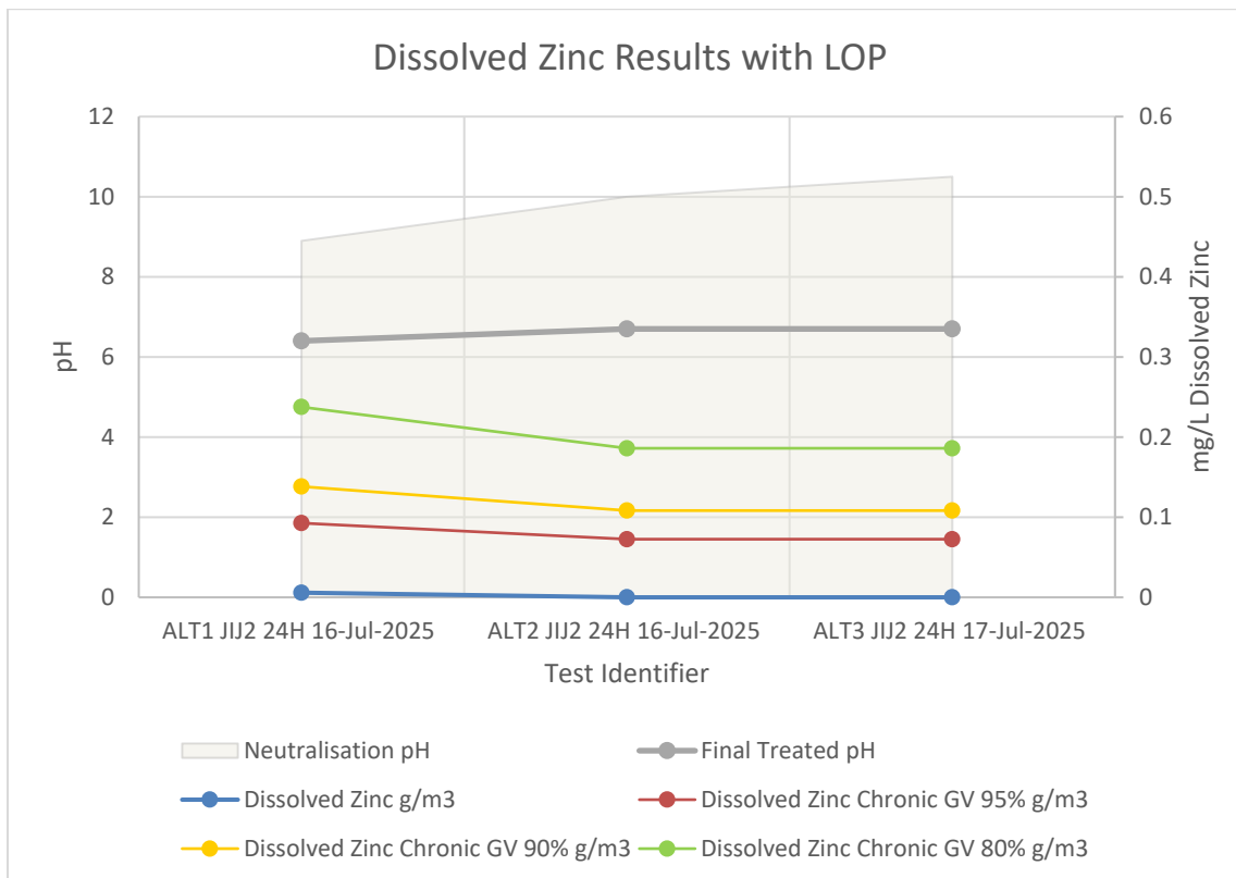
Figure 13 Dissolved Zinc Results
