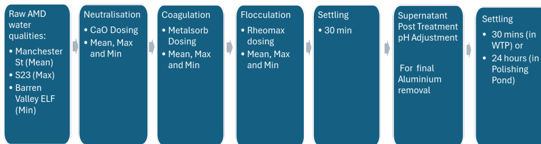
Figure 2 Treatment Processes used in Confirmation Testing
