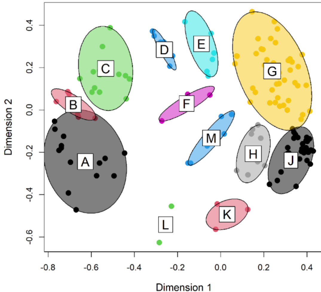
Figure 30: Ordination diagram showing the first two dimensions from a NMDS ordination using only the 35 principal species.
