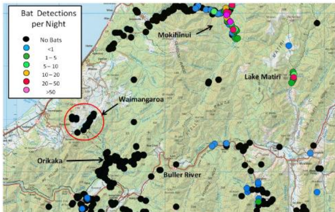
Figure 11: Acoustic bat survey results from the Northern South Island 2007 – 2013 (from Lloyd 2018, 2019).
