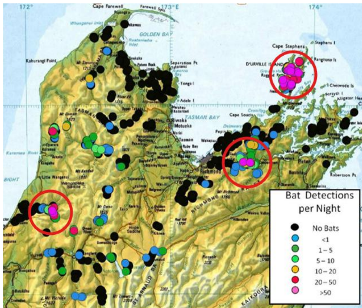
Figure 10: Acoustic bat survey results from the northern South Island 2007- 2013 (from Lloyd 2018, 2019).
