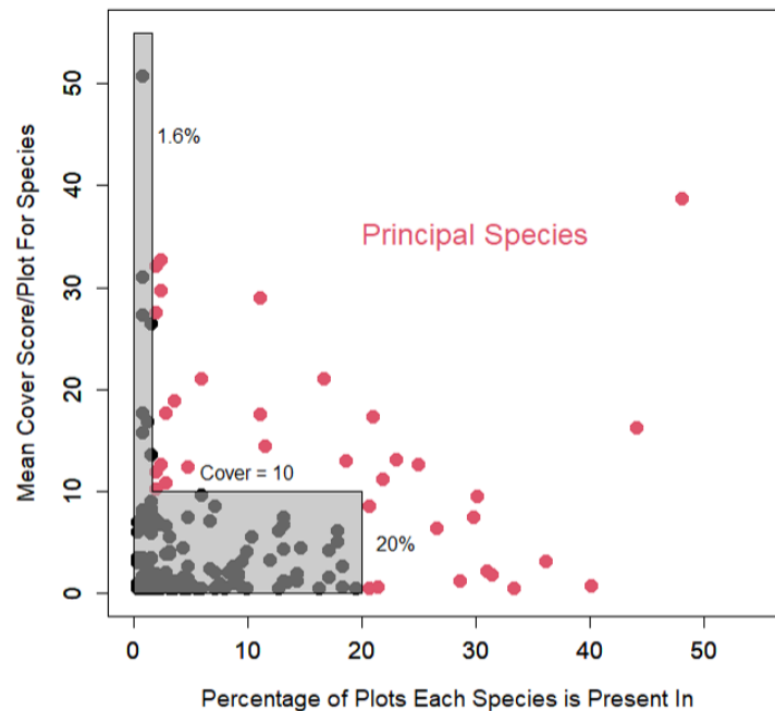
Figure 6: Mean cover score per plot and percentage of plots where they occurred for the 256 species recorded at 147 plots. Red symbols are the 35 principal species defined in text.
