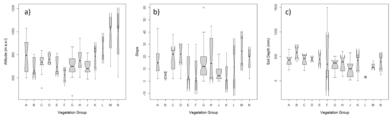
Figure 27: Box-and-whisker plots showing the distribution among ordination groups for: a) altitude (m a.s.l), b) slope (°) and c) soil depth (mm).
