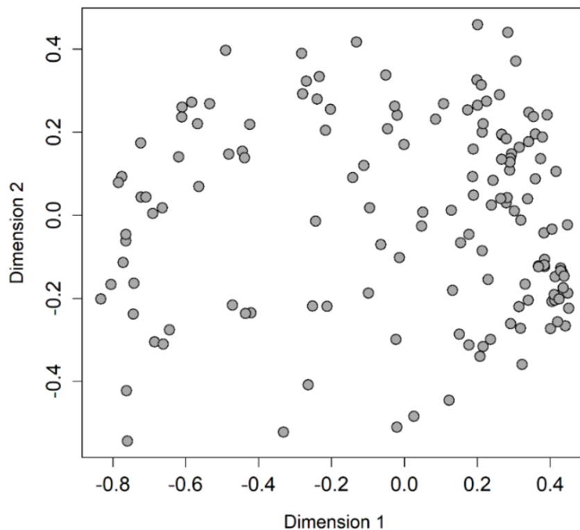
Figure 7: Ordination diagram from Non-metric Multidimensional Scaling (NMDS) showing the first two dimensions.
