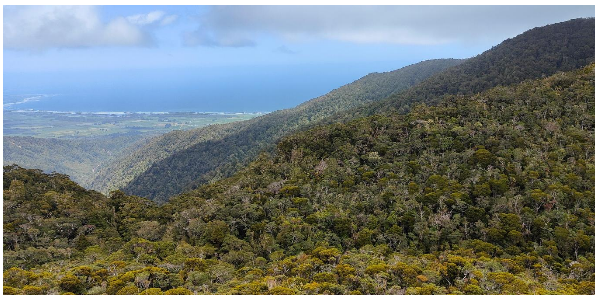
Figure 11: Southern rātā-mountain beech-podocarp forest near the Waimangaroa Gorge, showing dominant podocarps with emergent Southern rātā.
