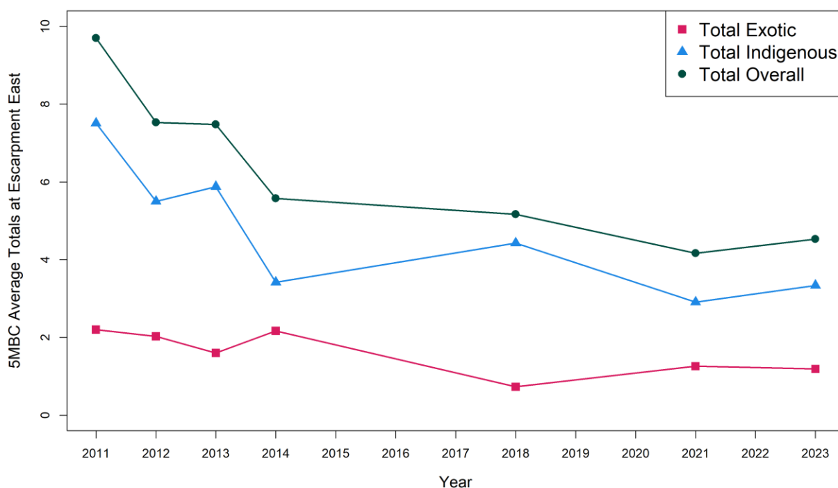
Figure 12: Average number of birds recorded in 5MBCs at Escarpment East.
