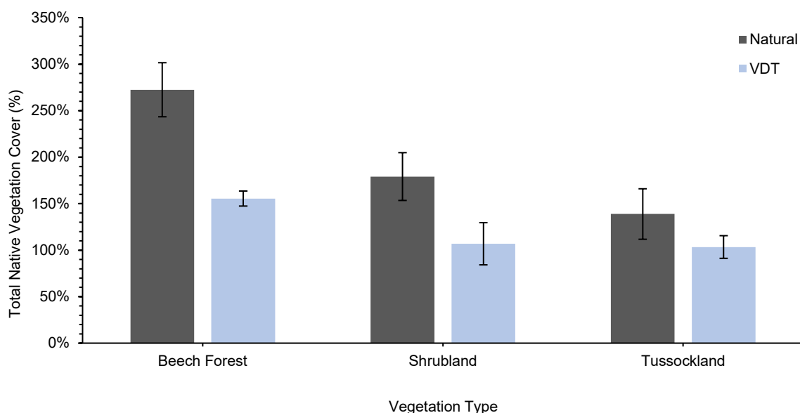
Figure 19: Mean ( \pm SE) percentage cover of native species at natural and VDT sites by vegetation type.
