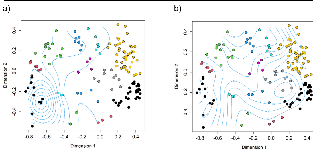
Figure 25: Ordination diagram from NMDS overlayed by contours for a) average canopy top-height (m) and b) percentage canopy cover. The 13 clusters of plots are distinguished by colours.
