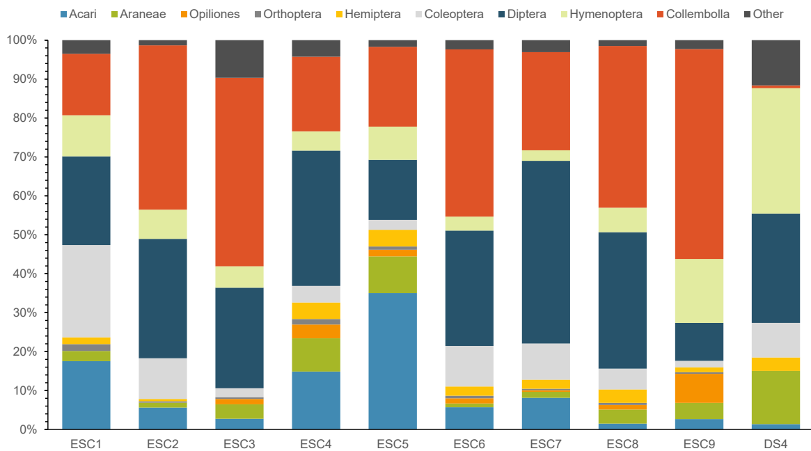
Figure 19: Terrestrial invertebrate community composition at each site within the Extended Escarpment Project sub-area.
