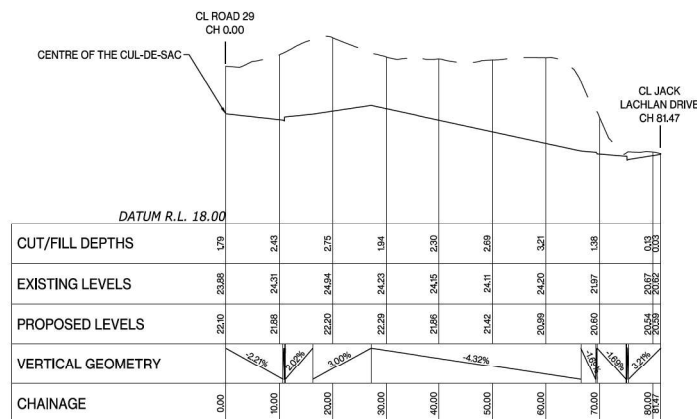
Coal 32 LONGSECTION BETWEEN 0.00 AND 81.47
