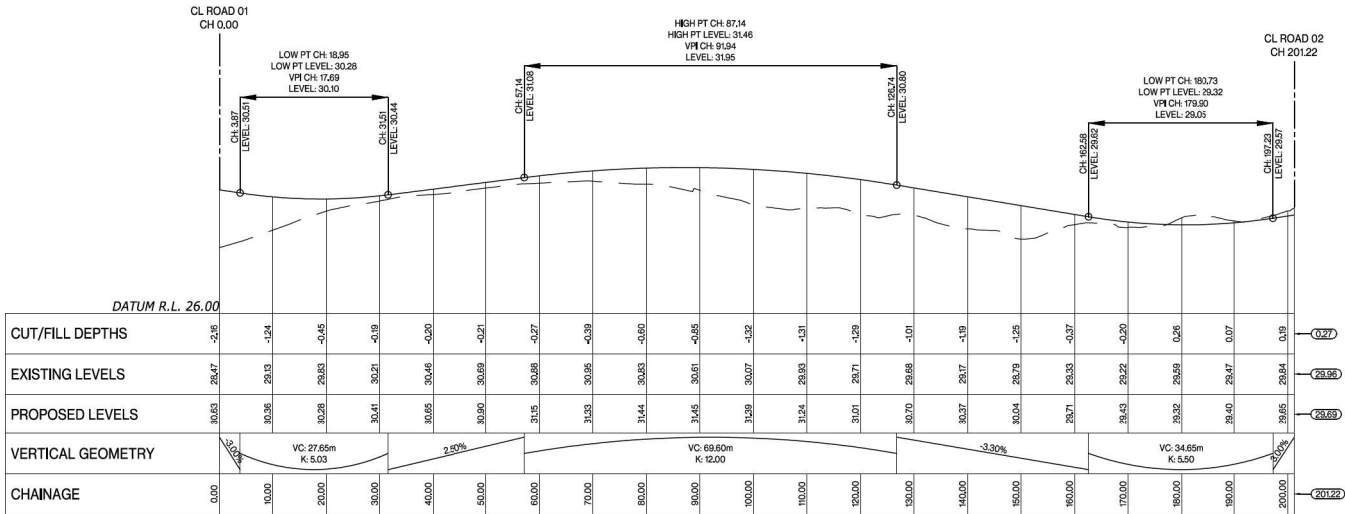
Road 05 LONGSECTION BETWEEN 0.00 AND 201.22
