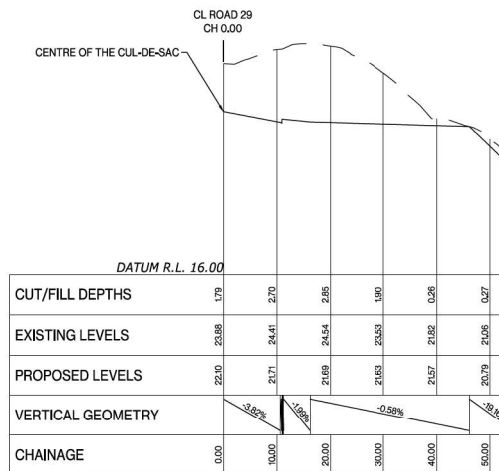
Coal 33 LONGSECTION BETWEEN 0.00 AND 54.59
