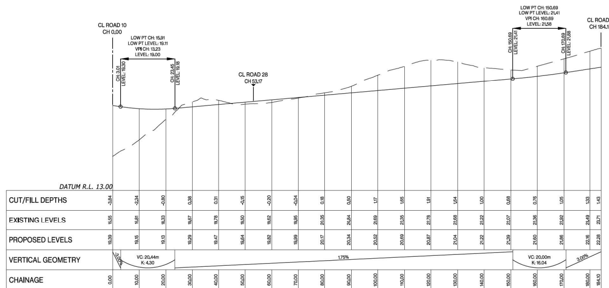
Road 26 LONGSECTION BETWEEN 0.00 AND 184.10
