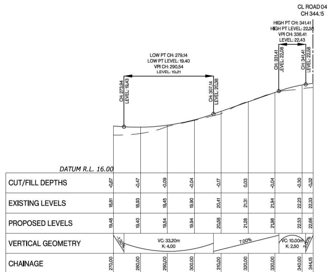
Road 30 LONGSECTION BETWEEN 270.00 AND 344.15
