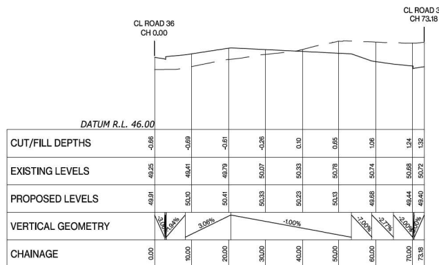
Coal 30 LONGSECTION BETWEEN 0.00 AND 73.18
