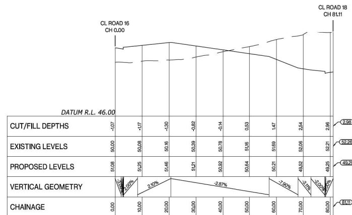
Coal 31 LONGSECTION BETWEEN 0.00 AND 81.11
