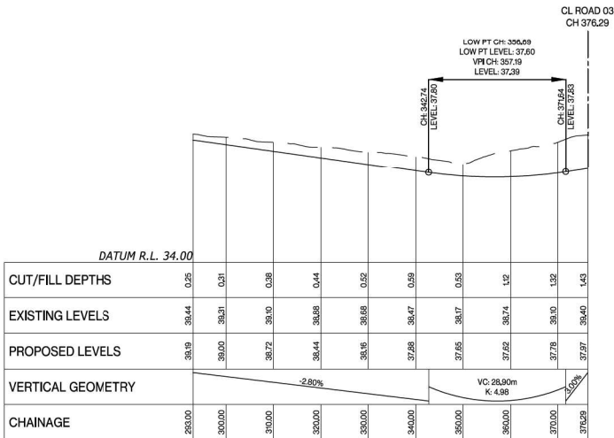
Road 07 LONGSECTION BETWEEN 293.00 AND 376.29
