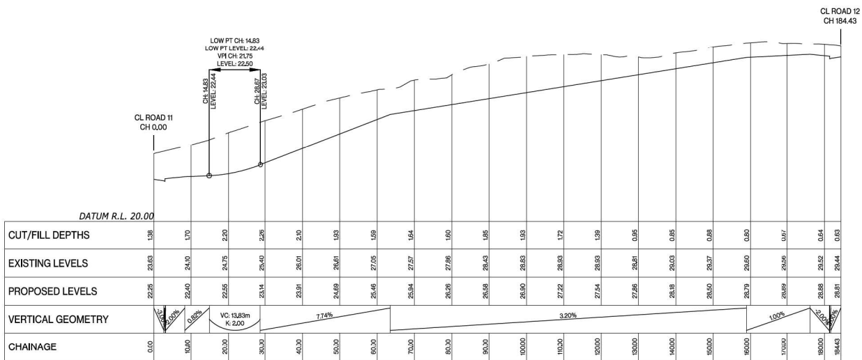
Coal 8 LONGSECTION BETWEEN 0.00 AND 184.43
