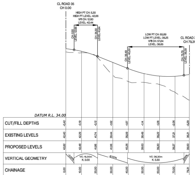
Road 35 LONGSECTION BETWEEN 0.00 AND 79.31
