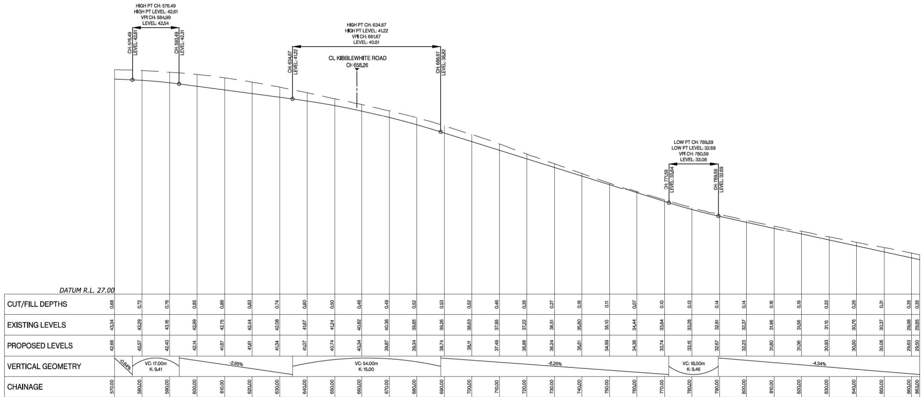
JLD CENTRELINE LONGSECTION BETWEEN 570.00 AND 863.00
