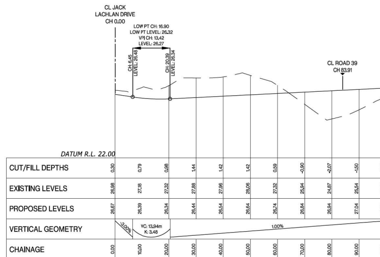
Road 25 LONGSECTION BETWEEN 0.00 AND 99.70
