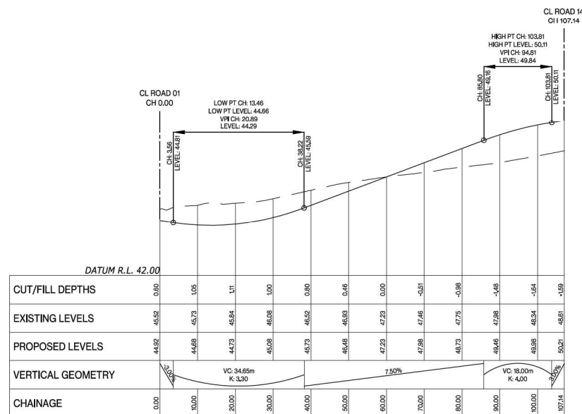
Road 27 LONGSECTION BETWEEN 0.00 AND 107.14
