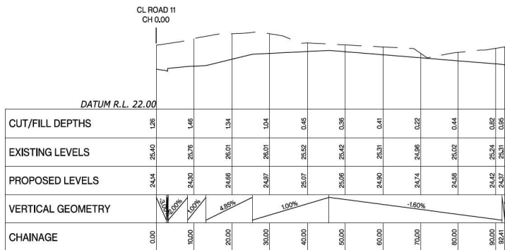
Coal 9 LONGSECTION BETWEEN 0.00 AND 92.41
