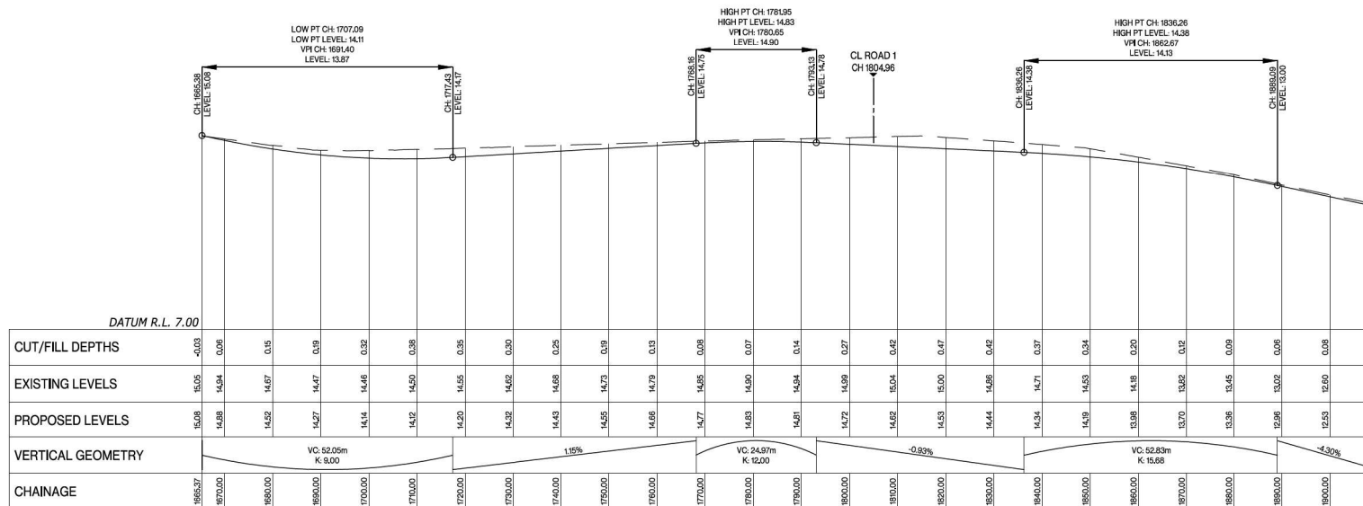
JLD CENTRELINE LONGSECTION BETWEEN 1665.37 AND 1910.00
