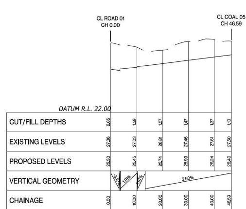
Coal 6 LONGSECTION BETWEEN 0.00 AND 46.59
