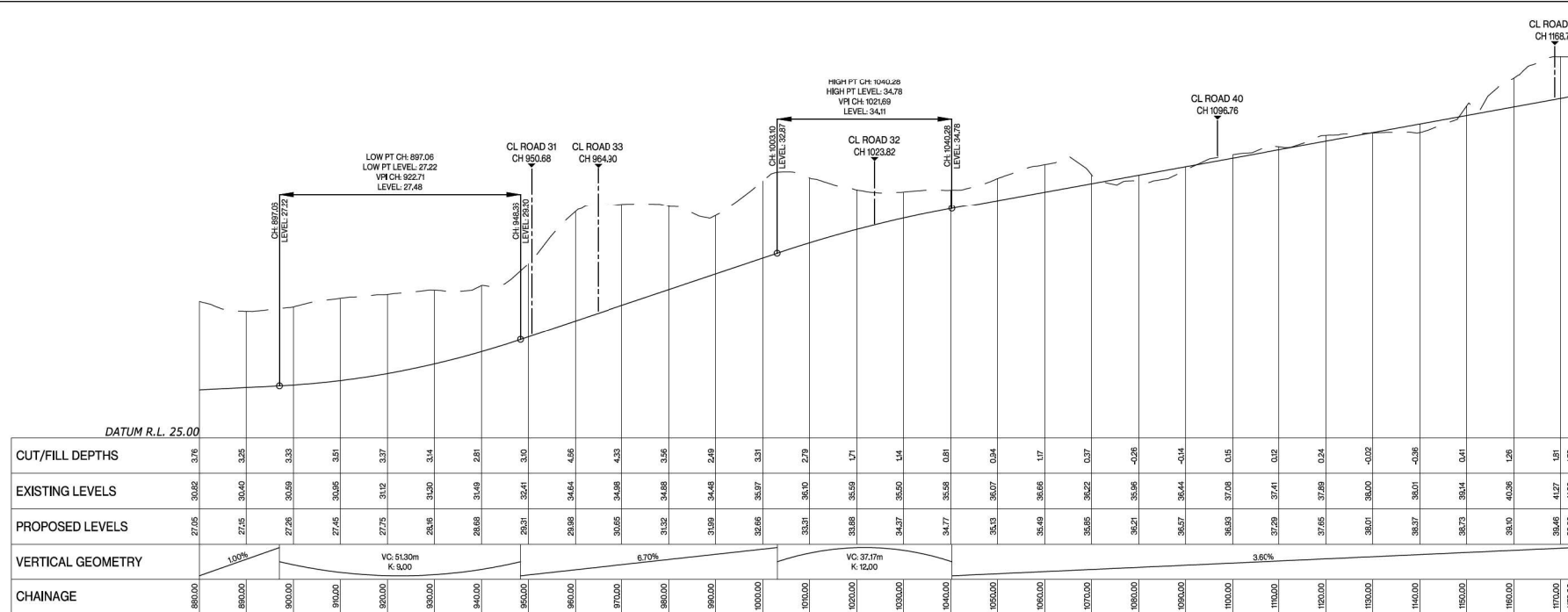
Road 01 LONGSECTION BETWEEN 880.00 AND 1173.00
