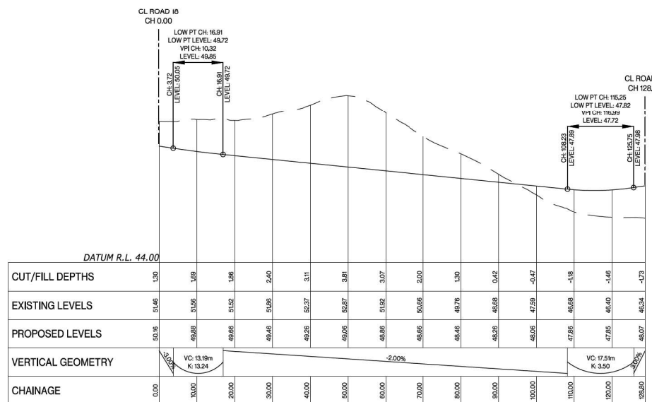
Road 18 LONGSECTION BETWEEN 0.00 AND 128.80
