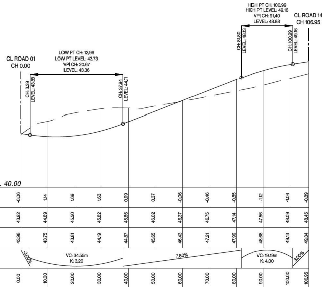
Road 17 LONGSECTION BETWEEN 0.00 AND 106.95
