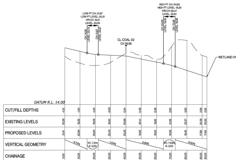
Coal 3 LONGSECTION BETWEEN 0.00 AND 93.00
