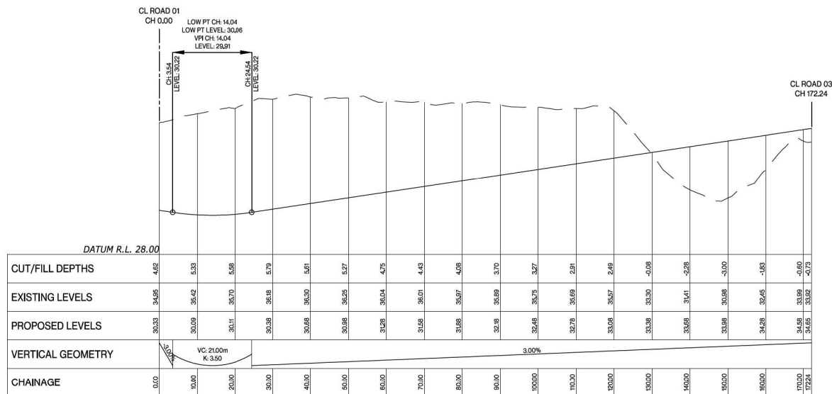
Road 33 LONGSECTION BETWEEN 0.00 AND 172.24
