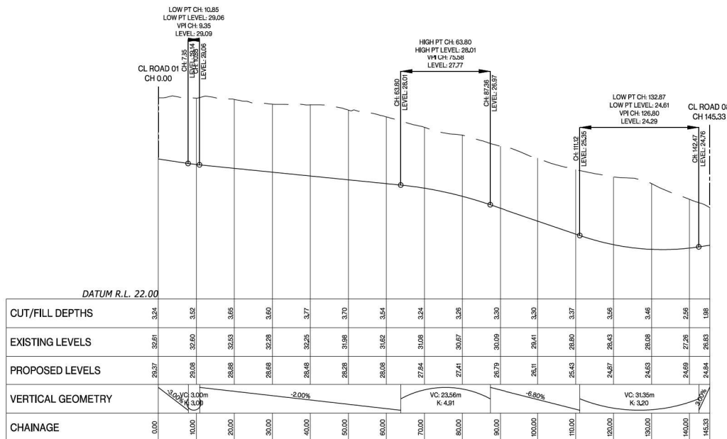
Road 31 LONGSECTION BETWEEN 0.00 AND 145.33
