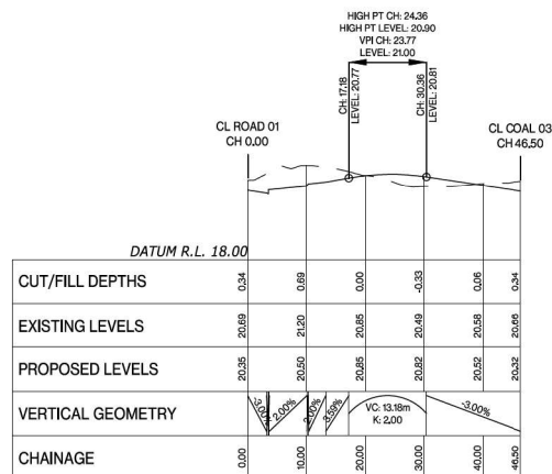
Coal 2 LONGSECTION BETWEEN 0.00 AND 46.50
