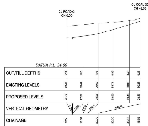
Coal 7 LONGSECTION BETWEEN 0.00 AND 46.79
