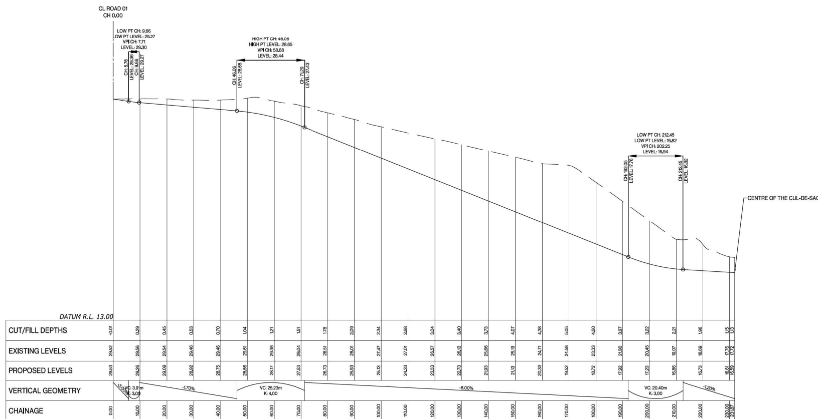
Road 12 LONGSECTION BETWEEN 0.00 AND 231.87
