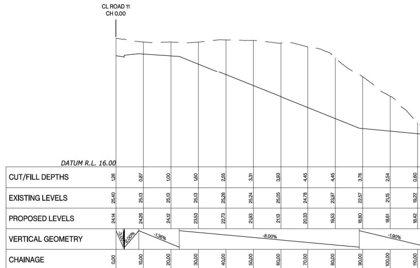
Coal 10 LONGSECTION BETWEEN 0.00 AND 114.03
