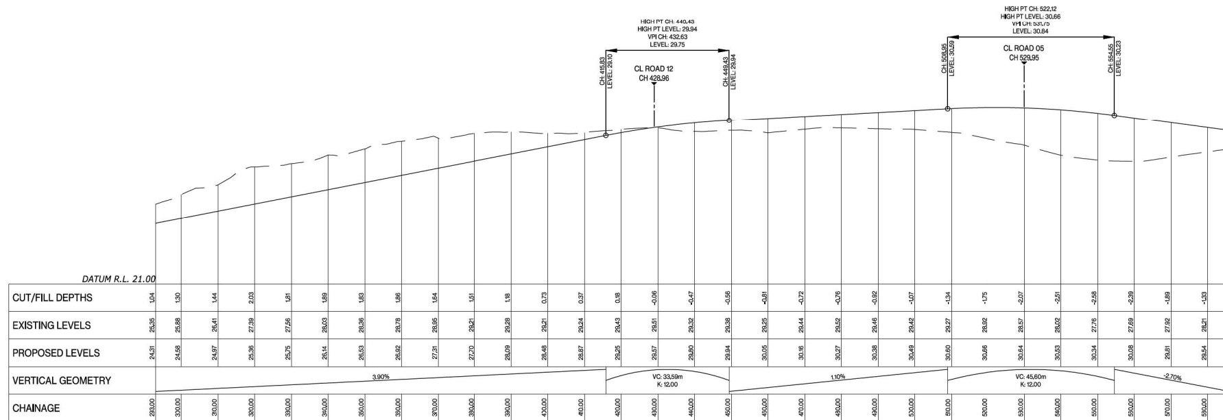
Road 01 LONGSECTION BETWEEN 293.00 AND 586.00
