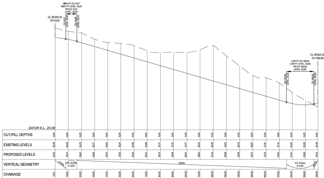
Road 32 LONGSECTION BETWEEN 0.00 AND 199.38
