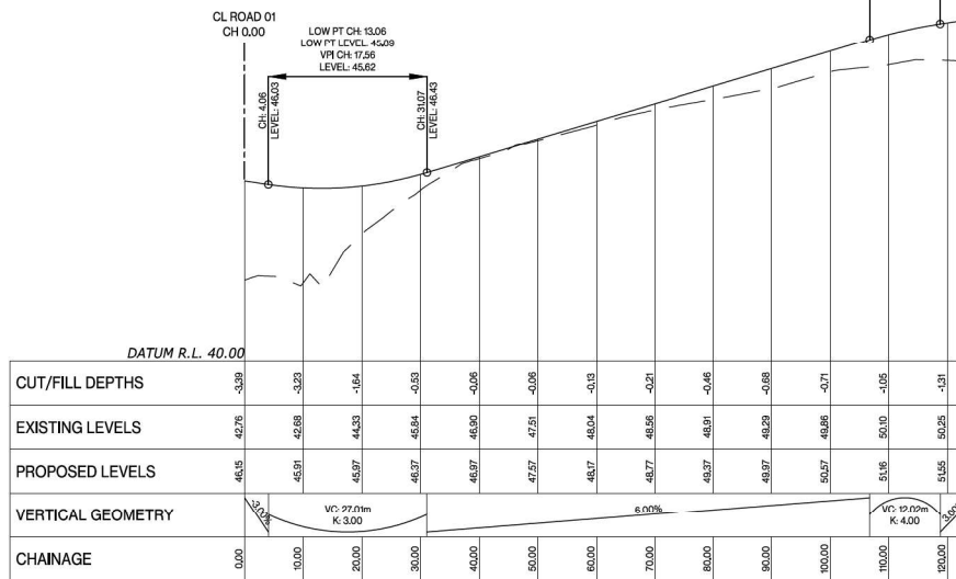
Road 36 LONGSECTION BETWEEN 0.00 AND 124.66
