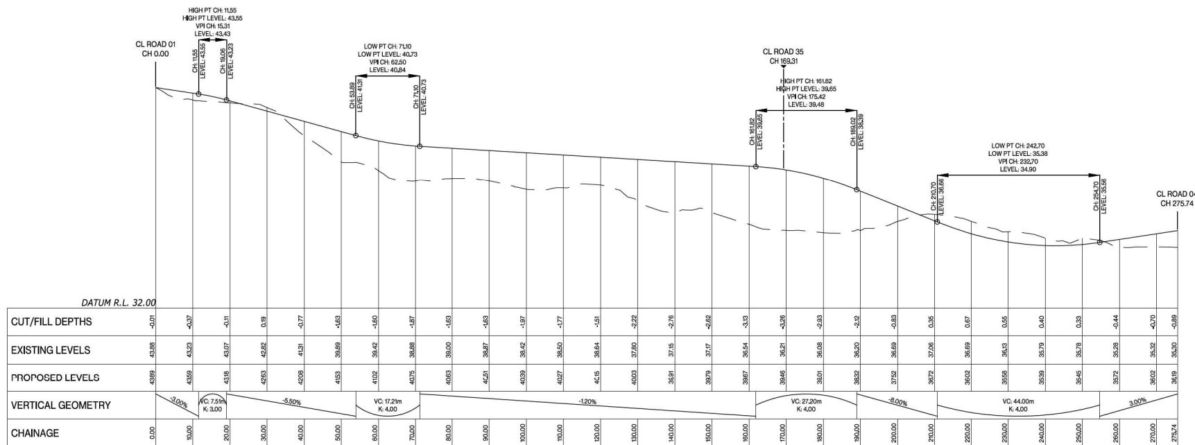
Road 34 LONGSECTION BETWEEN 0.00 AND 275.74
