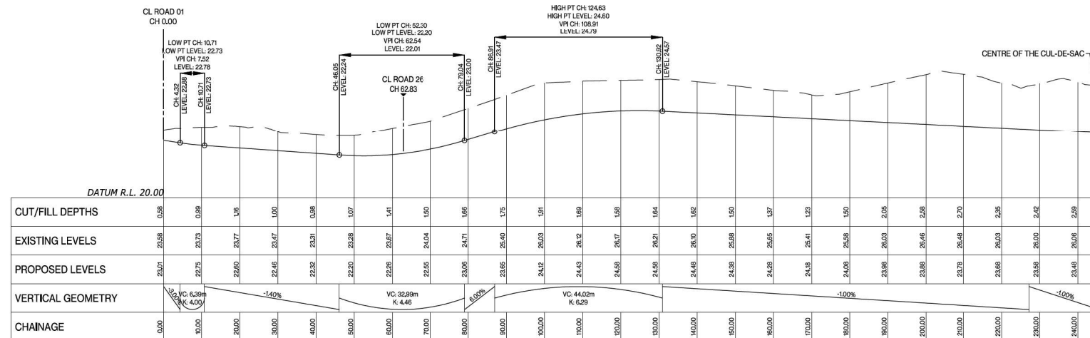
Road 11 LONGSECTION BETWEEN 0.00 AND 245.62
