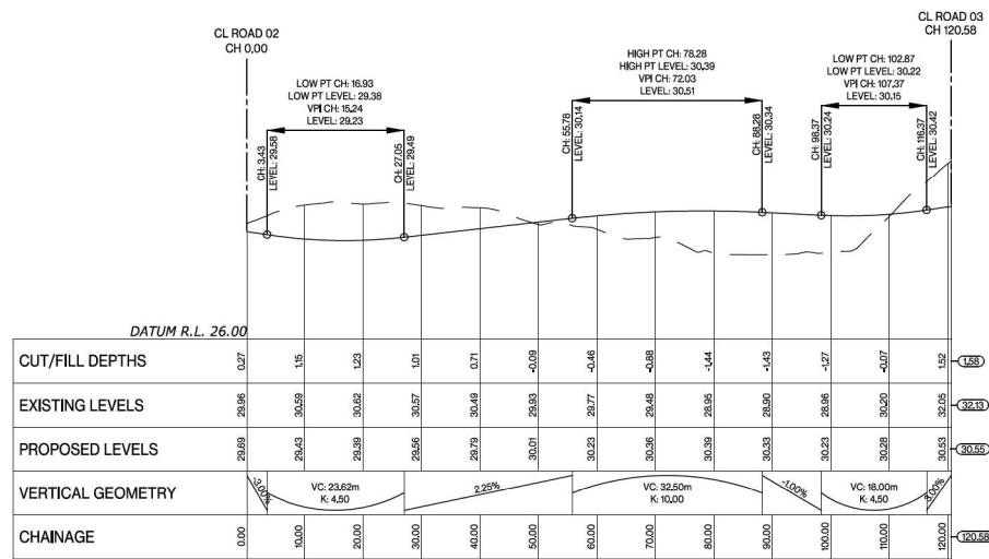
Road 06 LONGSECTION BETWEEN 0.00 AND 120.58
