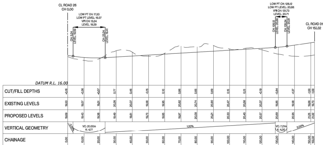
Road 28 LONGSECTION BETWEEN 0.00 AND 152.32
