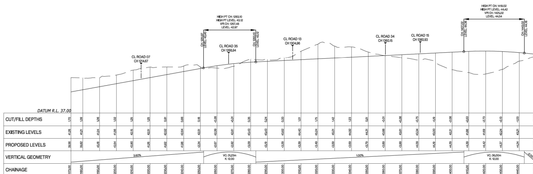
Road 01 LONGSECTION BETWEEN 1173.00 AND 1450.00
