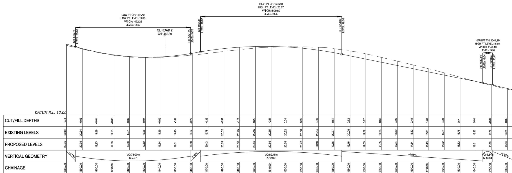
JLD CENTRELINE LONGSECTION BETWEEN 1380.00 AND 1665.37
