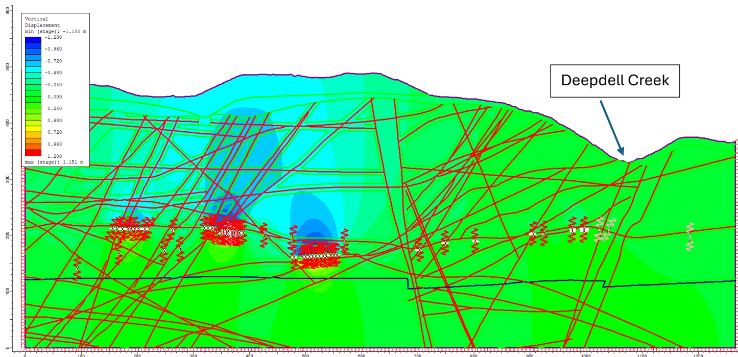
Figure 1: Section B –Vertical Displacement
