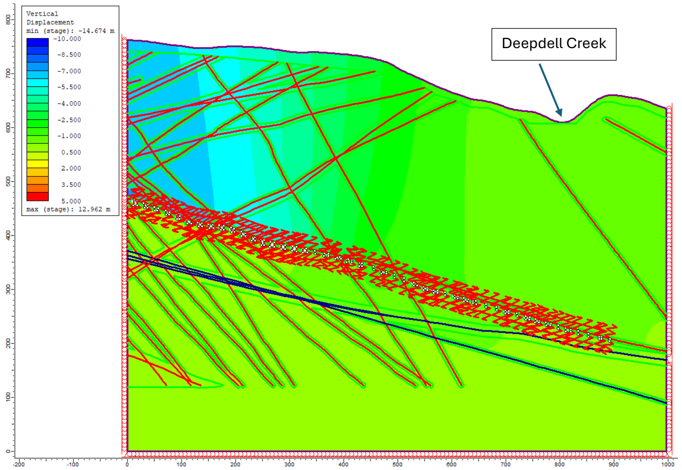
Figure 3: Section E Vertical Displacement
