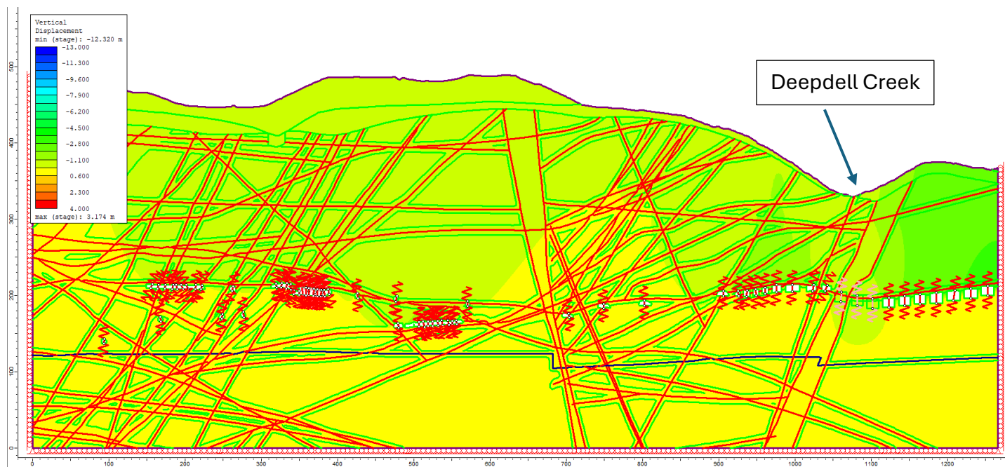
Figure 2: Section B (with artificial openings under the Deepdell Creek)– Vertical Displacement
