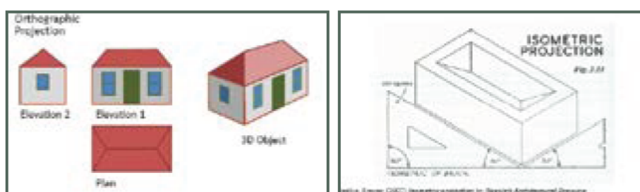
Fig. 7. Examples of two dimensional drawing method (Wesley Maguire IMG006 and IMG007).
