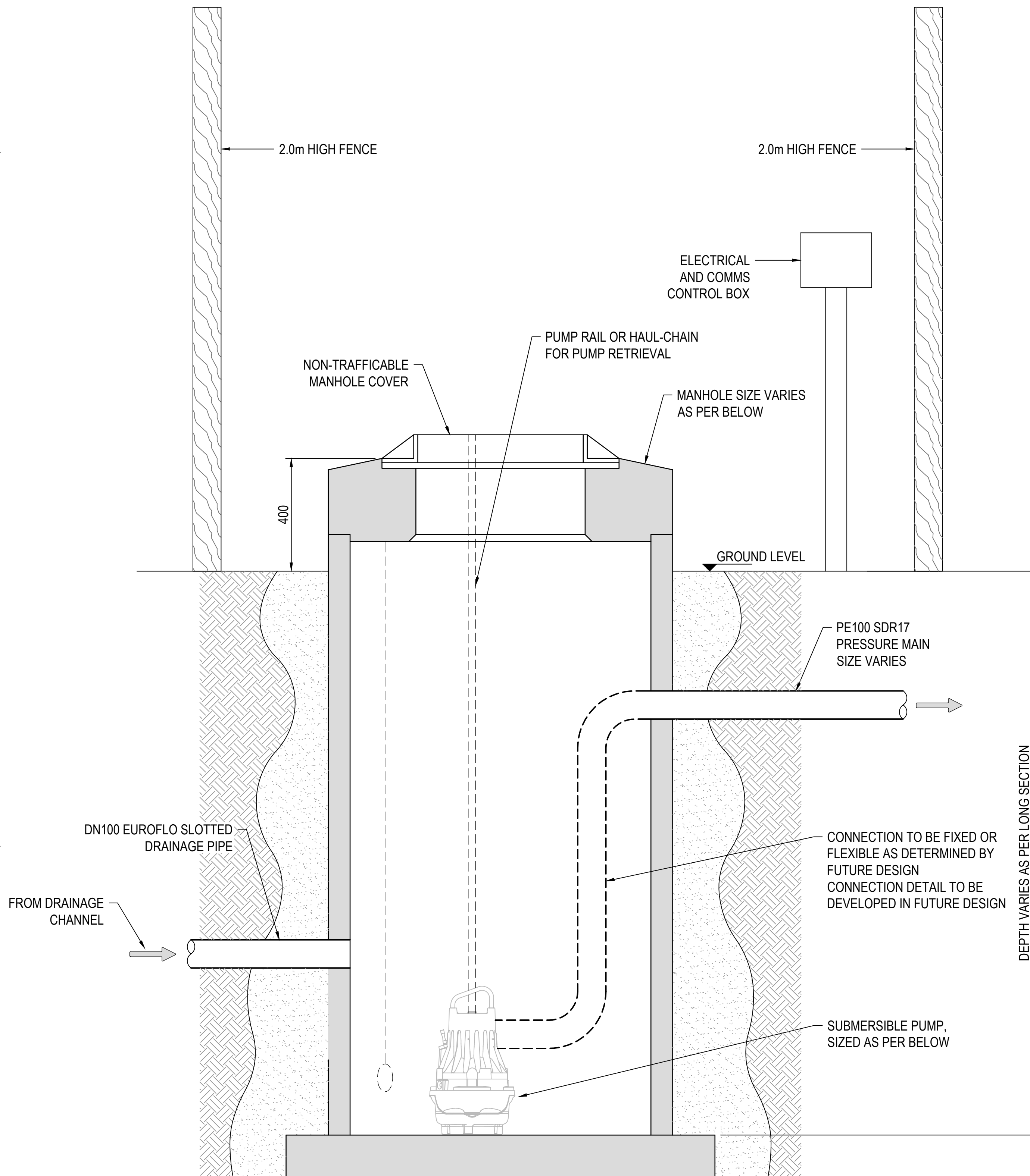
TYPICAL MANHOLE DETAIL NOT TO SCALE
