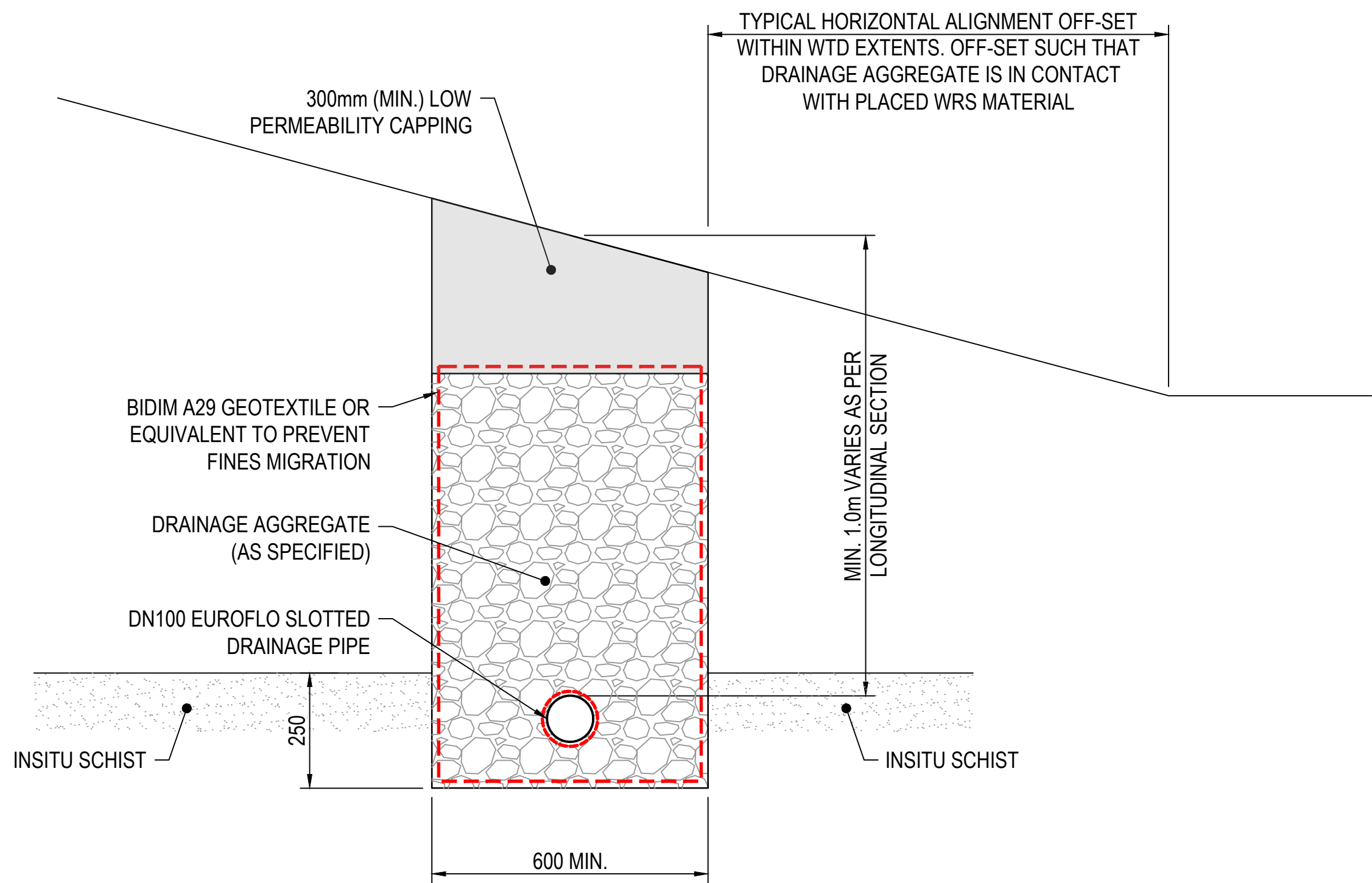
TYPICAL ENGINEERING DRAINAGE CHANNEL CROSS-SECTION NOT TO SCALE
