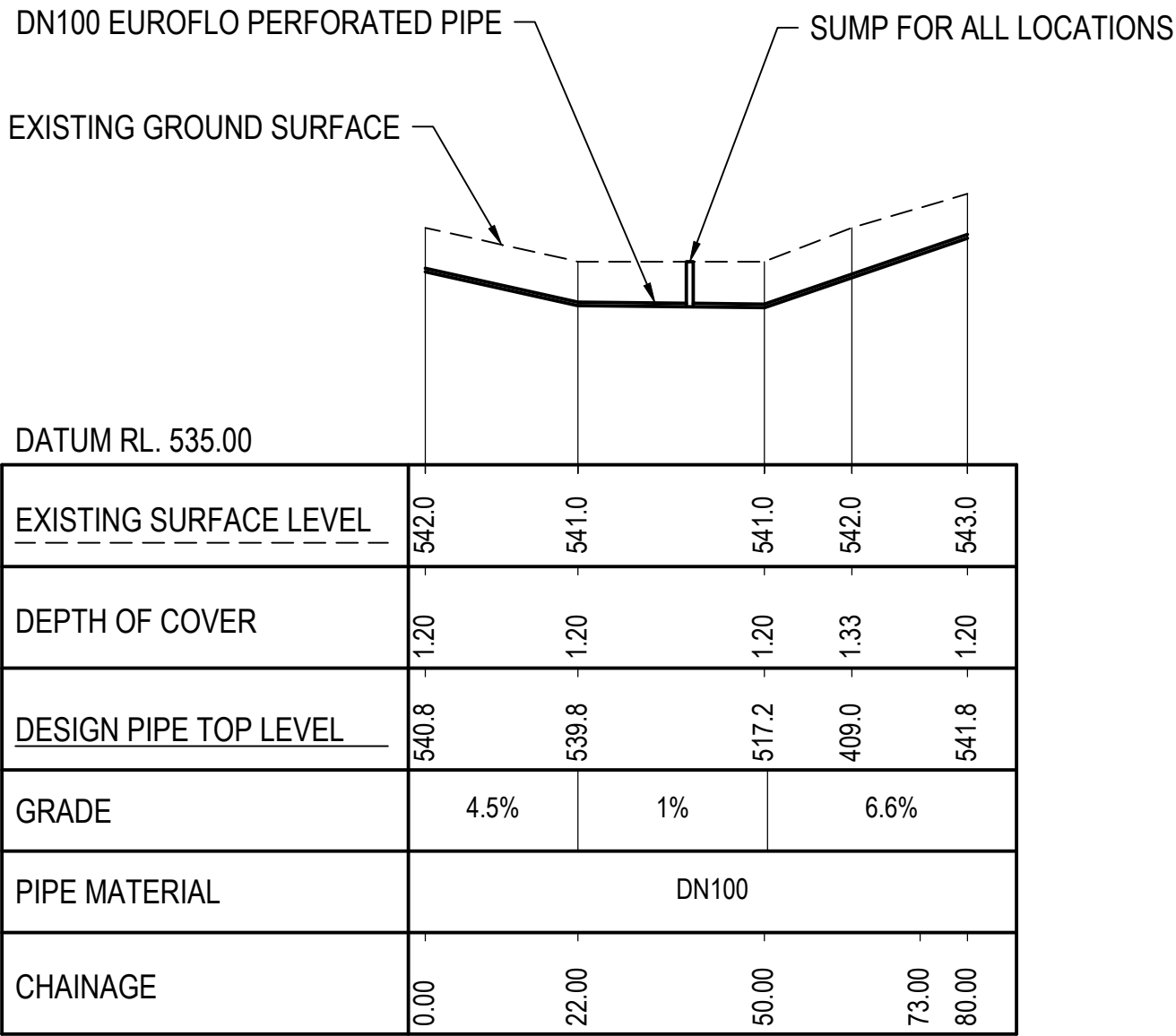
LONG SECTION CORONATION NORTH DRAIN - 4 SCALE 1:1000
