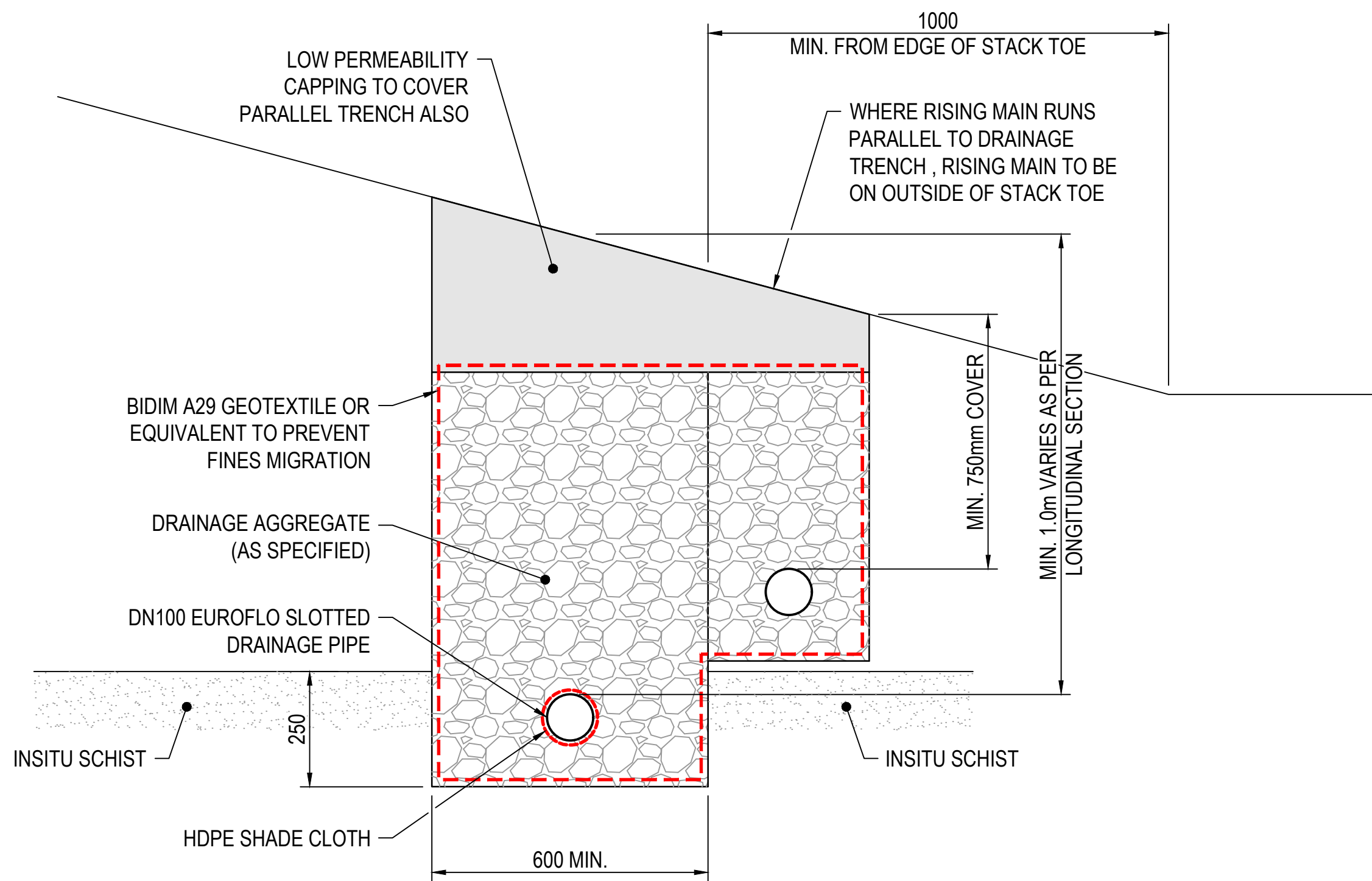
TYPICAL DUAL PIPELINE CROSS-SECTION NOT TO SCALE
