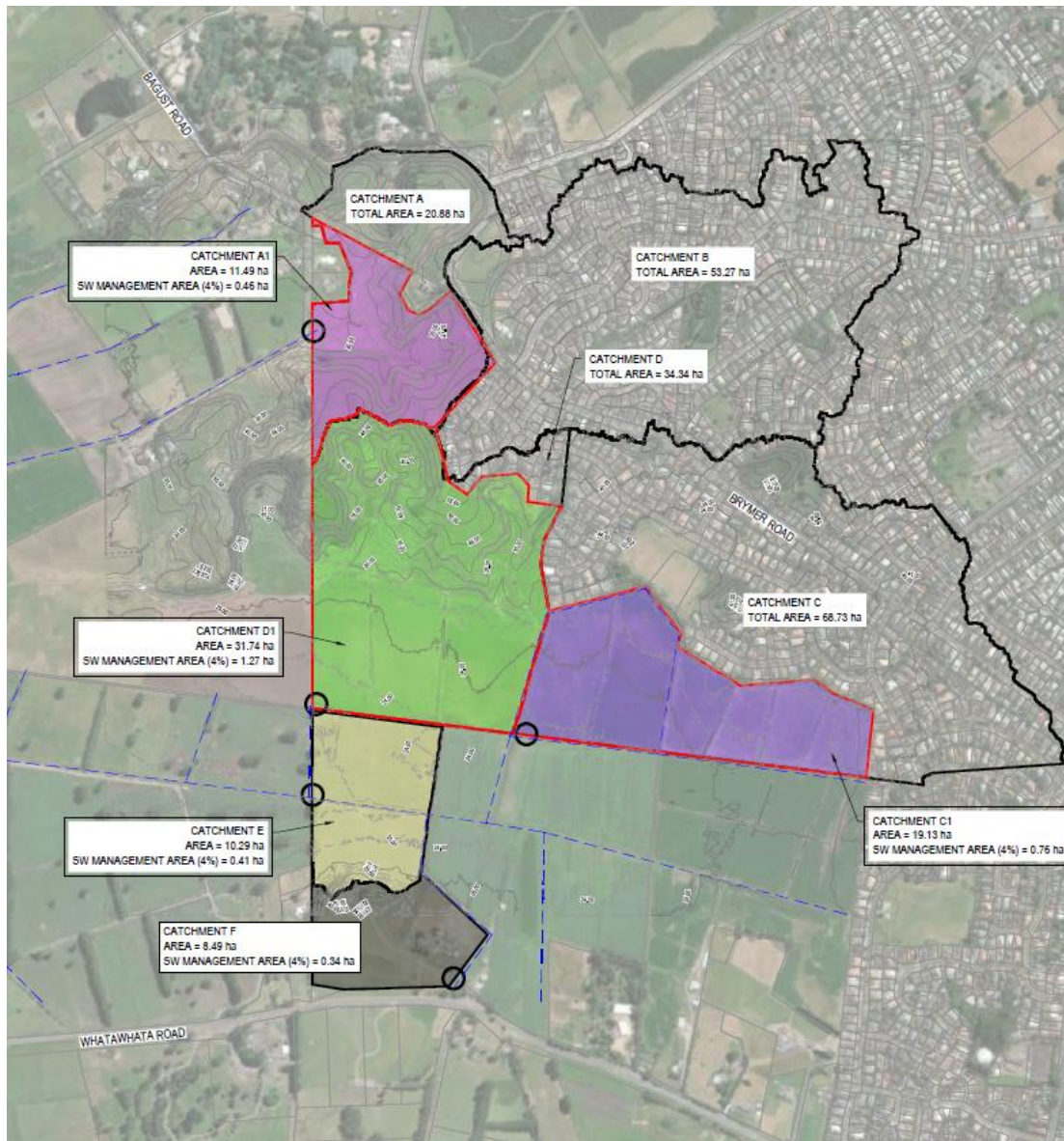
Image 3-Stormwater Catchment Summary
