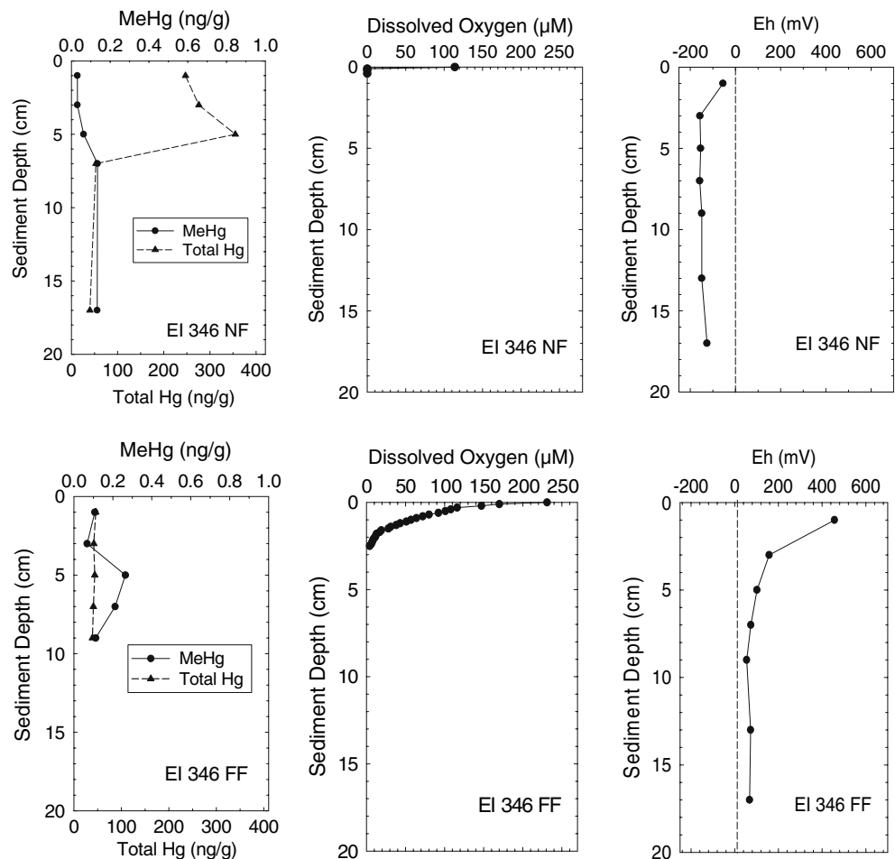
Fig. 6 Vertical profiles for concentrations of total Hg, methylmercury ( MeHg ), dissolved oxygen and Eh for NF and FF sediment cores from site EI346 on the shelf
