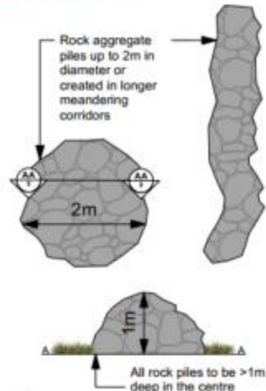
Piles to comprise of washed river rocks 50–200mm grade to provide optimal interstitial spaces amongst the piles for lizard occupation. Rocks will be sourced from a landscape supplier or local quarry prior to lizard release.
