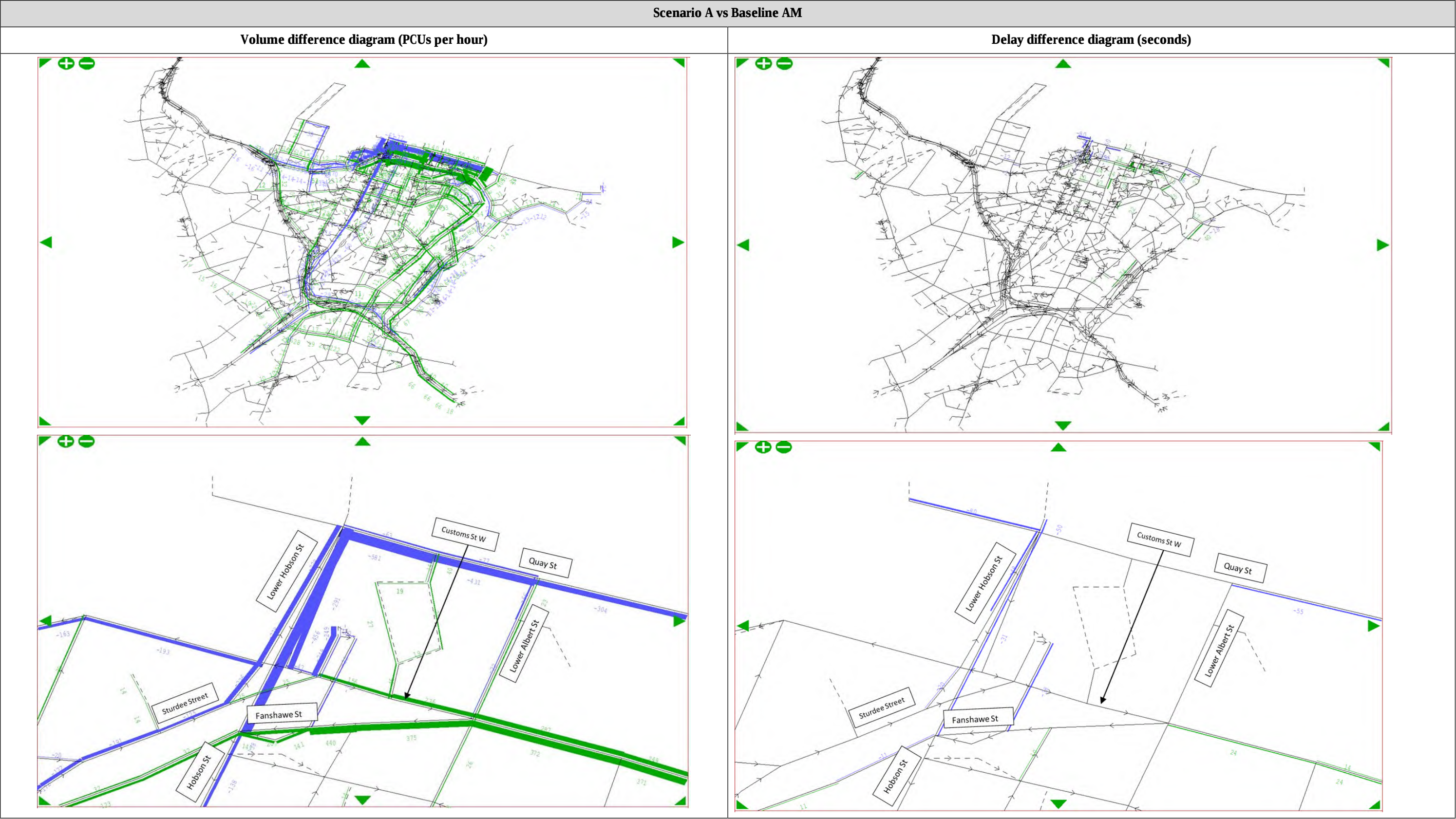
SATURN model volume (in Passenger Car Units / PCUs per hour) and delay difference (in seconds) diagrams between the baseline scenario and demolition scenarios
