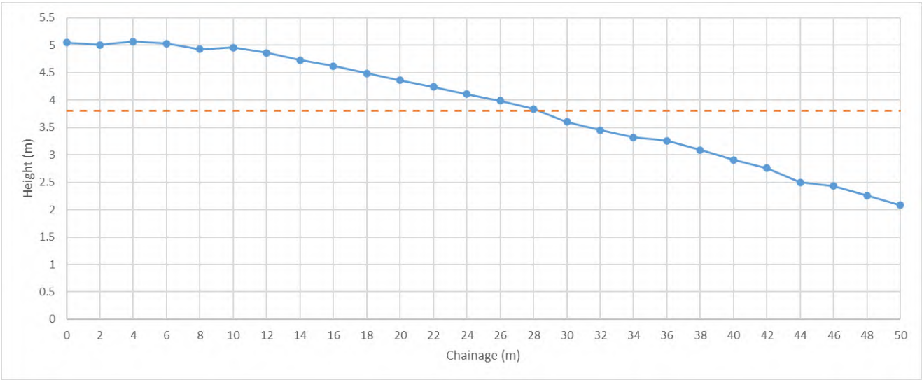
Figure 5: Vertical clearance of Lower Hobson Street Flyover
