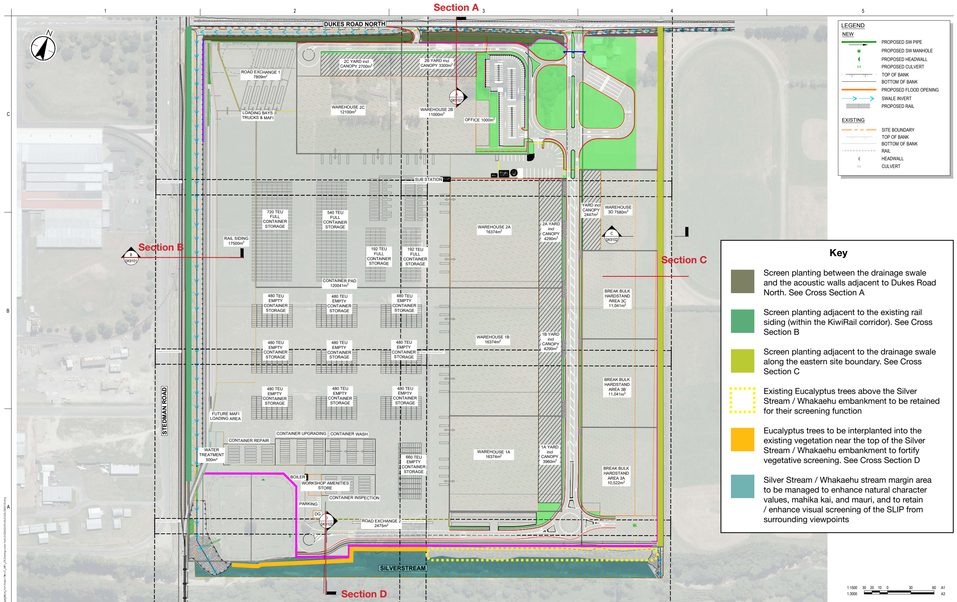
Figure 12: Proposed Southern Link Inland Port – Landscape Concept Plan
