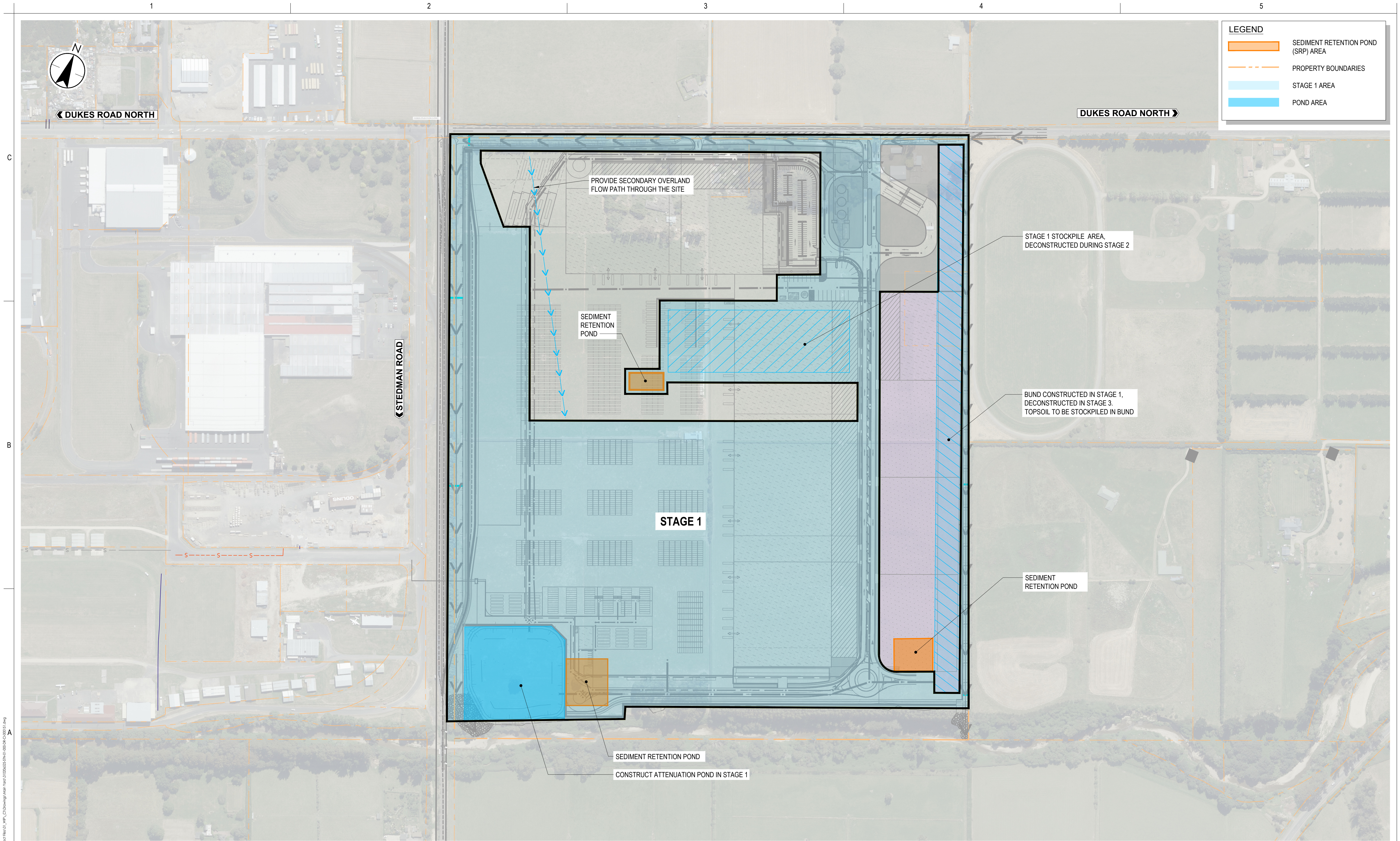
STAGE 1 PLAN SCALE - 1:2,000
