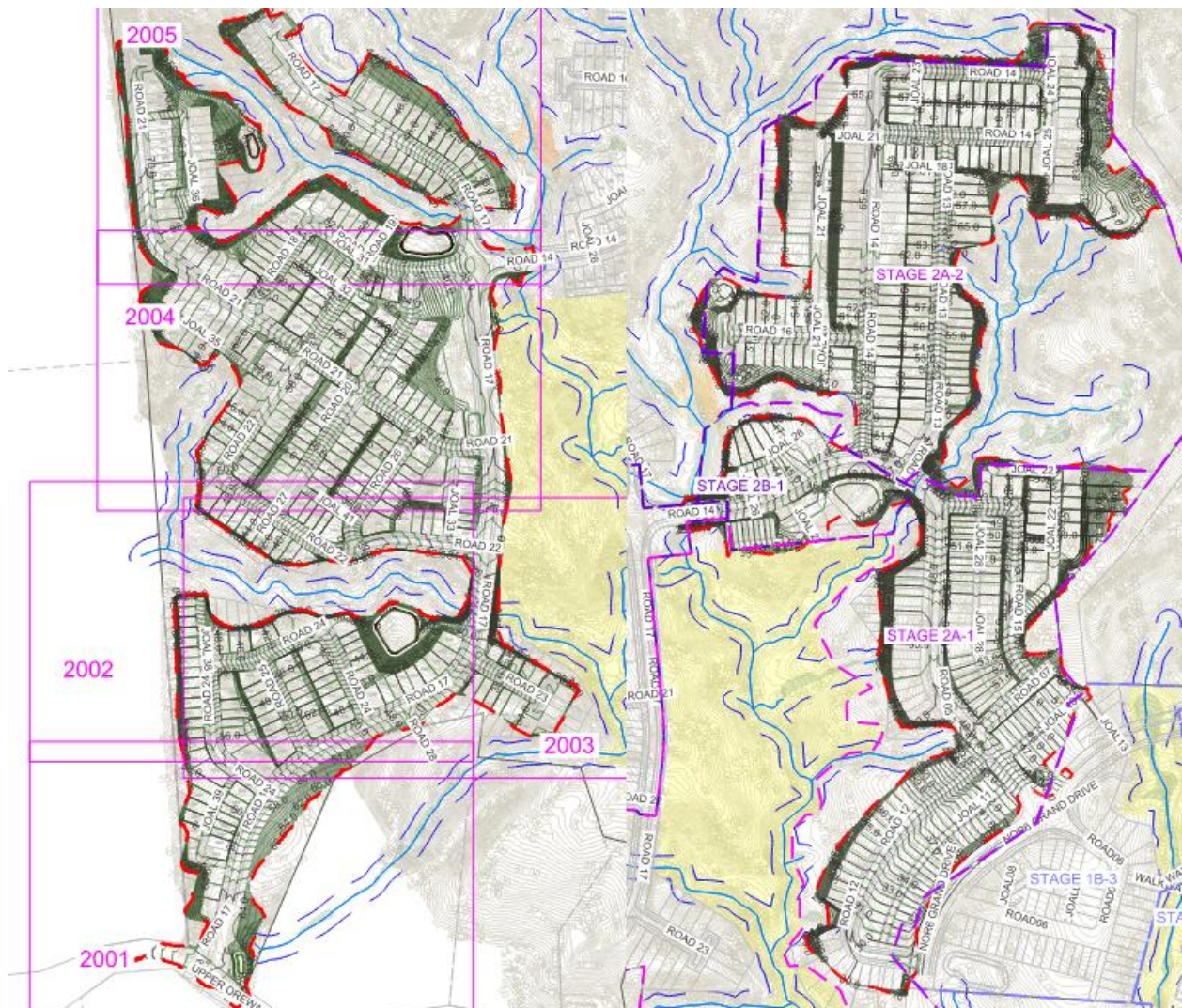
Figure 5 - Stage 2 Earthworks Contour plan
