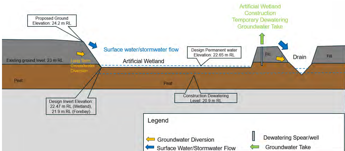
Figure 20: Wetland D Schematic (Not Drawn to Scale)
