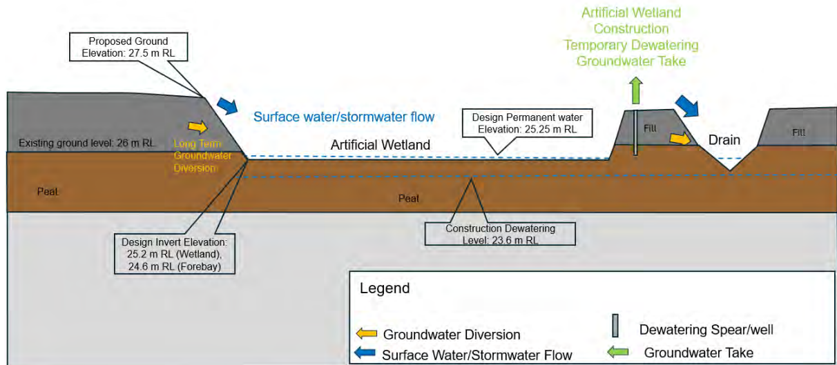
Figure 19: Wetland C Schematic (Not Drawn to Scale)
