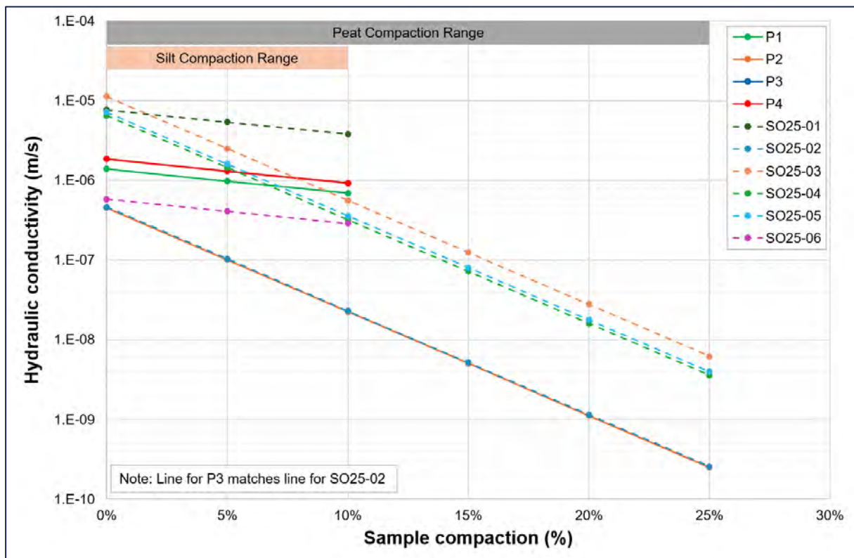
Figure 14: Hydraulic Conductivity Change to Field Test Analysis Results
