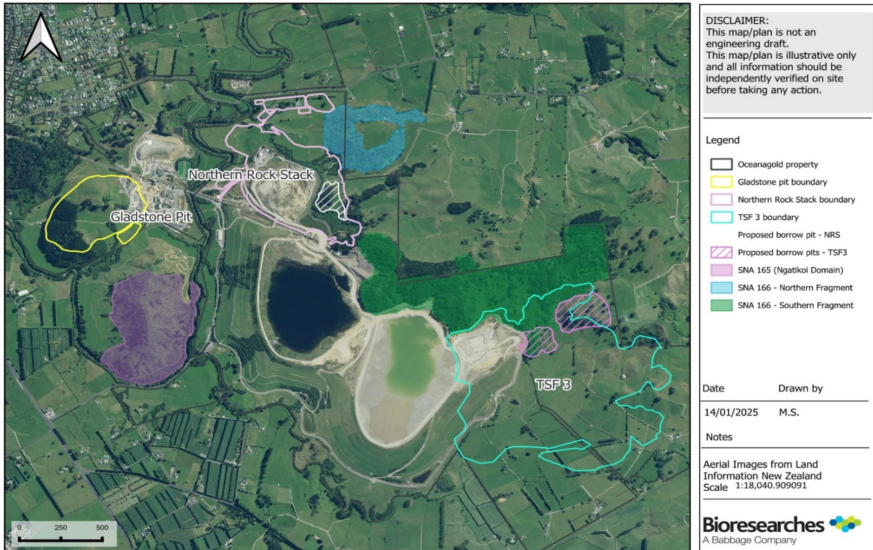
Figure 3: WNP components; GOP, NRS and TSF 3, including proposed borrow pit sites and SNA habitats
