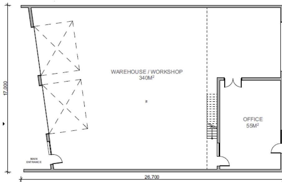
Typical Unit Plan WL_4 scale 1:200
