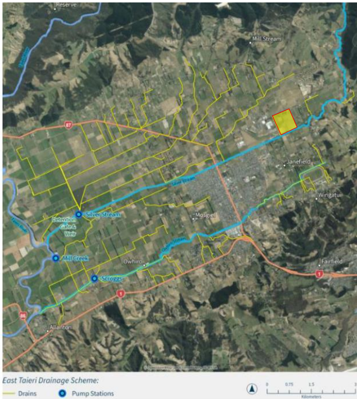
Figure 1: Extent of East Taieri Drainage Scheme
