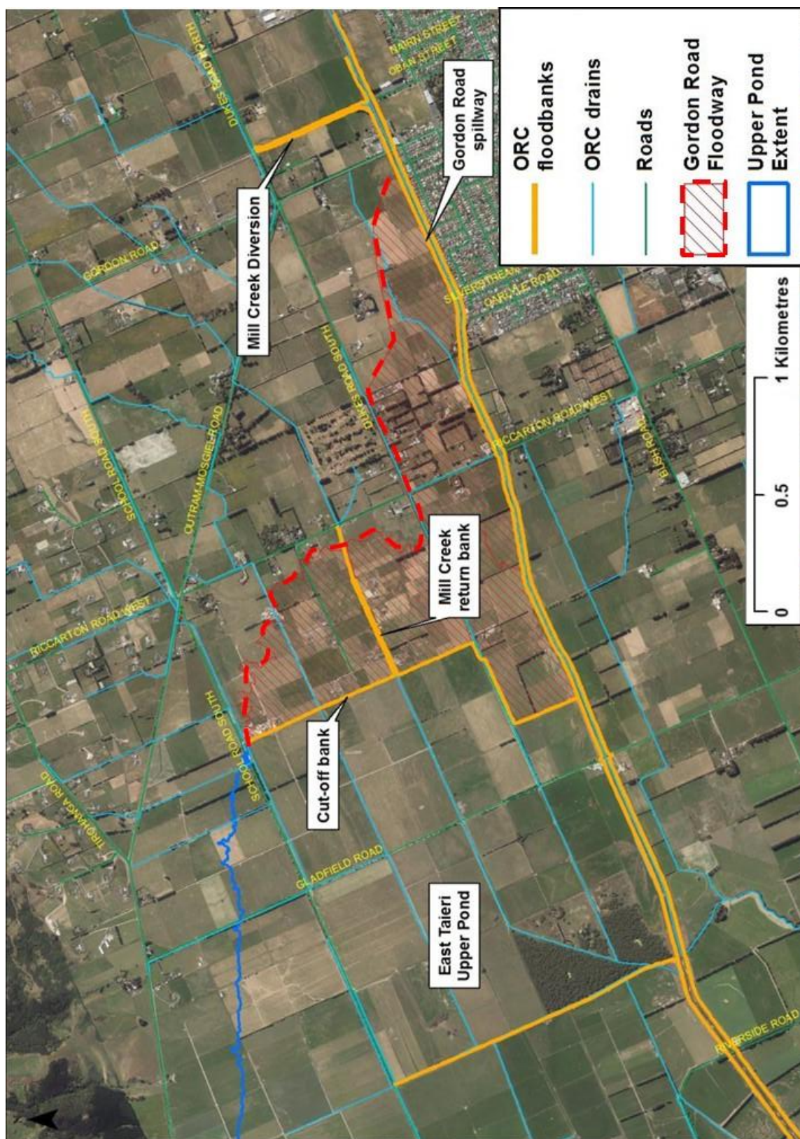
Figure 3: Gordon Road Spillway and Floodway
