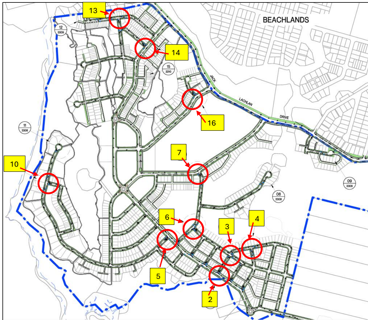
Figure 7-26: Overview of Internal Priority or Stop-Controlled Intersections
