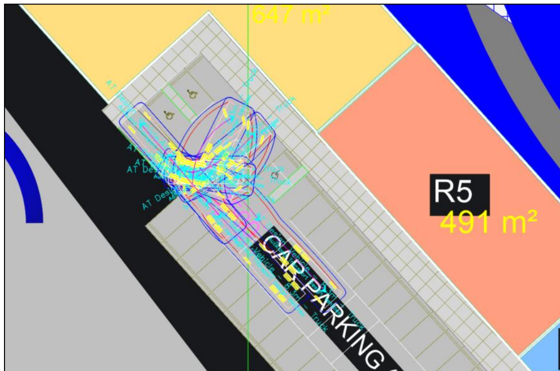
Figure 7-71: Super lot VC2 – loading space tracking
