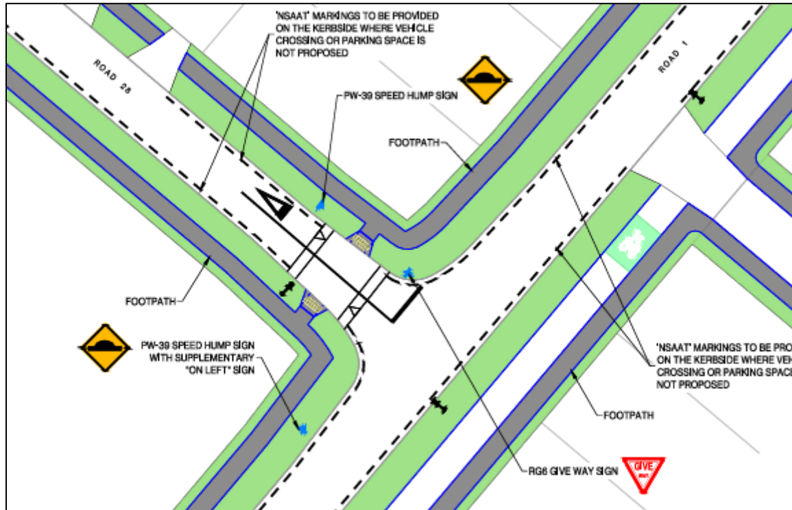
Figure 7-35: Intersection 14
