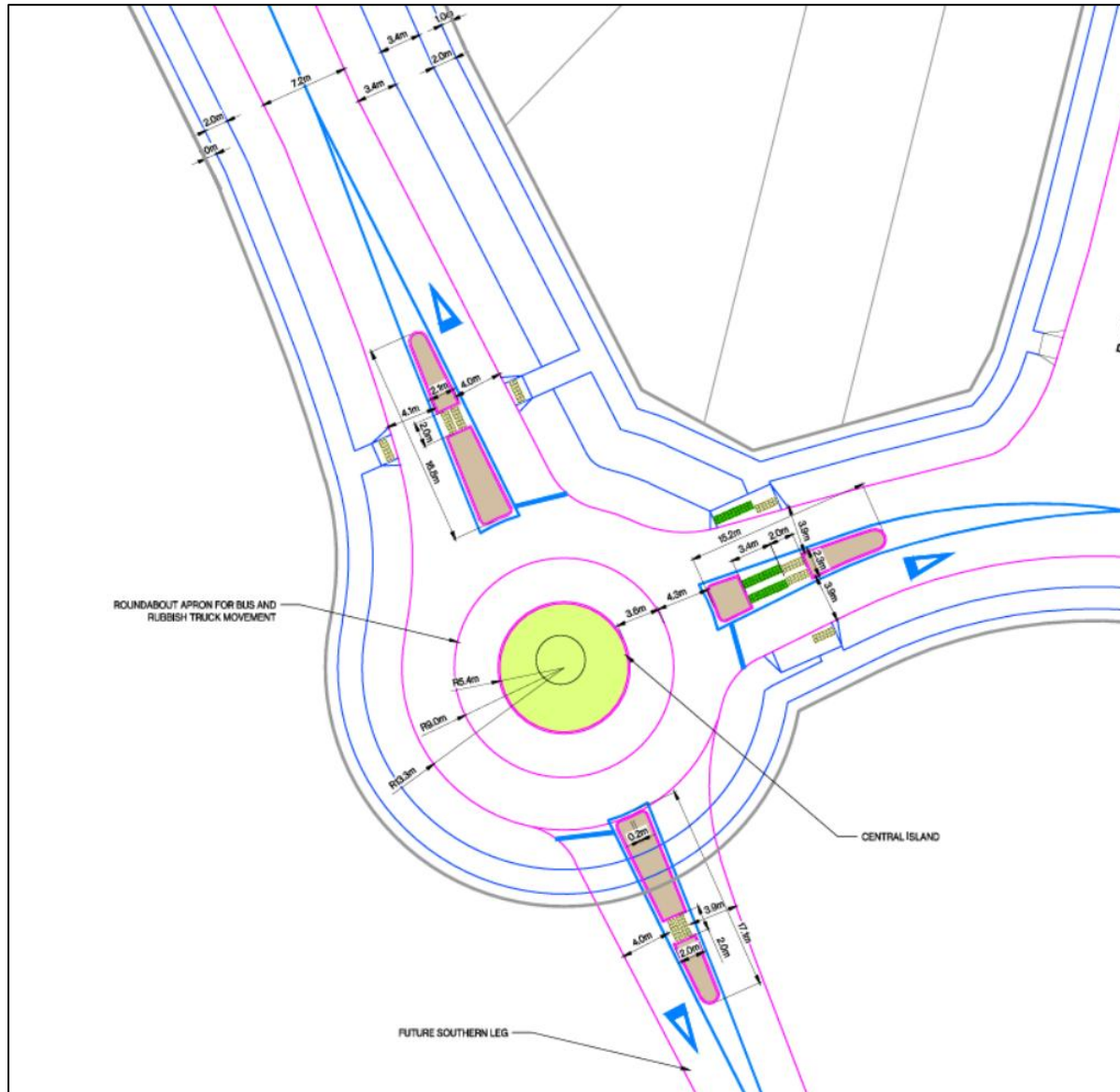
Figure 7-40: Roundabout at Road 1 / Road 20
