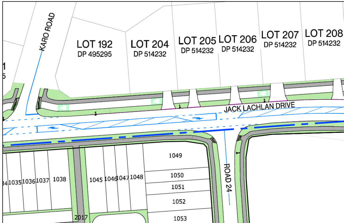
Updated Figure 7-24: Road 24 Industrial Local / Jack Lachlan Drive Intersection
