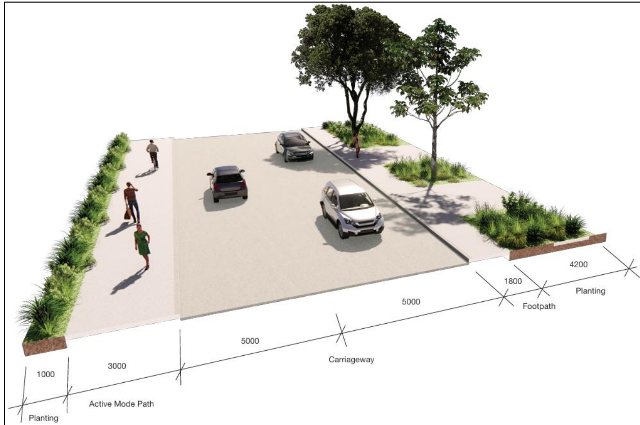
Figure 7-18: Proposed Typical Jack Lachlan Drive corridor Cross Section (Segment C boat houses)
