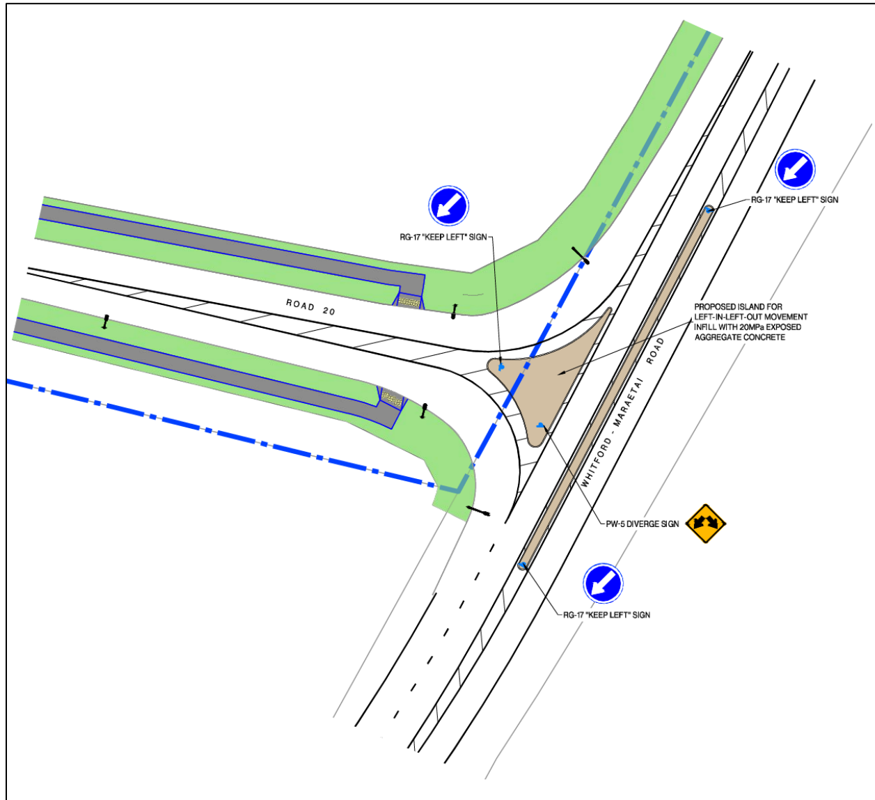
Updated Figure 7-25: Road 20 / Whitford-Maraetai Road Intersection Showing Solid Median
