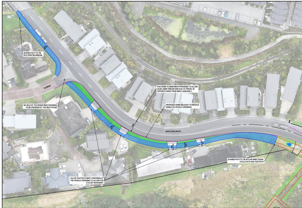
Figure 7-18b: Proposed Typical Jack Lachlan Drive Corridor Concept Design (Segment C boat houses)
