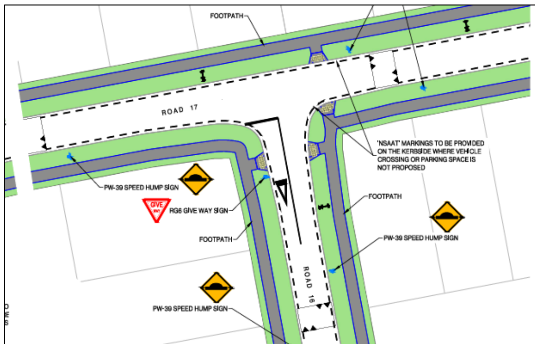
Figure 7-29: Intersection 4
