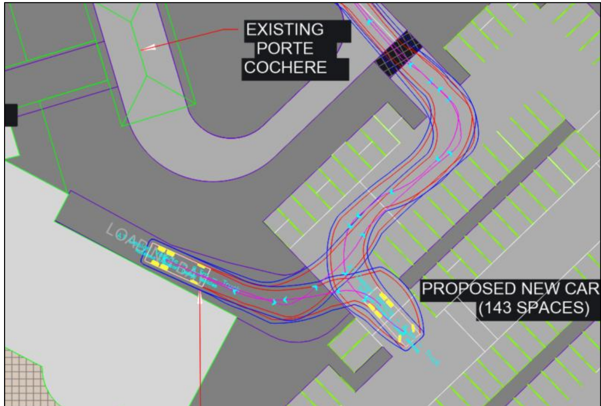
Figure 7-66: Super lot CM5 – loading space tracking (ground floor)
