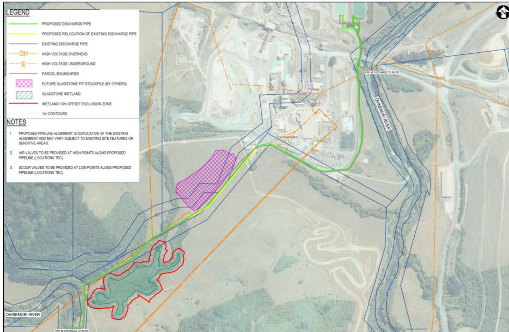
Figure 2-54: Proposed Alignment of the Pipelines for the Additional Discharge Outfalls
