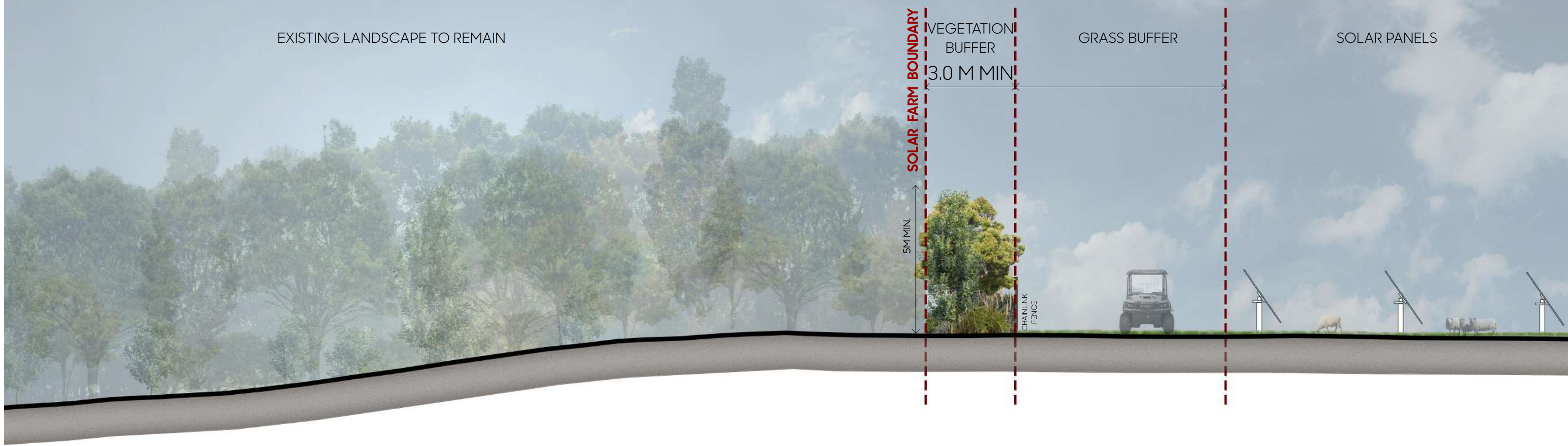
SECTION A-A 1:125@A1 / 1:250@A3 NOTE: VEGETATION SHOWN AS INDICATIVE OF 5-7 YEAR MATURITY
