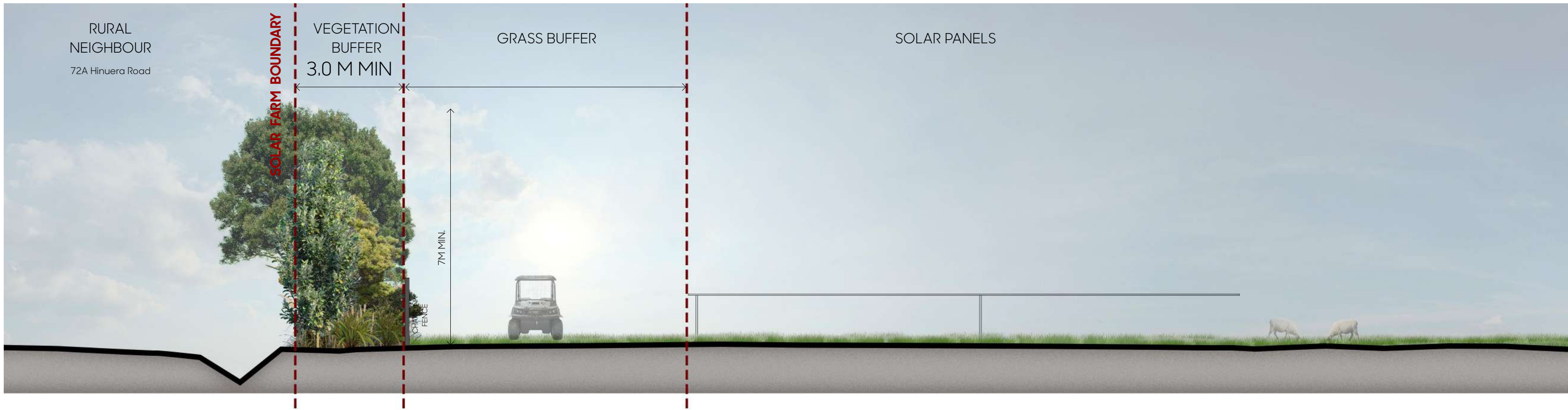
SECTION B-B 1:100@A1 / 1:200@A3 NOTE: VEGETATION SHOWN AS INDICATIVE OF 5-7 YEAR MATURITY
