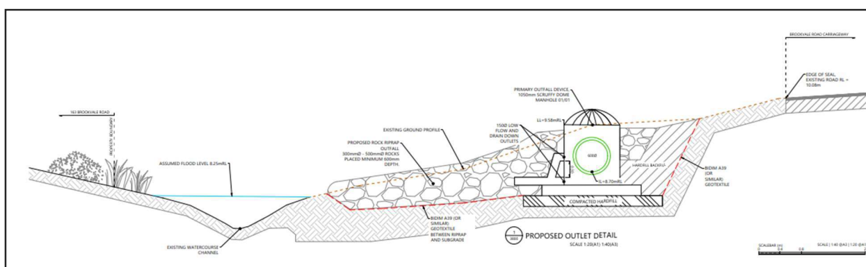
Figure 18: outlet structure details
