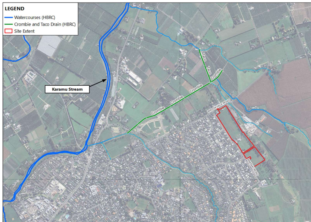
Figure 7: Catchment drainage
