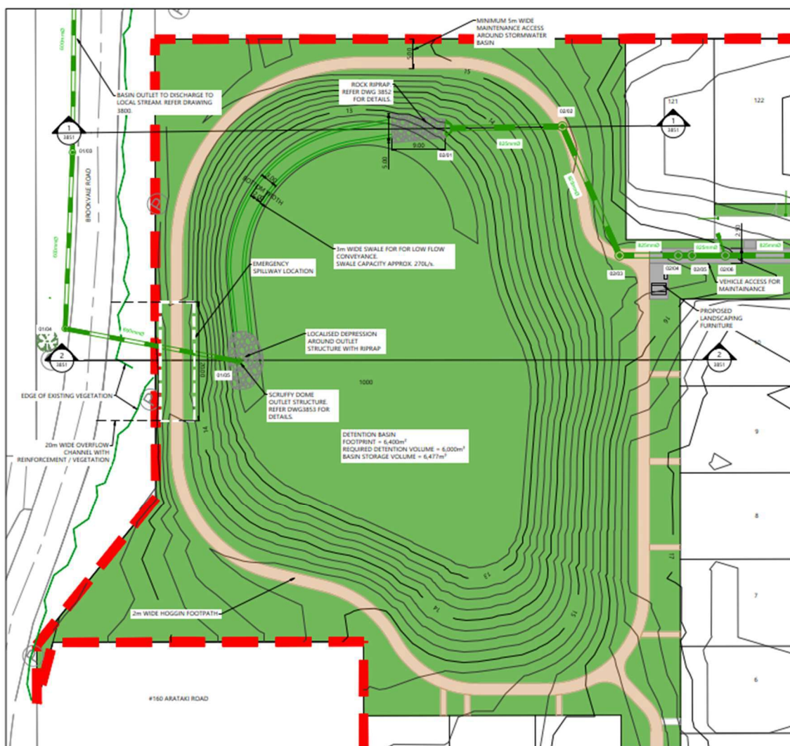
Figure 10: Pond layout
