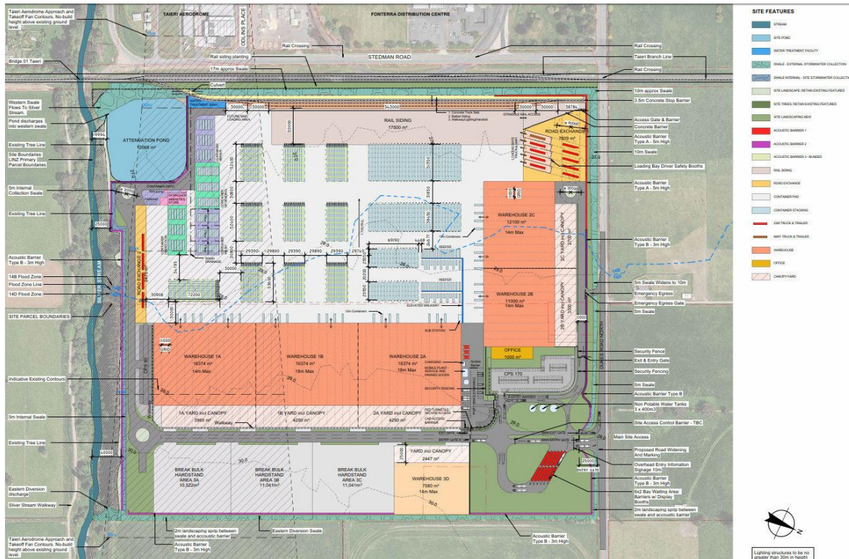
Figure 3: Concept plan of the proposed development (Williams Architects Limited, Master Plan Concept 9.2, dated 13 April 2026).
