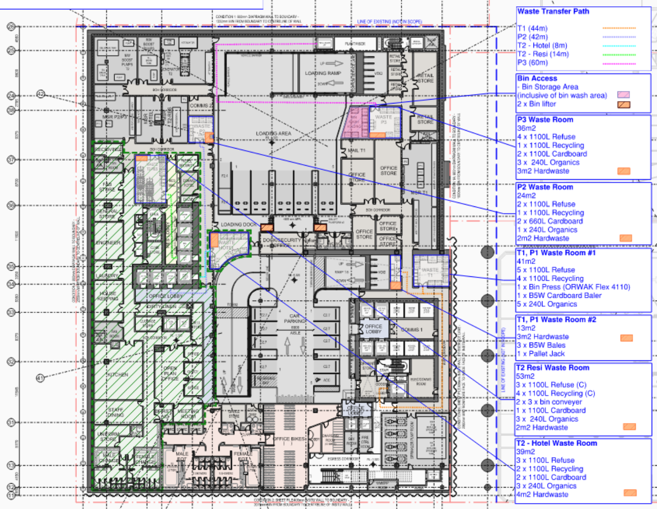
Figure 3-2: Scaled waste room sketch
