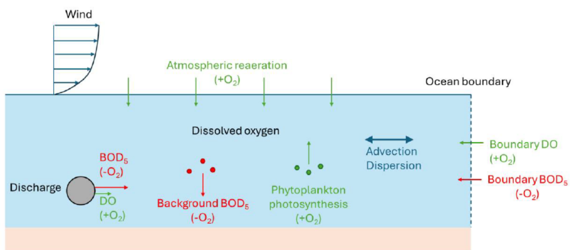
Figure 5.1: DO processes
