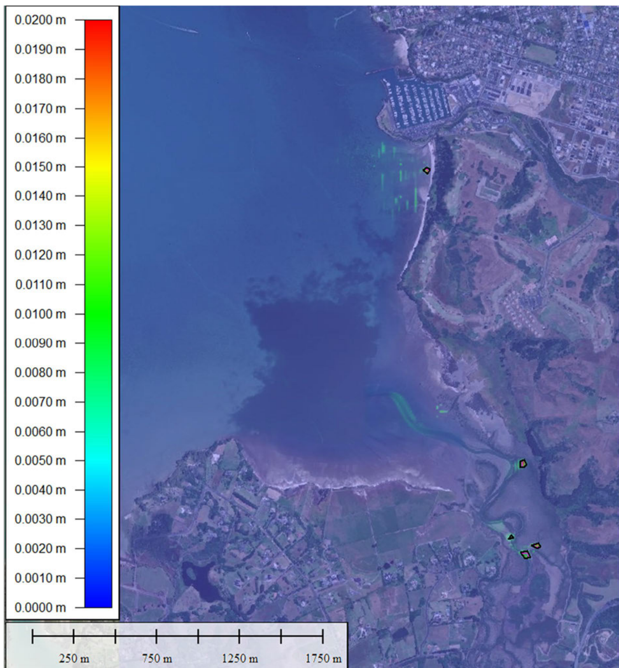
Figure 10-24 10 ARI TSS assuming Spring tide, ET peak discharge
