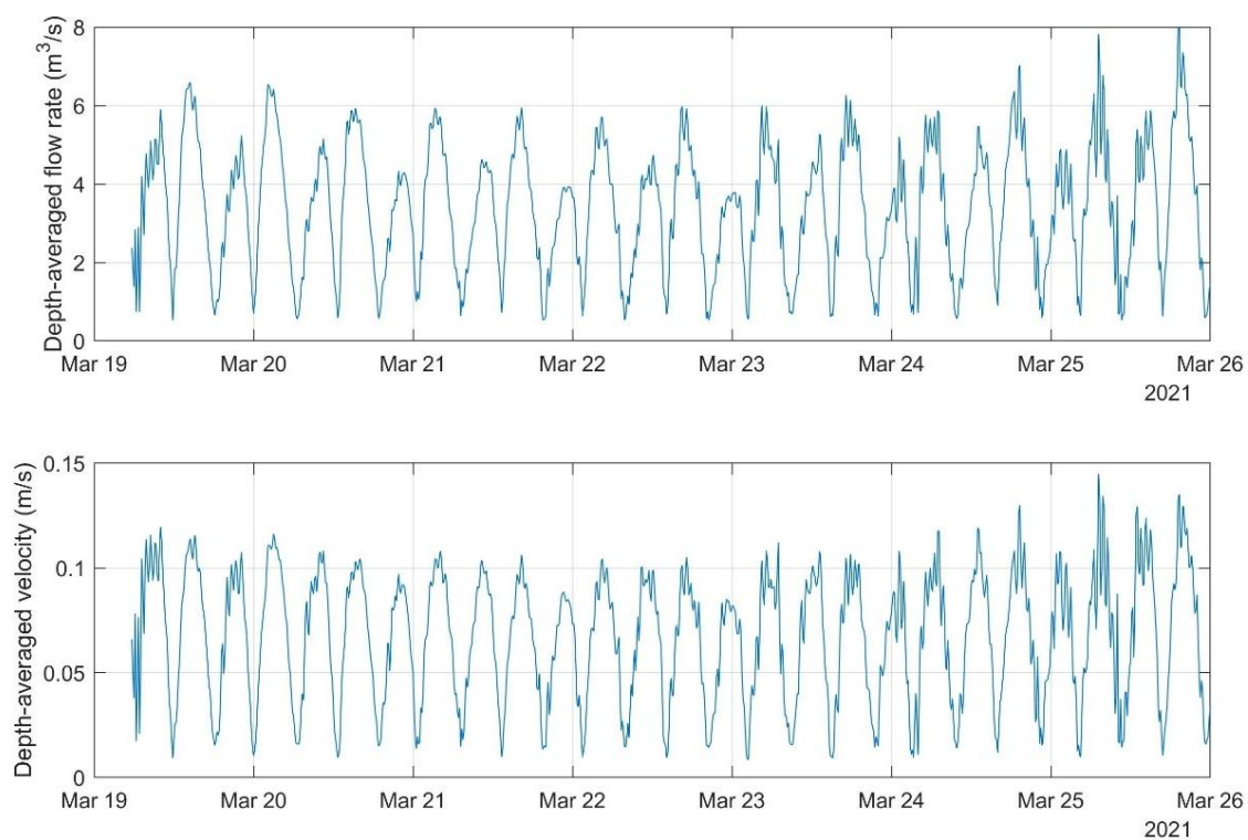
Figure 4.1: Depth-averaged flowrate and velocity at the discharge location using the baseline hydrodynamic model. The minimum flowrate is 0.53 \text{ m}^3/\text{s} , which is much higher than the discharge flowrate of 0.046 \text{ m}^3/\text{s} .
