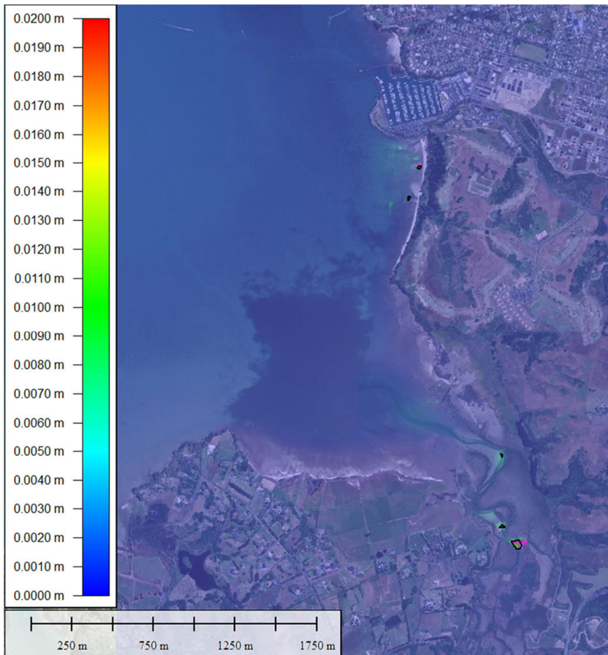
Figure 10-27 10 ARI TSS assuming Neap tide, FT peak discharge
