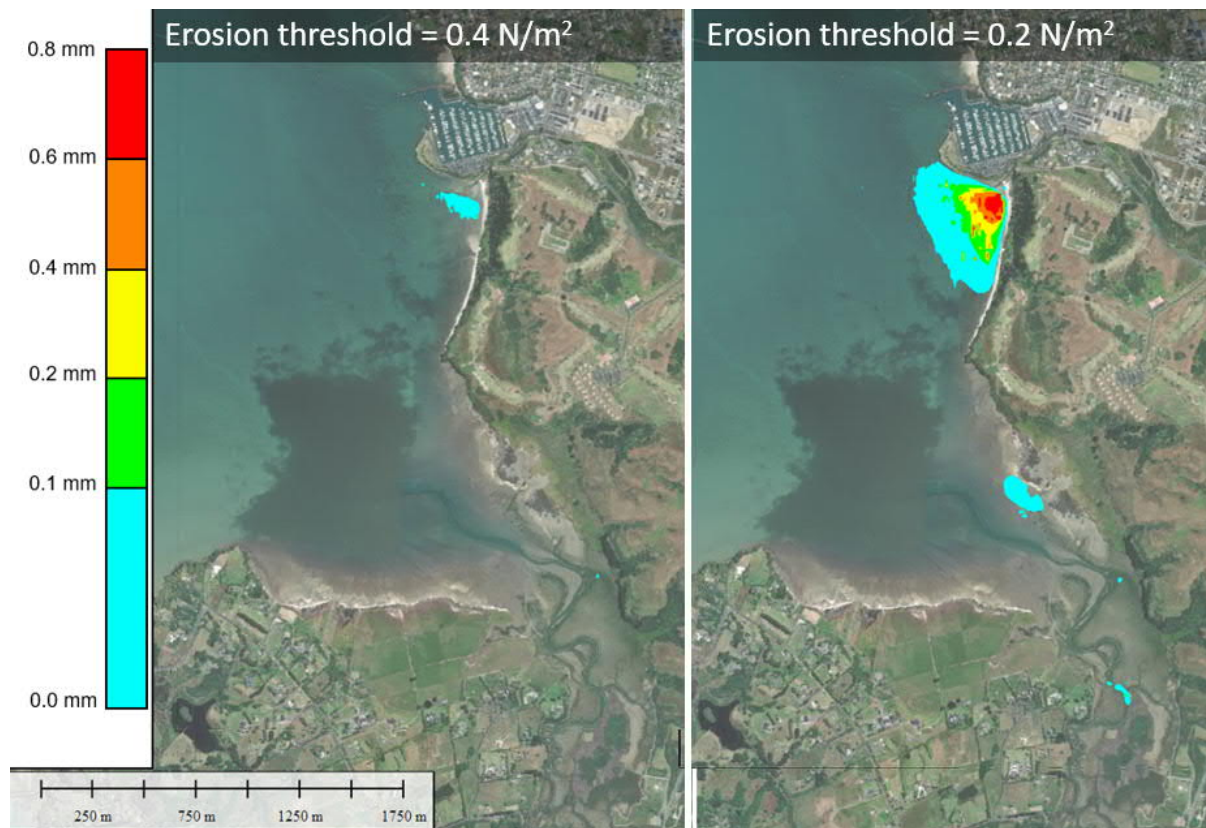
Figure 3-10 Re-erosion rates over a single high tide for a NW event, following a spring high tide deposition, in relation to 0.4 N/m 2 and 0.2 N/m 2 erosion thresholds in image left and image right respectively
