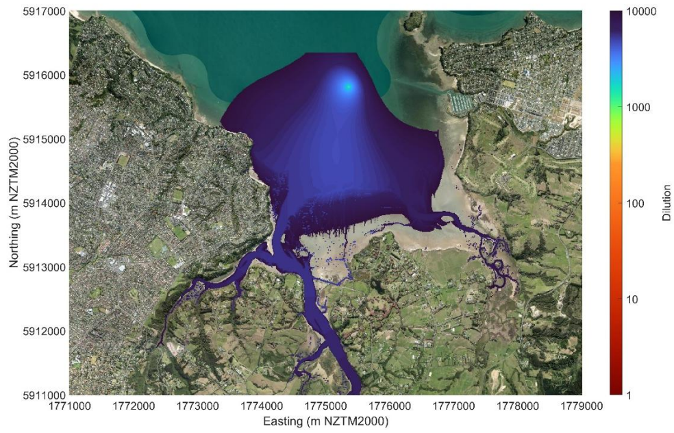
Figure Appendix C.5: Horizontal dispersion coefficient of 10 \text{ m}^2/\text{s} .
