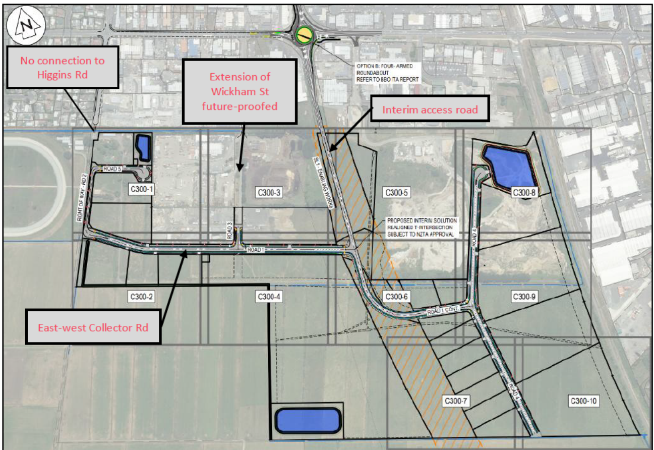
Figure 15: Interim Option B - Four-arm Roundabout and Interim Access Road
