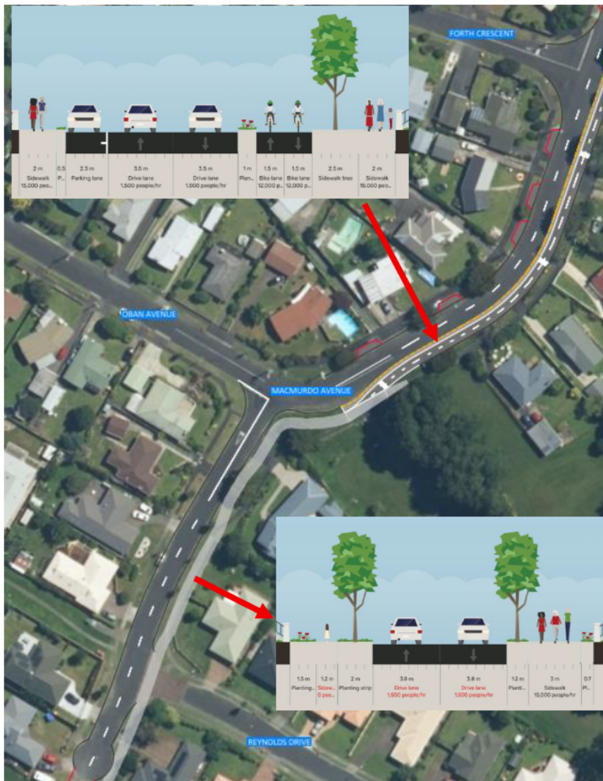
Figure 30: Indicative Alignment and Cross-section of MacMurdo Ave
