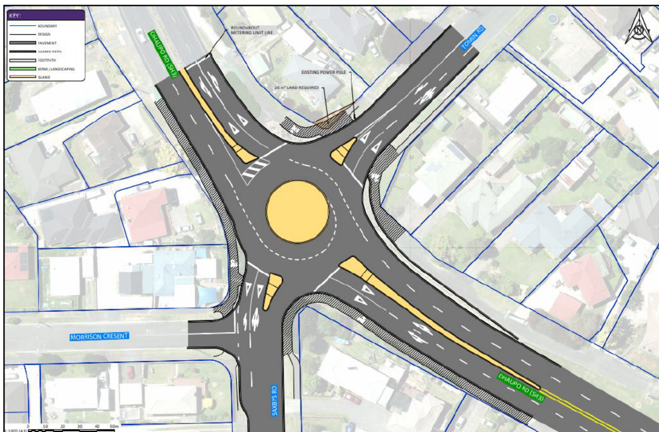
Figure 54: Ohaupo Rd / Saxbys Rd / Tomin Rd Alternative Roundabout Layout with Four Lanes on Ohaupo Rd (South), Additional Lanes on Saxbys Rd and Tomin Rd and Metering on Northern Approach
